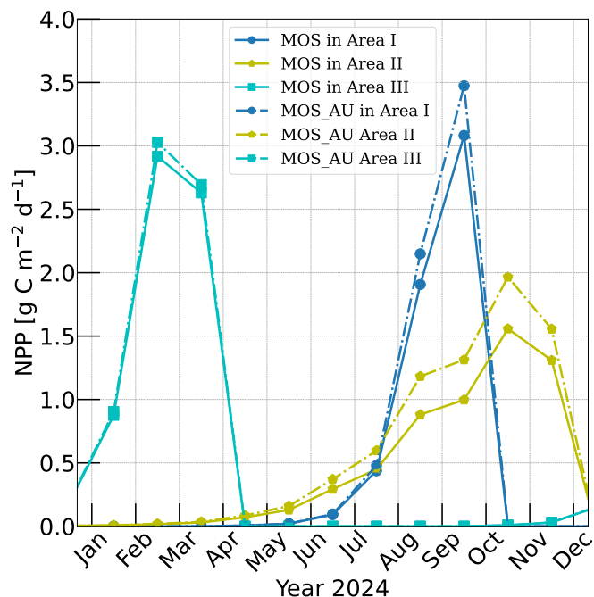
Figure 3. Vertically integrated \text{MOS}_{\text{macroalgae}} NPP rates simulated by experiment MOS (solid lines) for year 2024 and representative Areas I (dark blue circle), II (yellow pentagon) and III (cyan rectangle) highlighted by rectangles with corresponding colours in Fig.2. The NPP of MOS (solid) from the selected area I, II and III are reasonable compared to reported macroalgae NPP, and of experiment MOS_AU (dashed) shows an enhancement of NPP as expected.
