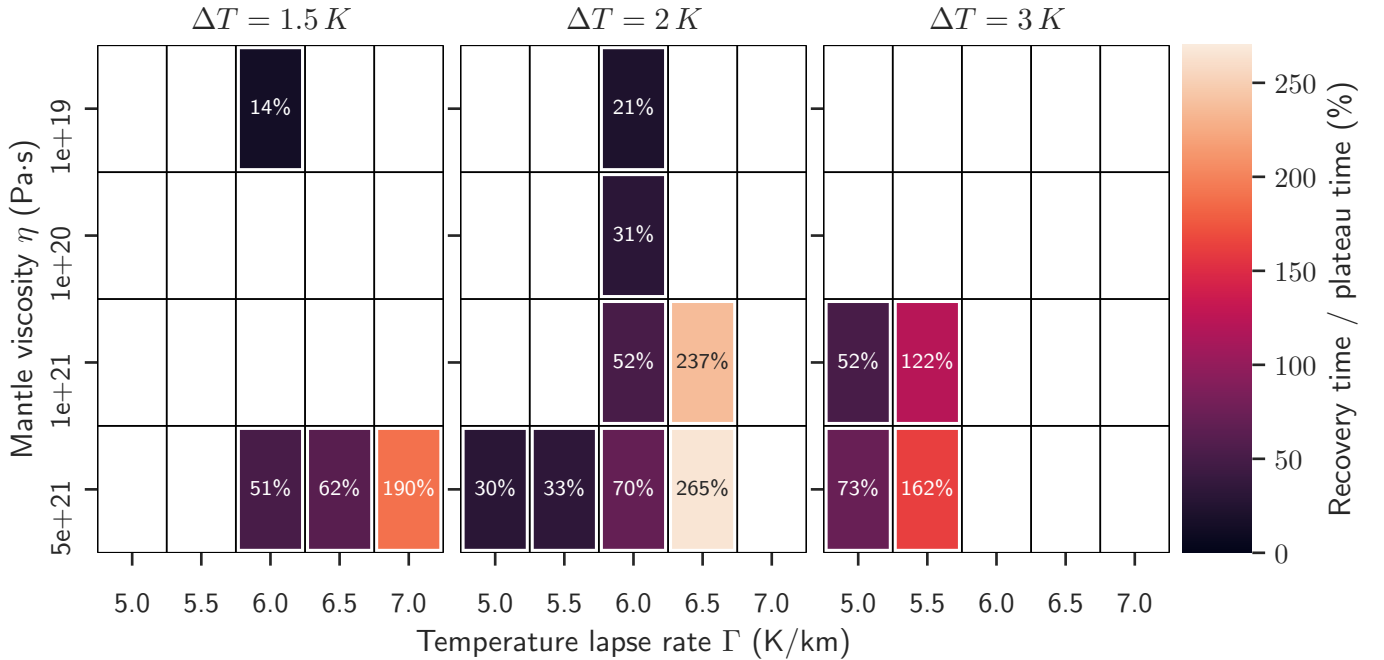
Figure 5. Ratio of recovery time vs. plateau time for three different warming temperatures, \Delta T = 1.5 K, 2 K, and 3 K. Measure for how long the lower half of the oscillation is compared to the upper half. A ratio of 100% would signify a perfectly symmetric oscillation, the lower the number, the more time is spent in a recovered regime (ice volume > average of minimal and maximal oscillation volume), and the higher the number the more time is spent at low ice volumes (ice volume < average of minimal and maximal oscillation volume).
