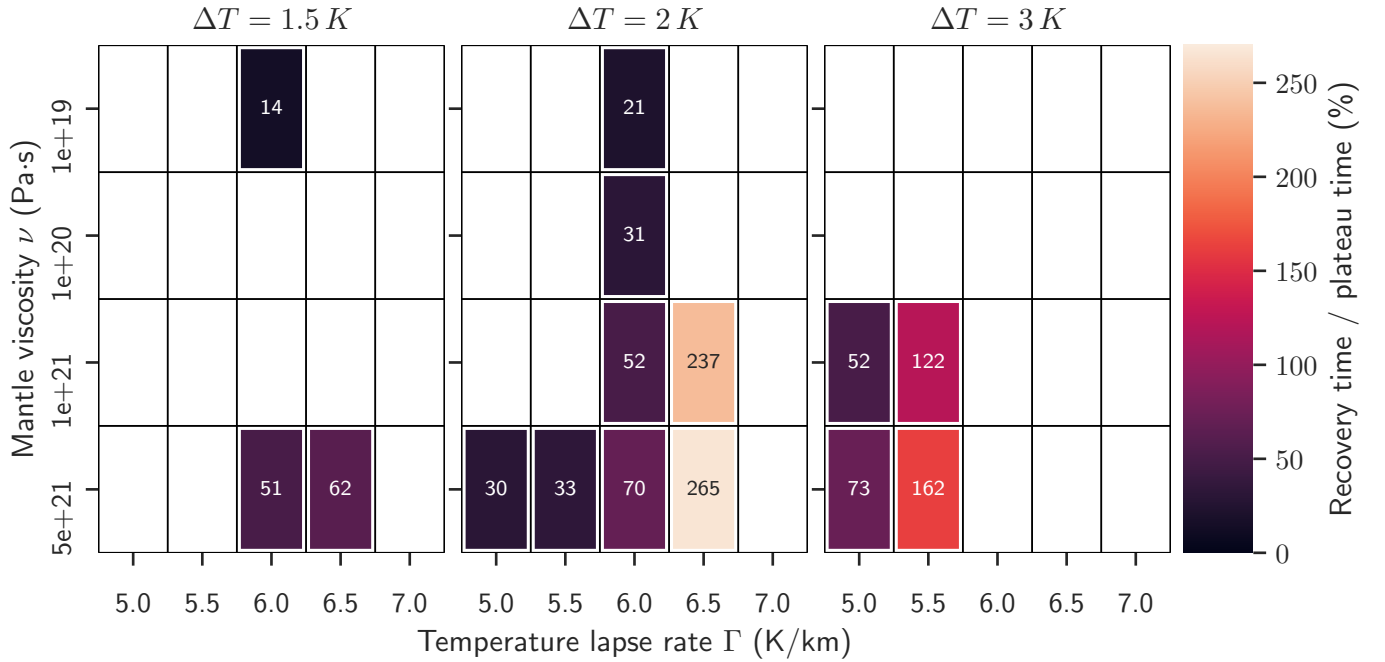
Figure 5. Ratio of recovery time vs. plateau time for three different warming temperatures, \Delta T = 1.5 \text{ K} , 2 \text{ K} , and 3 \text{ K} . Measure for how long the lower half of the oscillation is compared to the upper half. A ratio of 1 would signify a perfectly symmetric oscillation, the lower the number, the more time is spent in a recovered regime (ice volume > average of minimal and maximal oscillation volume), and the higher the number the more time is spent at low ice volumes (ice volume < average of minimal and maximal oscillation volume).
