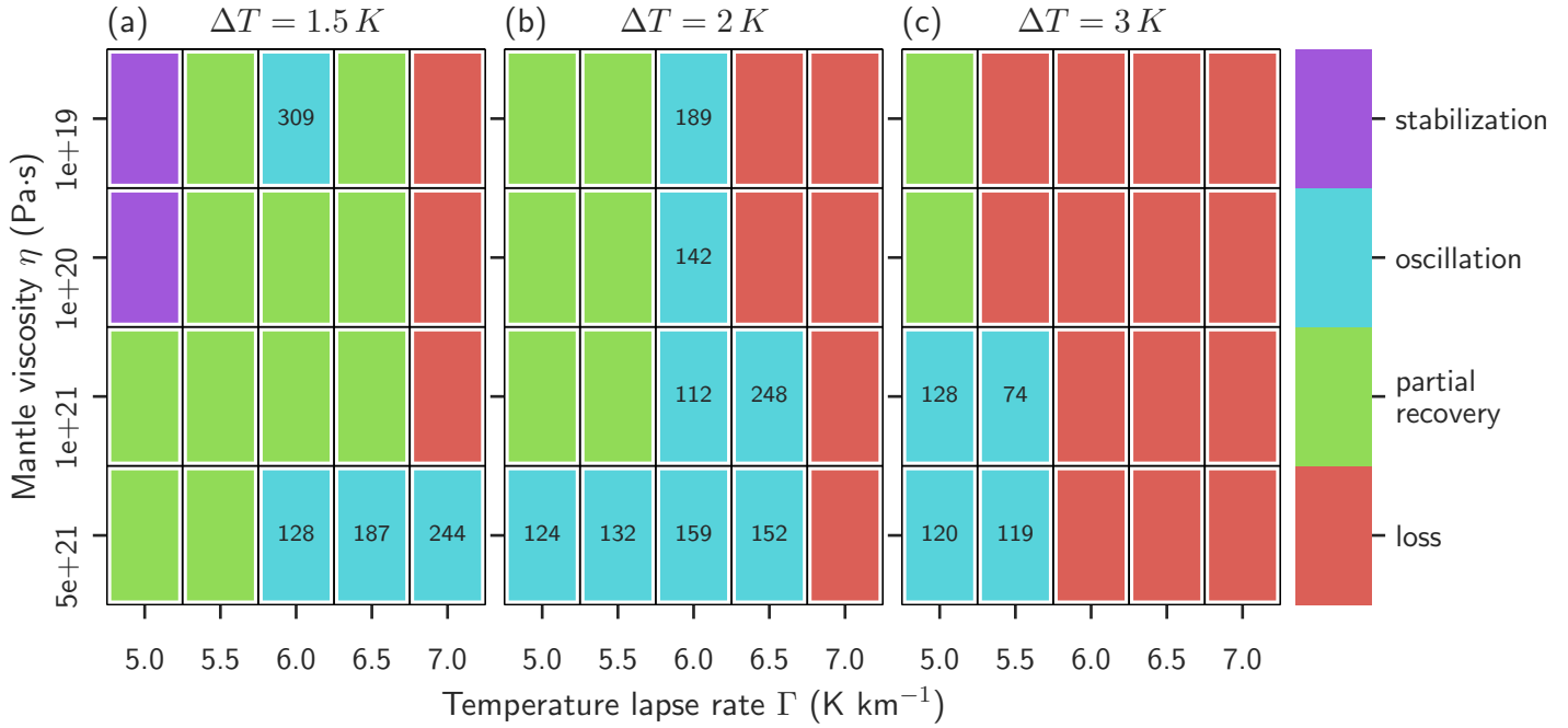
Figure 4. Dynamical regimes of Greenland ice sheet evolution for three different warming temperatures, \Delta T = 1.5 K, 2 K, and 3 K. The evolution regime of the Greenland Ice Sheet volume is indicated by the color code. Purple indicates immediate stabilization to a stable state, which preserves more than 90 % of the initial ice sheet volume, without passing a minimum. Green indicates, that the ice sheet volume recovers permanently after passing a minimum first. Blue indicates, that the ice sheet volume does not recover permanently, but shows self-sustained oscillations on a long time scale instead. Red indicates a permanent loss of ice sheet volume. The numbers in the cyan tiles show the approximate oscillation times.
