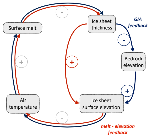
Figure 1. Interacting feedback loops for the proposed glacial isostatic adjustment feedback (GIA feedback). The orange-red part indicates the melt-elevation feedback: Higher air temperatures lead to decreasing climatic mass balance. This in turn leads to a decreasing ice thickness and in consequence to a decreasing ice surface elevation. If the surface elevation decreases, the air temperature rises due to the atmospheric lapse rate. This further decreases the climatic mass balance and leads to a positive (enhancing) feedback cycle. The timescale of this feedback cycle is driven by changes in the climate and is typically comparably fast. The blue part shows the counteracting mechanism of the ice load-bedrock uplift feedback. The decreasing ice thickness reduces the load on the bedrock, which leads to isostatic adjustment and therefore an uplift of the bedrock elevation. This mechanism partly counteracts the decrease in ice surface elevation and thus mitigates further increase in temperature. The timescale of this feedback loop depends on the rate of ice retreat and on the viscosity of the upper Earth mantle.
