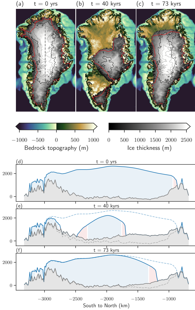
Figure 3. Spatial distribution of ice thickness at a temperature anomaly of \Delta T = 2\text{K} for the parameters \nu = 1 \times 10^{21} s, \Gamma = 6\text{K/km} . Maps and cross-sections of the bedrock topography and ice thickness show the initial state at the start of the simulation (A,D), the state with minimal volume after 40 kyrs (B,E) and the recovered state after 73 kyrs (C,F). The red outline and the red shaded areas indicate the ablation regions. The dashed lines in (E) and (F) show the initial topography of the ice sheet.
