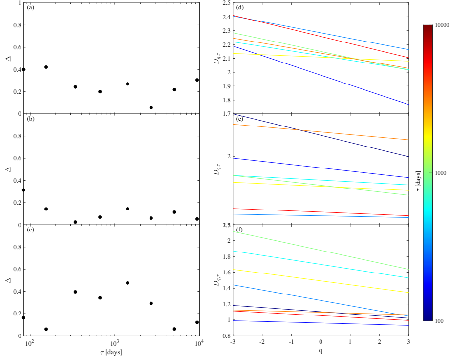
Figure 13. (a)-(c) Multifractal width \Delta and (d)-(f) D_{q,\tau} spectra at different timescales \tau_j for reconstructions of MIMFs as in Eq. (12) ( D_{q,\tau} ) for (a,d) the North Atlantic, (b,e) the North Pacific, and (c,f) the Tropical Pacific, respectively.
