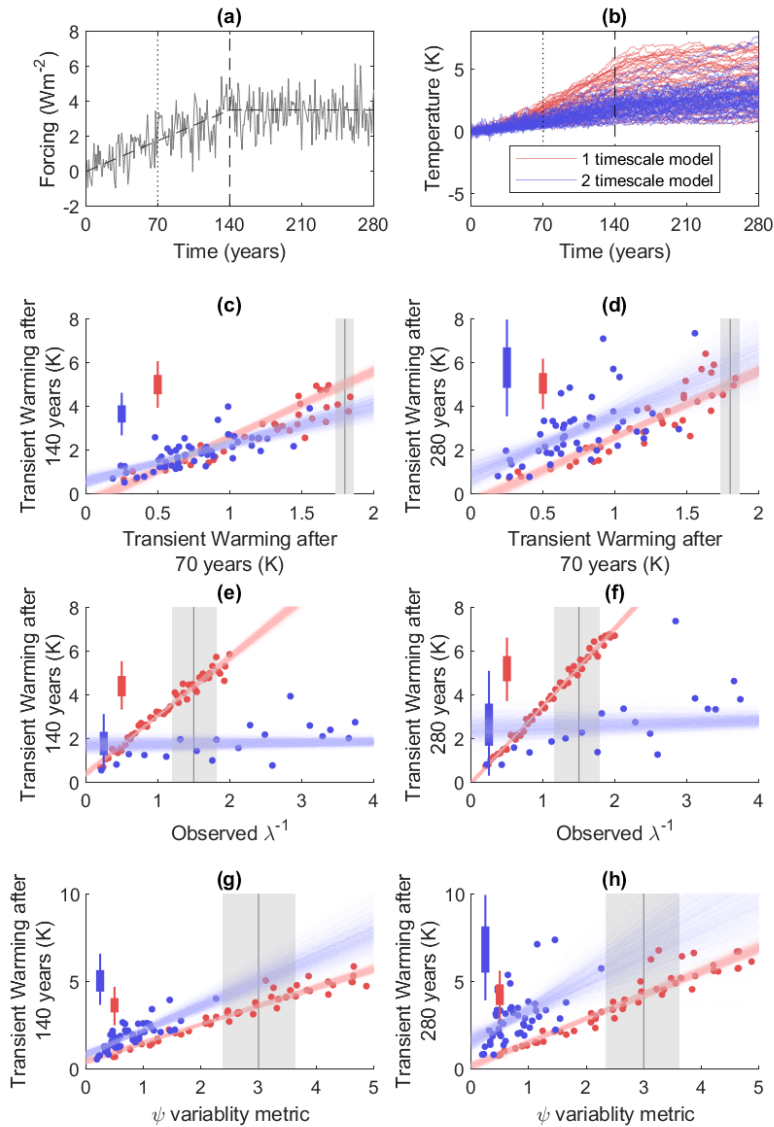
Figure 1. An illustration of the three kinds of emergent constraint in two structurally-different ensembles. (a) an idealised forcing timeseries used for each of the simulations - a (noisy) linear ramping of radiative forcing from years 0-140 followed by (noisy) constant forcing from years 140-280. (b) shows the response in 50-member perturbed parameter ensembles of two energy balance models, with one (red) and two (blue) timescales of response. (c) a constraint of the first kind, showing TCR (warming after 70 years of 1 percent annual increase in CO 2 concentrations) as a predictor of T140 (warming at time of CO 2 quadrupling, 140 years in the same experiment). (d) warming after a further 140 years of constant (quadrupled) CO 2 concentrations. (e,f) constraints of the second kind, using the feedback parameter 'lambda' to predict warming after (140, 280) years. (g,h) constraints of the third kind, using a variability metric (Cox et al., 2018b) derived from detrended temperature timeseries in years 1-70 as a predictor warming after (140, 280) years. In each case, colored points show members of the model ensemble, lines show bootstrap regression estimates, grey vertical bars show the 10th, 50th and 90th percentile of the (hypothetical) observed uncertainty distribution. Colored box/whisker plots show the 5/95th and 25/75th percentiles of the resulting constraint from each ensemble.
