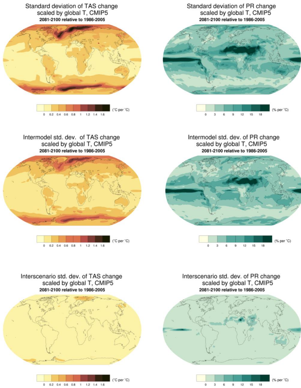
Figure A5: Top row: standard deviation of normalized patterns for individual CMIP5 models and scenarios. The individual patterns are the elements from which the averages shown in Fig. 3 are computed. Center row: Standard deviation of normalized patterns, after averaging across scenarios, highlighting the role of inter-model variability. Bottom row: Standard deviation of normalized patterns after averaging across models, highlighting the role of inter-scenario variability. These standard deviations can be compared with the corresponding results from CMIP6 models/scenarios in Fig. A5.
