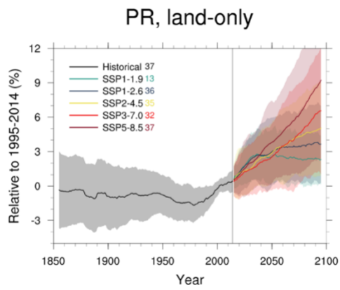
1000 Figure A2: Land-only and ocean-only average time series of temperature and percent precipitation changes relative to 1995-2014, for the 4 scenarios of Tier 1, SSP1-2.6, SSP2-4.5, SSP3-7.0, SSP5-8.5, and SSP1-1.9.
