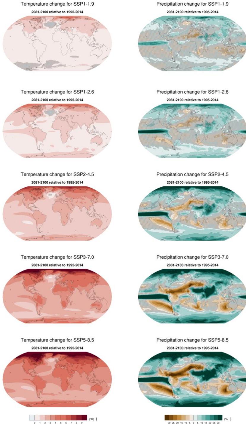
1015 Figure A4: Patterns of changes by 2081-2100 relative to 1995-2014 in surface air temperature (°C) and precipitation (%) under the five scenarios. Stitched areas are not significant, i.e., the magnitude of the change does not exceed the models' standard deviation.
