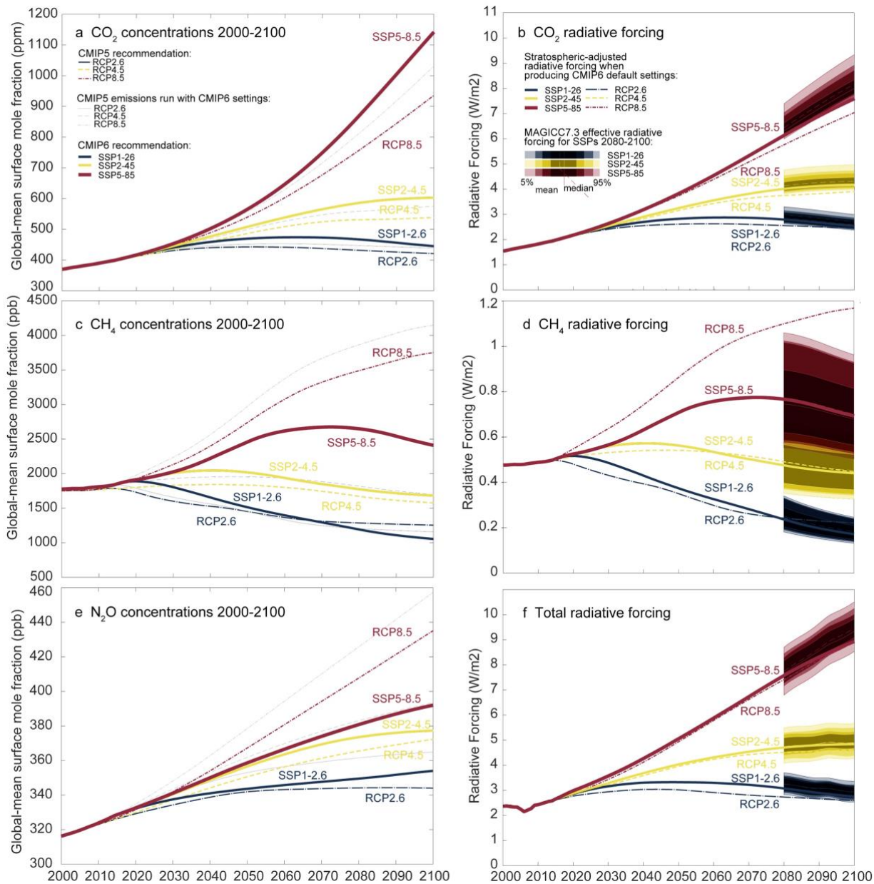
1035 Figure A7: Comparison of CO 2 , CH 4 and N 2 O concentrations and radiative forcings for the concentration-driven CMIP5 runs with RCP-Y scenarios (Meinshausen et al., 2011) and CMIP6 runs with SSPX-Y scenarios (Meinshausen et al., 2020). The higher scenario SSP5-8.5 features higher CO 2 concentrations largely due to updated carbon cycle settings. RCP8.5 emissions with the same carbon cycle settings (shown as thin dashed line in panel a) would produce similar CO 2 concentrations. The methane and nitrous oxide concentrations are however lower in SSP5-8.5 than in RCP8.5 (despite updated gas cycles producing higher concentrations for the same emission trajectory). Panels a, c and e adapted from Fig. 11 in Meinshausen et al. 2020. At the time of producing the SSPs (March 2018), stratospheric-adjusted radiative forcings have been used to compare the nameplate radiative forcing levels in 2100 using MAGICC6.8 with IPCC AR5 consistent settings (see panels b, d, f). Effective radiative forcings (ERFs) take additional adjustments into account that are non-temperature induced and differ from stratospheric-adjusted radiative 1040
