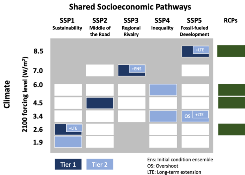
995 Figure A1: ScenarioMIP design (modified from O'Neill et al., 2020). White and colored boxes indicate achievable 2100 levels of forcings under the different SSPs. Grey areas are at the intersection of SSPs and radiative forcing levels that were not achievable by any of the IAMs employed to produce these scenarios.
