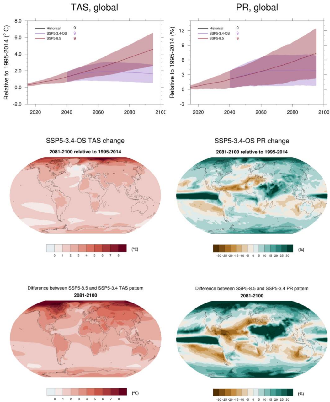
735 Figure 6: Time series and patterns comparing SSP5-8.5 to SSP5-3.4OS. First row: Global average time series of temperature and percent precipitation change (baseline: 1995-2014). Second row: Patterns of change for the same quantities, under the lower scenario, SSP5-3.4OS. Third row: Differences between the patterns of change under the higher (SSP5-8.5) and lower scenario.
