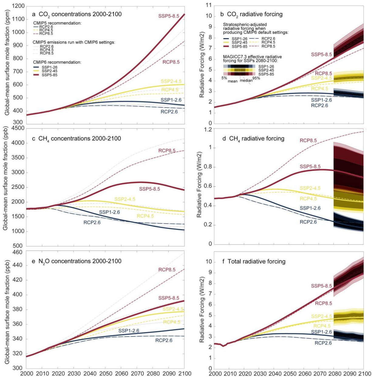
1490 Figure A7: Comparison of CO 2 , CH 4 and N 2 O concentrations and radiative forcings for the concentration-driven CMIP5 runs with RCP-Y scenarios (Meinshausen et al., 2011) and CMIP6 runs with SSPX-Y scenarios (Meinshausen et al., 2020). The higher 1495 scenario SSP5-8.5 features higher CO 2 concentrations largely due to updated carbon cycle settings. RCP8.5 emissions with the same carbon cycle settings (shown as thin dashed line in panel a) would produce similar CO 2 concentrations. The methane and nitrous oxide concentrations are however lower in SSP5-8.5 than in RCP8.5 (despite updated gas cycles producing higher concentrations for the same emission trajectory). Panels a, c and e adapted from Figure 11 in Meinshausen et al. 2020. At the time of producing the SSPs (March 2018), stratospheric-adjusted radiative forcings have been used to compare the nameplate radiative forcing levels in 2100 using MAGICC6.8 with IPCC AR5 consistent settings (see panels b, d, f). Effective radiative forcings (ERFs) take additional adjustments into account that are non-temperature induced and differ from stratospheric-adjusted radiative
