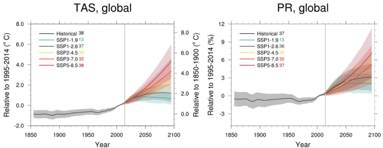
310 Figure 1: Left panel: global average temperature time series (21-yr running averages) of changes from current baseline (1995- 2014, left axis) and pre-industrial baseline (1850-1900, right axis, obtained by adding a 0.84°C offset) for SSP1-1.9, SSP1-2.6, SSP2-4.5, SSP3-7.0 and SSP5-8.5. Right panel: global average precipitation time series (21-yr running averages) of percent 315 changes from current baseline (1995-2014) for SSP1-1.9, SSP1-2.6, S SP2-4.5, SSP3-7.0 and SSP5-8.5. Thick lines are ensemble means (number of models shown in the legends). The shading represents the \pm 1.64\sigma interval, where \sigma is the standard deviation of the smoothed trajectories computed year-by-year (thus approximating the 5-95% confidence interval around the mean of a normal distribution). Note that the uncertainty bands are computed for the anomalies with respect to the historical baseline (1995- 2014). Thus, the right axis of the global temperature plot, showing anomalies with respect to pre-industrial, applies to the ensemble means, not to the uncertainty bands, which would be narrowest over the period 1850-1900 if we were to calculate uncertainties on
