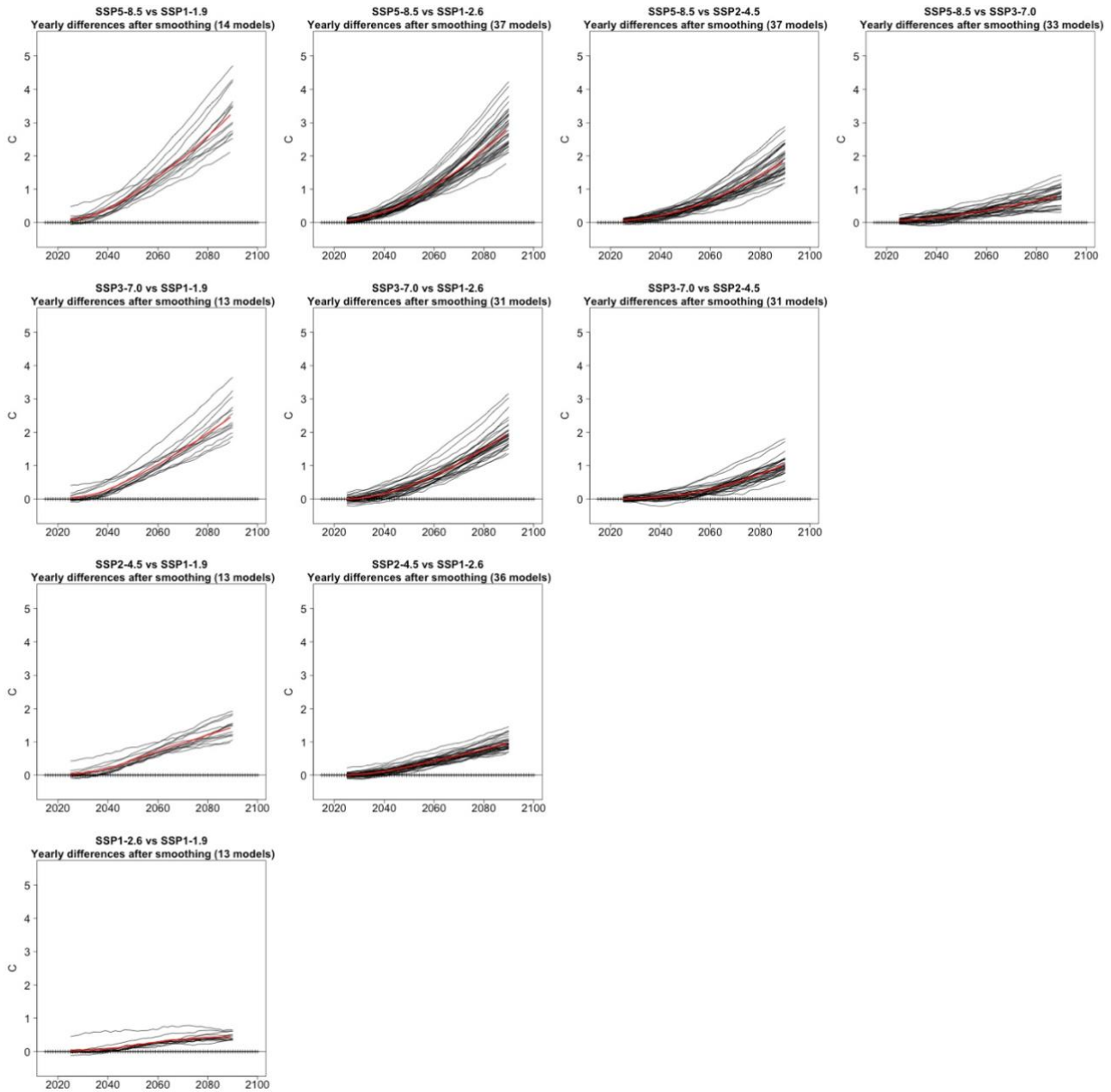
1460 Figure A3: Time series of year-by-year differences in GSAT between each scenario run in Tier 1 and each of the lower scenario runs (including SSP1-1.9). The time series from the individual models were first smoothed by a 21-year running mean. First row: differences between SSP5-8.5 and, respectively, SSP1-1.9, SSP1-2.6, SSP2-4.5 and SSP3-7.0. Second row: differences between SSP3-7.0 and respectively SSP1-1.9, SSP1-2.6 and SSP2-4.5. Third row: differences between SSP2-4.5 and SSP1-1.9 and SSP1-2.6. Fourth row: differences between SSP1-2.6 and SSP1-1.9. Each black line corresponds to an 1465 individual model's time series of differences. The red line is the ensemble mean difference. The ensemble size varies across the plots based on the number of models available for which the difference can be computed. It is as small as 10 members for those
