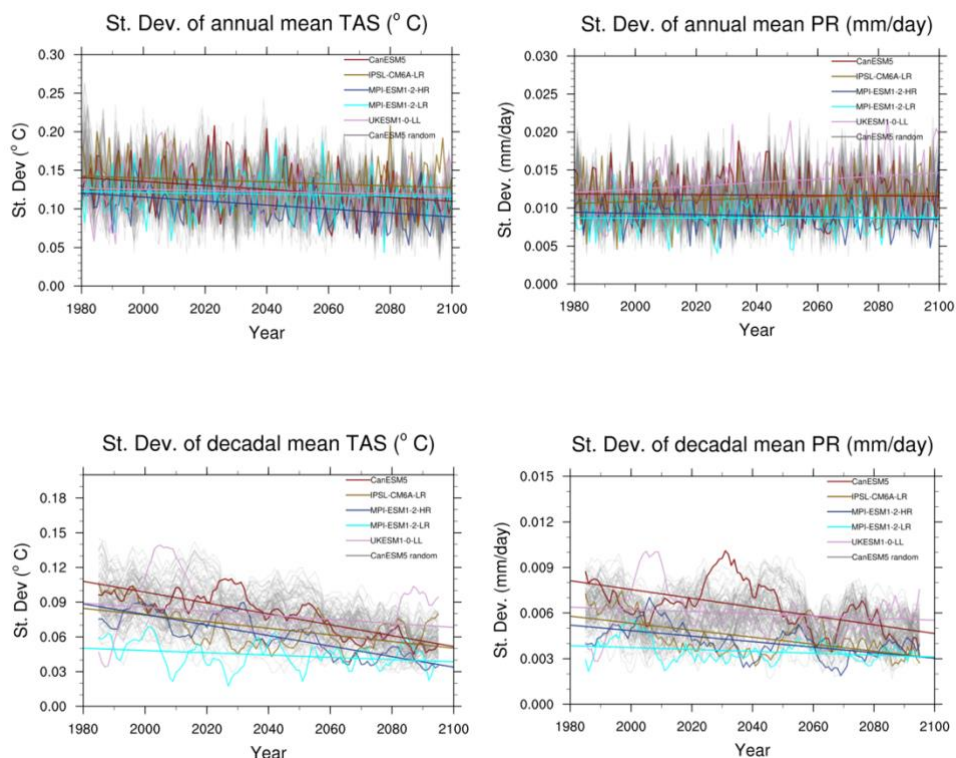
655 Figure 5: Time series of ensemble spreads (i.e., inter-member standard deviations) computed at each year among annual (top row) or decadal (bottom row) mean values of TAS (left) and PR (right). The grey lines are obtained by resampling subset of ten members from the CanESM5 model ensemble that provides 50 members. They are meant to provide a qualitative indication of the variability “hidden” in the 10 member ensembles provided by the majority of the models. The color lines show the time series of standard deviations computed from 10 members of 5 models running SSP3-7.0: CanESM5 (first ten members, red), IPSL-CM6A-LR (yellow), MPI-ESM1-2-HR (blue), MPI-ESM1-2-LR (cyan) and UKESM1 (light purple). Straight lines show least square fits of the linear trends.
