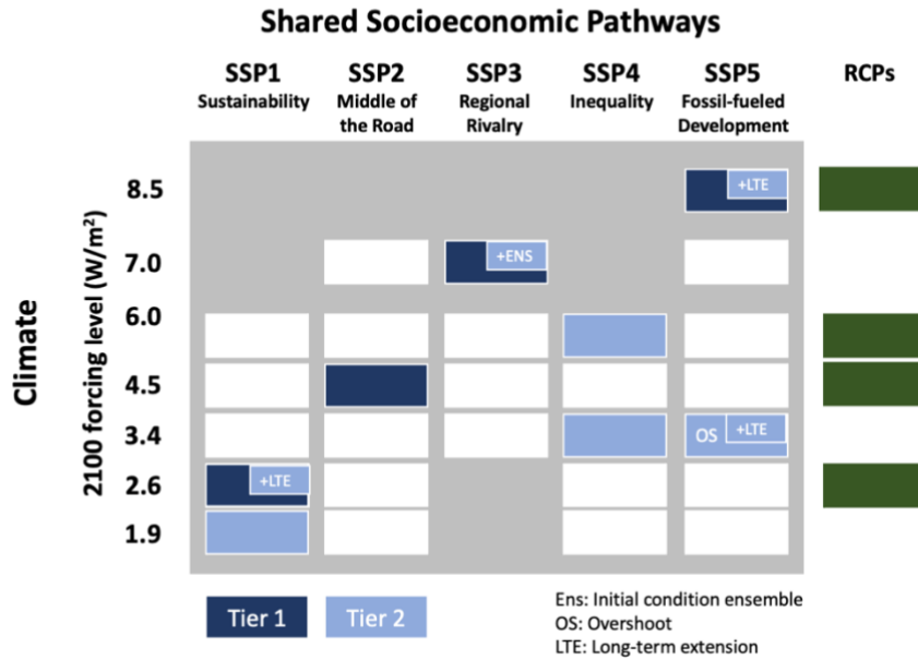
1450 Figure A1: ScenarioMIP design (modified from O'Neill et al., 2020). White and colored boxes indicate achievable 2100 levels of forcings under the different SSPs. Grey areas are at the intersection of SSPs and radiative forcing levels that were not achievable by any of the IAMs employed to produce these scenarios.
