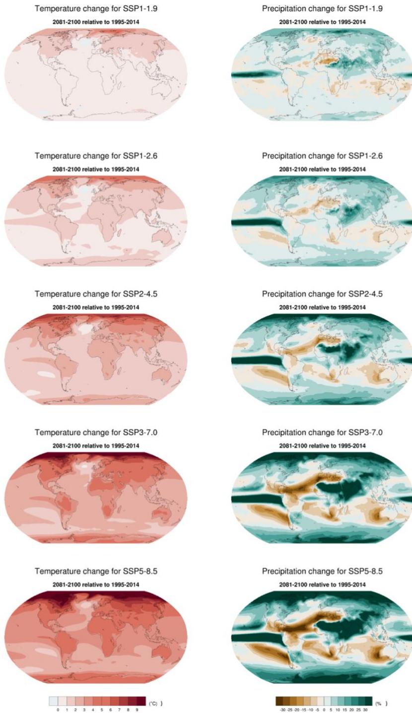
1470 Figure A4: Patterns of changes by 2081-2100 relative to 1995-2014 in surface air temperature (°C) and precipitation (%) under the five scenarios.
