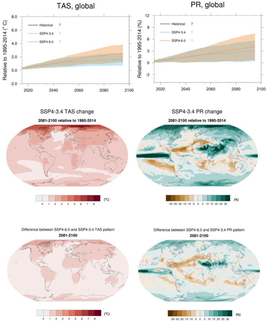
740 Figure 7: Like Figure 6, but for SSP4-6.0 and SSP4-3.4.
