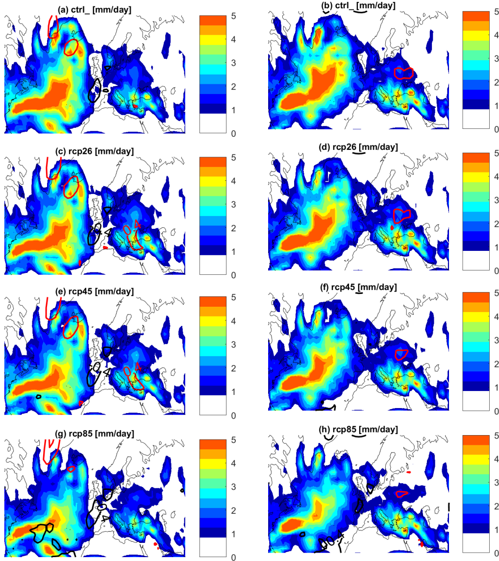
Figure 10. Daily precipitation rates in PlaSIM simulations: Average of the daily precipitation rates [mm/day] for Cluster 1 (a,c,e,g), Cluster 2 (b,d,f,h) of analogues. (a,b) control run, (c,d) RCP2.6 run, (e,f) RCP4.5 run, (g,h) RCP8.5 run. Isolines represent positive (in red) and negative (in black) standardized anomalies.
