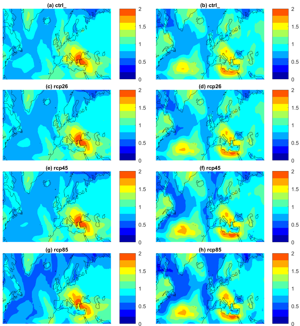
Figure B4. Two meters Temperature uncertainty in PlaSIM analogues: Root mean squared difference in standardized two meters Temperature [standard deviations] between analogues and cluster centroids for Cluster 1 (a,c,e,g), Cluster 2 (b,d,f,h). (a,b) control run, (c,d) RCP2.6 run, (e,f) RCP4.5 run, (g,h) RCP8.5 run
