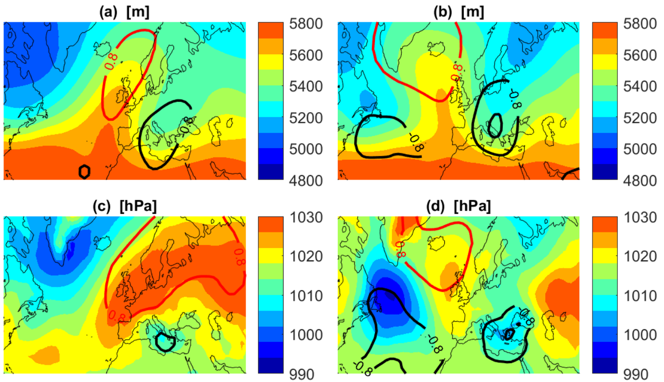
Figure 2. Dynamics for clusters of cold spells over Italy 500 hPa Geopotential height [m] (a,b) and sea-level pressure [hPa] (c,d) averaged over the two clusters of cold spells in Italy found via k -means. Cluster 1 (a,c) is characterized by a zonally tilted high pressure located between the British Islands and Russia, cluster 2 (b,d) by an omega-blocking pattern between the Atlantic and Europe. Black and red isolines represent negative and positive standardized anomalies.
