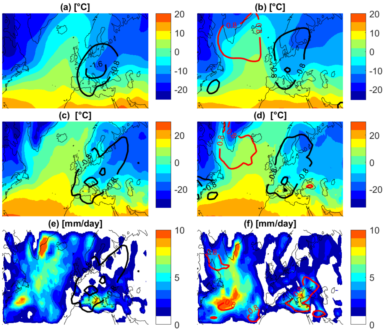
Figure 3. Physics for clusters of cold spells over Italy Temperature at 850 hPa [°C] (a,b), two meters temperatures [°C] (c,d), precipitation rate [mm/day] (e,f) averaged over the two clusters of cold spells in Italy found via k -means. In cluster 1 (a,c,e) warm air is advected towards the British Islands and cold air flows mainly from Russia and Eastern Europe. In cluster 2 (b,d,f) warm air extends North from the Azores to Iceland and cold air flows South from Scandinavia. The temperature field at the surface is very similar, with cold temperatures over continental areas, and negative or very low positive daily values over Italy, especially the peninsular regions. Black and red isolines represent negative and positive standardized anomalies.
