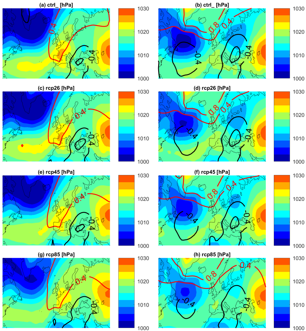
Figure 7. Sea level pressure in PlaSIM simulations: Average of the sea-level pressure [hPa] for Cluster 1 (a,c,e,g), Cluster 2 (b,d,f,h) of analogues. (a,b) control run, (c,d) RCP2.6 run, (e,f) RCP4.5 run, (g,h) RCP8.5 run. Isolines represent positive (in red) and negative (in black) standardized anomalies.
