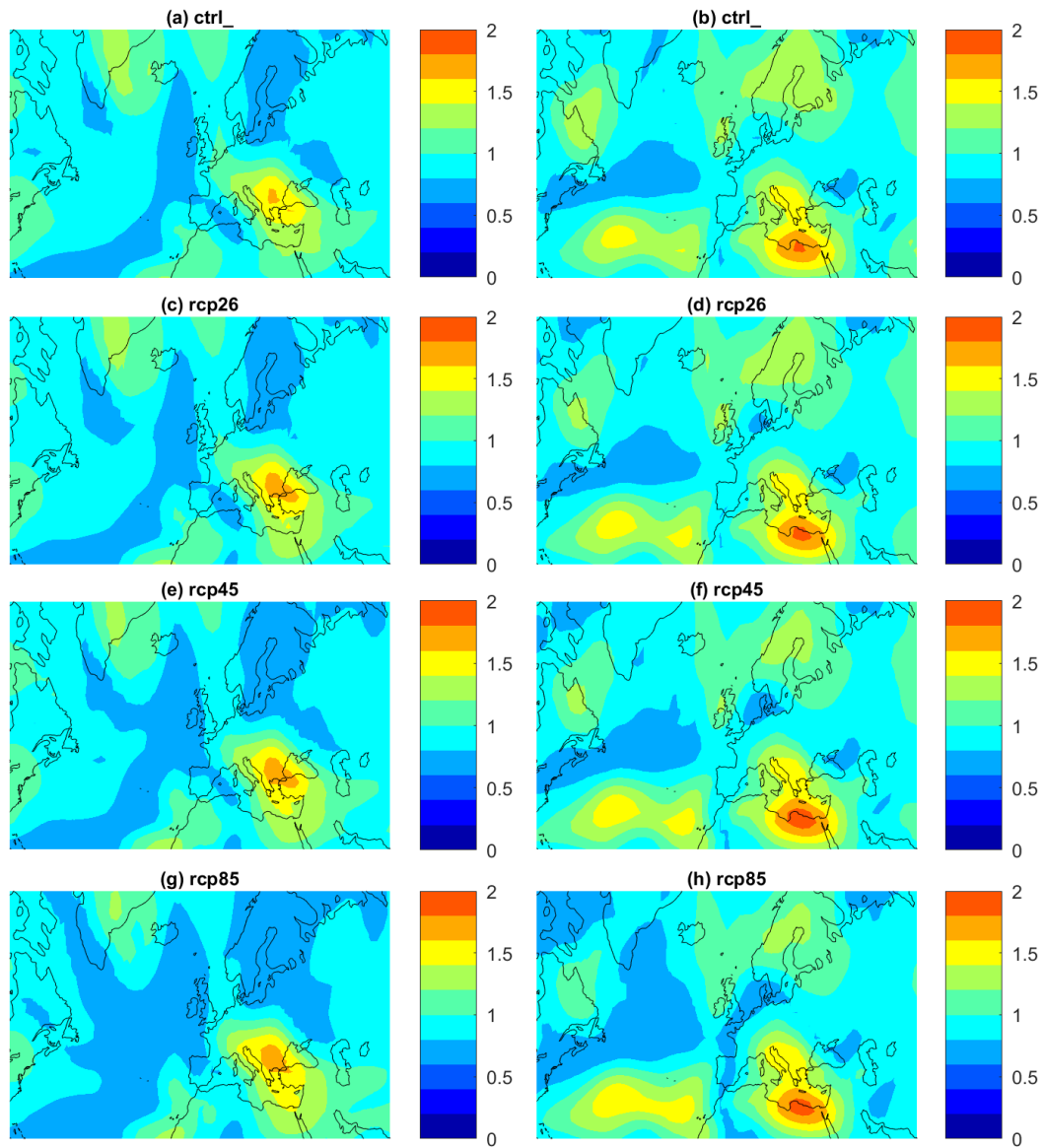
Figure B3. 850 hPa Temperature uncertainty in PlaSIM analogues: Root mean squared difference in standardized 850 hPa Temperature [standard deviations] between analogues and cluster centroids for Cluster 1 (a,c,e,g), Cluster 2 (b,d,f,h). (a,b) control run, (c,d) RCP2.6 run, (e,f) RCP4.5 run, (g,h) RCP8.5 run
