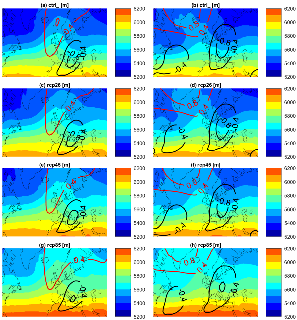
Figure 6. 500 hPa Geopotential heights in PlaSIM simulations: Average of the 500 hPa geopotential height [m] for Cluster 1 (a,c,e,g), Cluster 2 (b,d,f,h) of analogues. (a,b) control run, (c,d) RCP2.6 run, (e,f) RCP4.5 run, (g,h) RCP8.5 run. Isolines represent positive (in red) and negative (in black) standardized anomalies.
