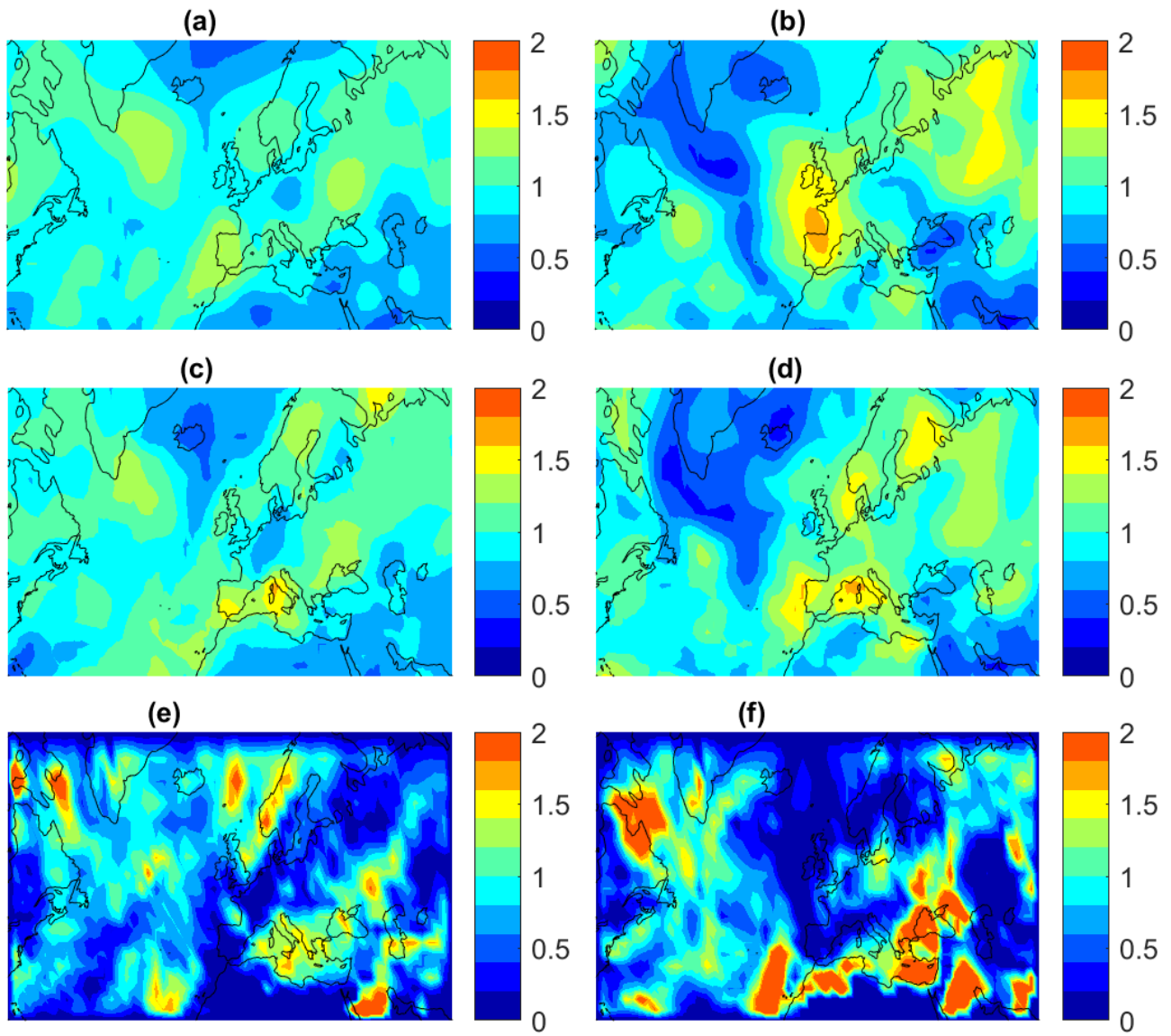
Figure 5. Cluster uncertainty Standard deviation of Temperature at 850 hPa [°C] (a,b), two meters temperatures [°C] (c,d), precipitation rate [mm/day] (e,f) of the two clusters of cold spells in Italy found via k-means.
