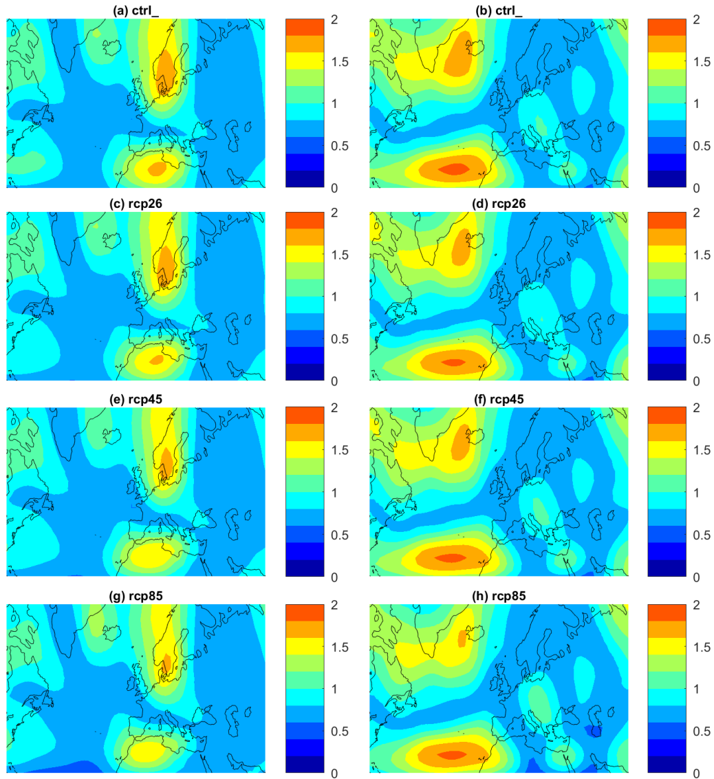
Figure B1. 500 hPa Geopotential height uncertainty in PlaSIM analogues: Root mean squared difference in standardized 500 hPa geopotential height [standard deviations] between analogues and cluster centroids for Cluster 1 (a,c,e,g), Cluster 2 (b,d,f,h). (a,b) control run, (c,d) RCP2.6 run, (e,f) RCP4.5 run, (g,h) RCP8.5 run
