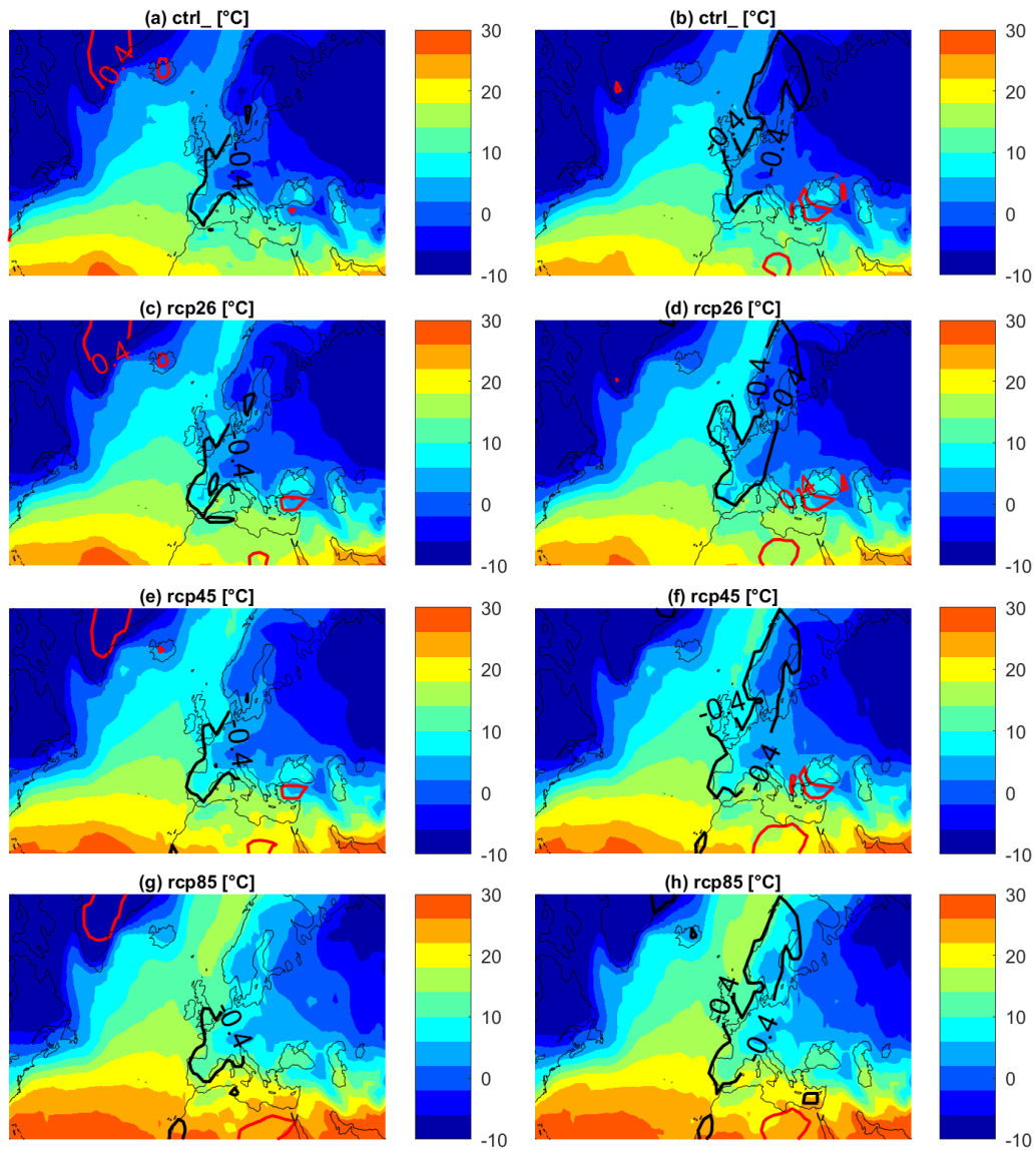
Figure 9. Two meters temperatures in PlaSIM simulations: Average of the two meters temperature [°C] for Cluster 1 (a,c,e,g), Cluster 2 (b,d,f,h) of analogues. (a,b) control run, (c,d) RCP2.6 run, (e,f) RCP4.5 run, (g,h) RCP8.5 run. Isolines represent positive (in red) and negative (in black) standardized anomalies.
