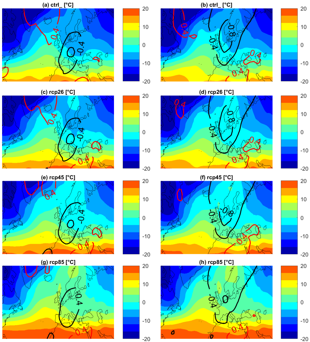
Figure 8. 850 hPa Temperature in PlaSIM simulations: Average of the 850 hPa temperature [ ^{\circ}\text{C} ] for Cluster 1 (a,c,e,g), Cluster 2 (b,d,f,h) of analogues. (a,b) control run, (c,d) RCP2.6 run, (e,f) RCP4.5 run, (g,h) RCP8.5 run. Isolines represent positive (in red) and negative (in black) standardized anomalies.
