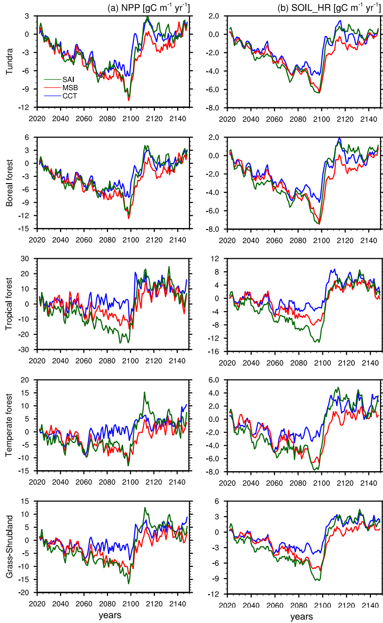
Figure 4. The relative difference between the RM to RCP8.5 scenario. The values are mean biome NPP and SOIL_HR in land areas across -60 to 70°N latitude.
