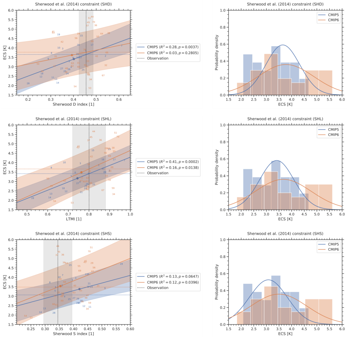
480 Figure 3: As Figure 2, but for the constraints SHD, SHL and SHS.
