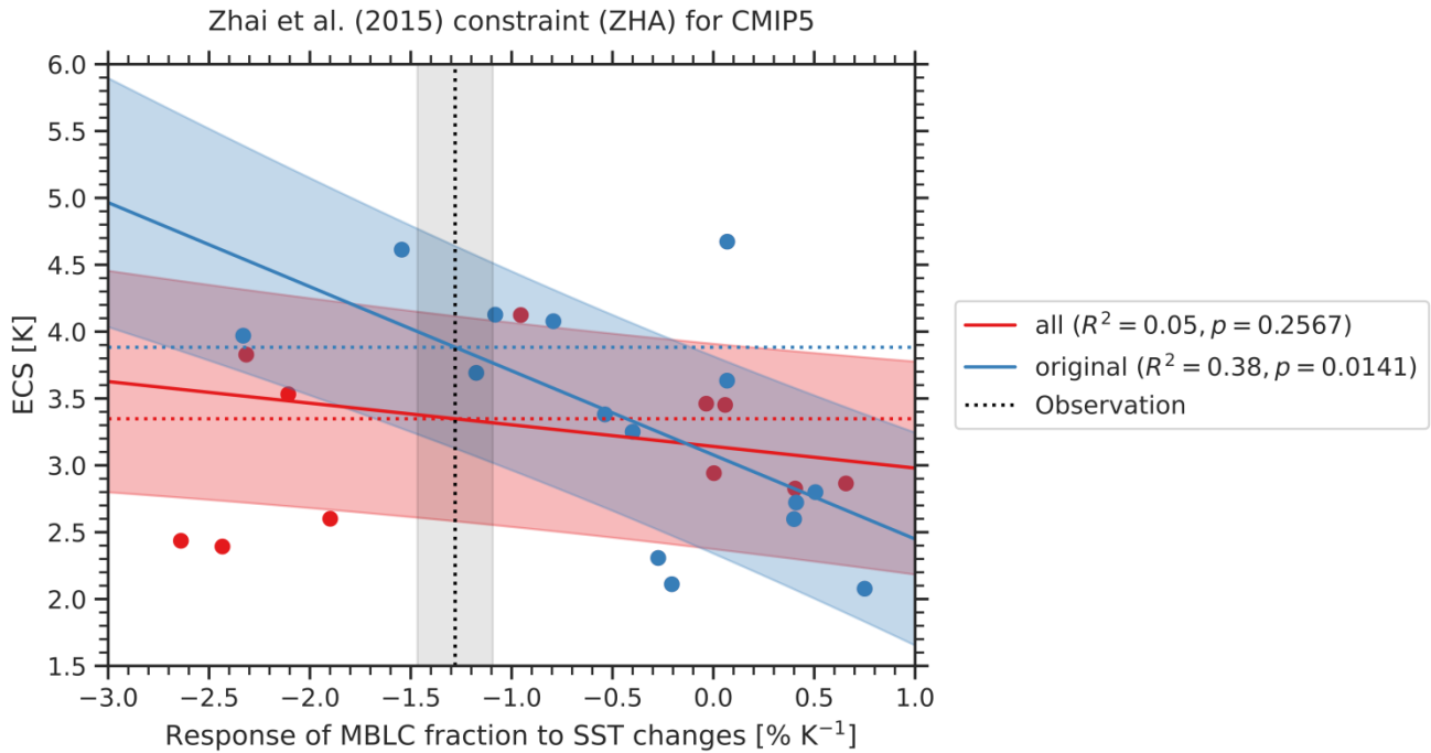
490 Figure 6: Emergent relationship ZHA (Zhai et al., 2015) for different subsets of CMIP5 models. Blue circles show the 15 CMIP5 models used in the original publication (except for CESM1-CAM5): the solid blue line and blue shaded area show the emergent relationships evaluated on these models including the uncertainty range. In our study, we added 11 more CMIP5 models (red circles). The corresponding emergent relationship that considers all available CMIP5 models is shown in red colors. This relationship shows a considerably lower coefficient of determination ( R^2 ) and higher p -value than the relationship using the original subset of CMIP5 models. The vertical dashed line and shaded area correspond to the observational reference and the horizontal dashed lines to the 495 corresponding ECS constraints using this observation.
