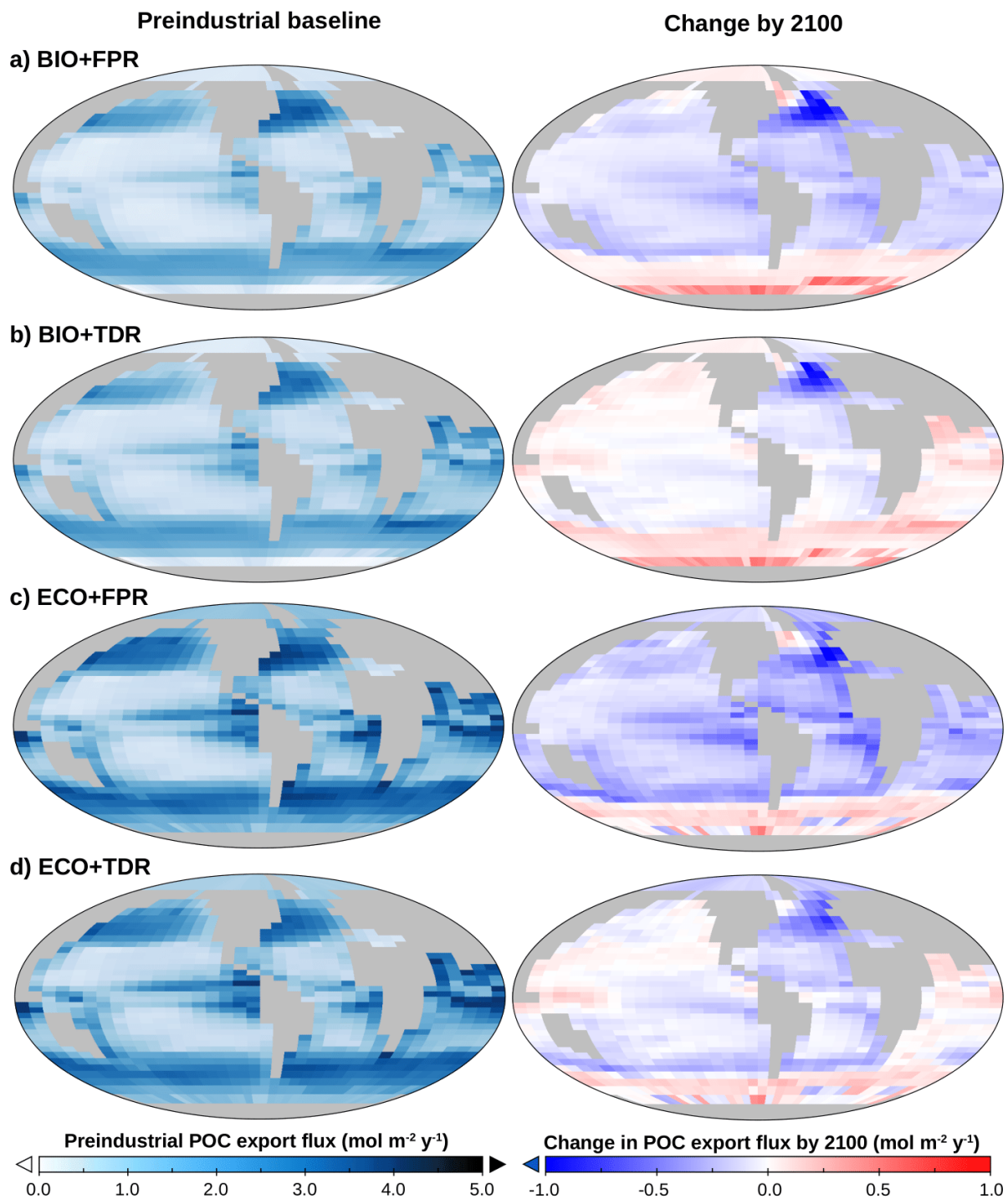
920 Figure 3: a) cGENIE/ecoGENIE POC export maps for default calibrations of BIO+FPR (a), BIO+TDR (b), ECO+FPR (c), and ECO+TDR (d), showing baseline export patterns (left) and the change in POC export by 2100 relative to the 1765 preindustrial baseline as a result of RCP4.5 (right). Plot created with Panoply, available from NASA Goddard Space Flight Center.
