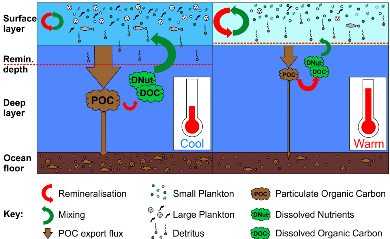
910 Figure 1: Schematic illustrating the impact of warming on the soft tissue biological pump. On the left-side, under cooler preindustrial conditions cGENIE's surface layer remains fairly well mixed with the deep ocean (green arrow), returning dissolved nutrients and carbon (DNut & DOC) from the remineralisation of exported POC (red arrow), while some POC is remineralised partly within the surface layer (surface red arrows). On the right-side, warming leads to a shift to dominance by smaller plankton as well as stratification leading to less mixing between the shallow and deep ocean, while shoaling of the remineralisation depth leads to greater recycling of nutrients and carbon close to the surface layer, combining to result in an overall reduction in POC export and sedimentation and an overall increase in the residence time of nutrients and carbon in the ocean.
