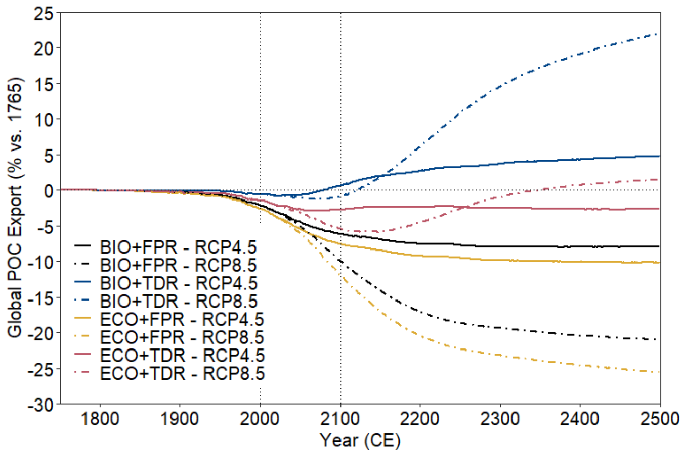
915 Figure 2: cGenIE/ecoGenIE simulation results for global POC export flux under different configurations and forcing scenarios. Results for RCP4.5 (solid lines) and RCP8.5 (dot-dashed lines) are shown for each of the configurations (BIO+FPR – black; BIO+TDR – blue; ECO+FPR – yellow; ECO+TDR – red), and the baseline POC export and the 21 st century marked by the horizontal and vertical dotted lines respectively. Results for all emission scenarios are shown in Supplementary Figure S48.
