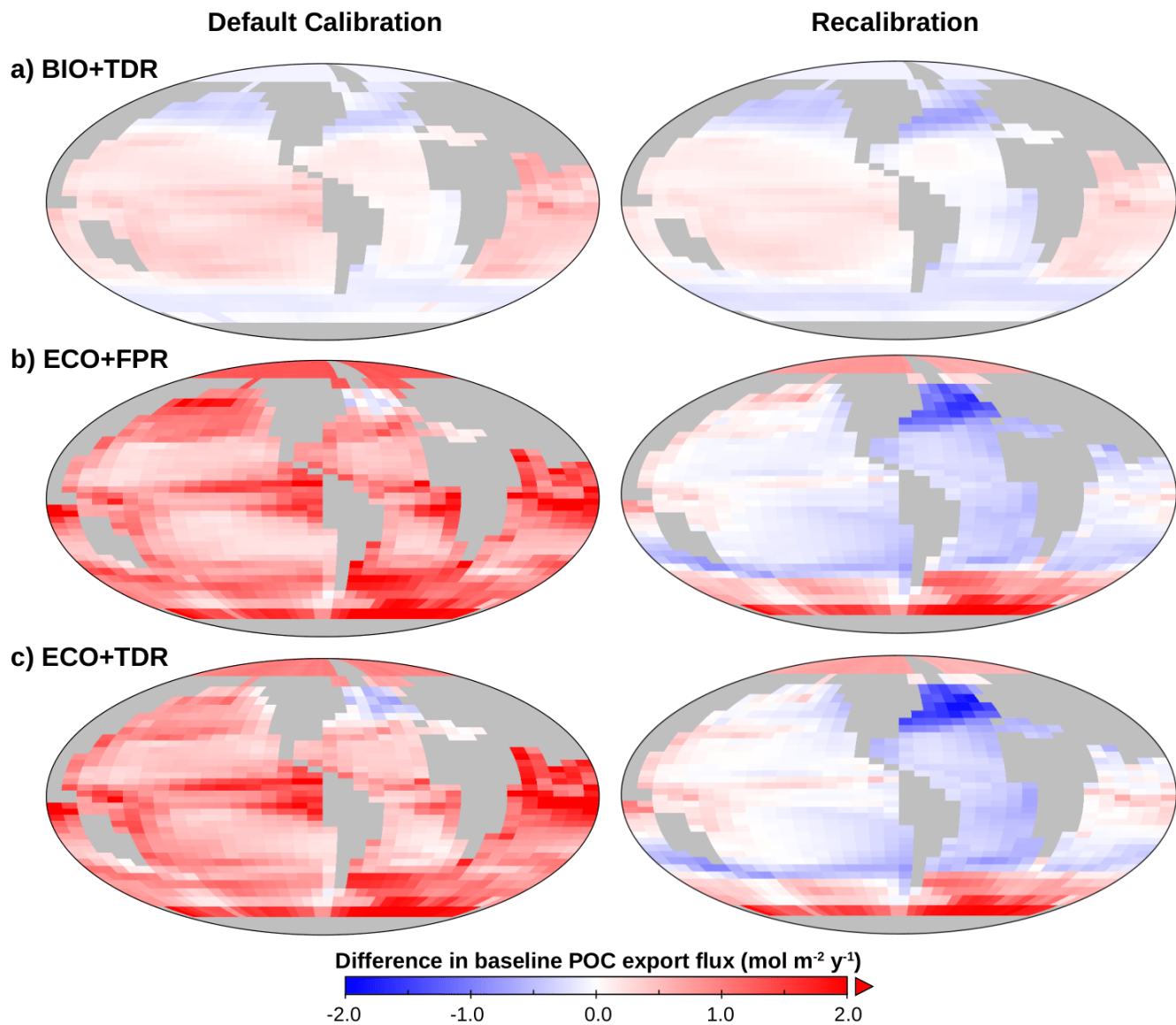
925 Figure 4: cGENIE/ecoGENIE POC export maps, showing changes in baseline for BIO+TDR (a), ECO+FPR (b), and ECO+TDR (c) in the default calibration (left) and recalibrations (right) relative to the default BIO+FPR configuration (Figure 3a, left). Plot created with Panoply, available from NASA Goddard Space Flight Center.
