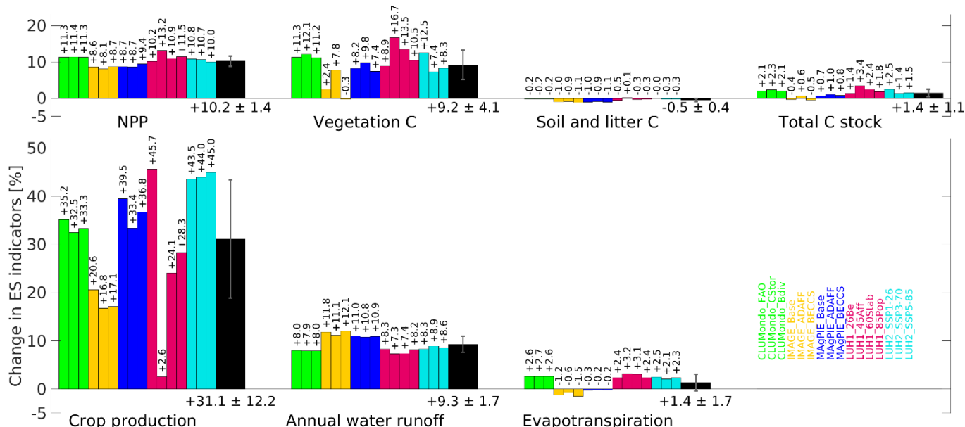
Fig. 3. Change and uncertainty in ES indicators from 2000-2004 to 2036-2040 in percent relative to the base level in 2000-2004 across 16 land-use scenarios. Black bars give average and standard deviation of the relative changes across all scenarios. See Table S3 for absolute levels and changes for each scenario.
