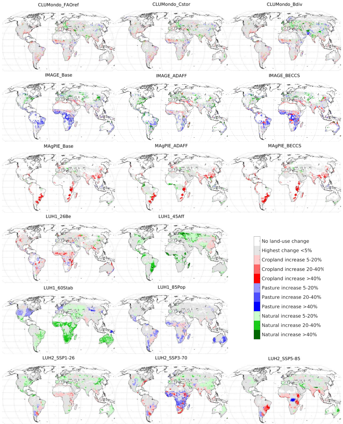
Fig. 2. Categories of dominant land-use change from 2000-2004 to 2036-2040 for each of 16 land-use scenarios. The legend is identical for all plots.
