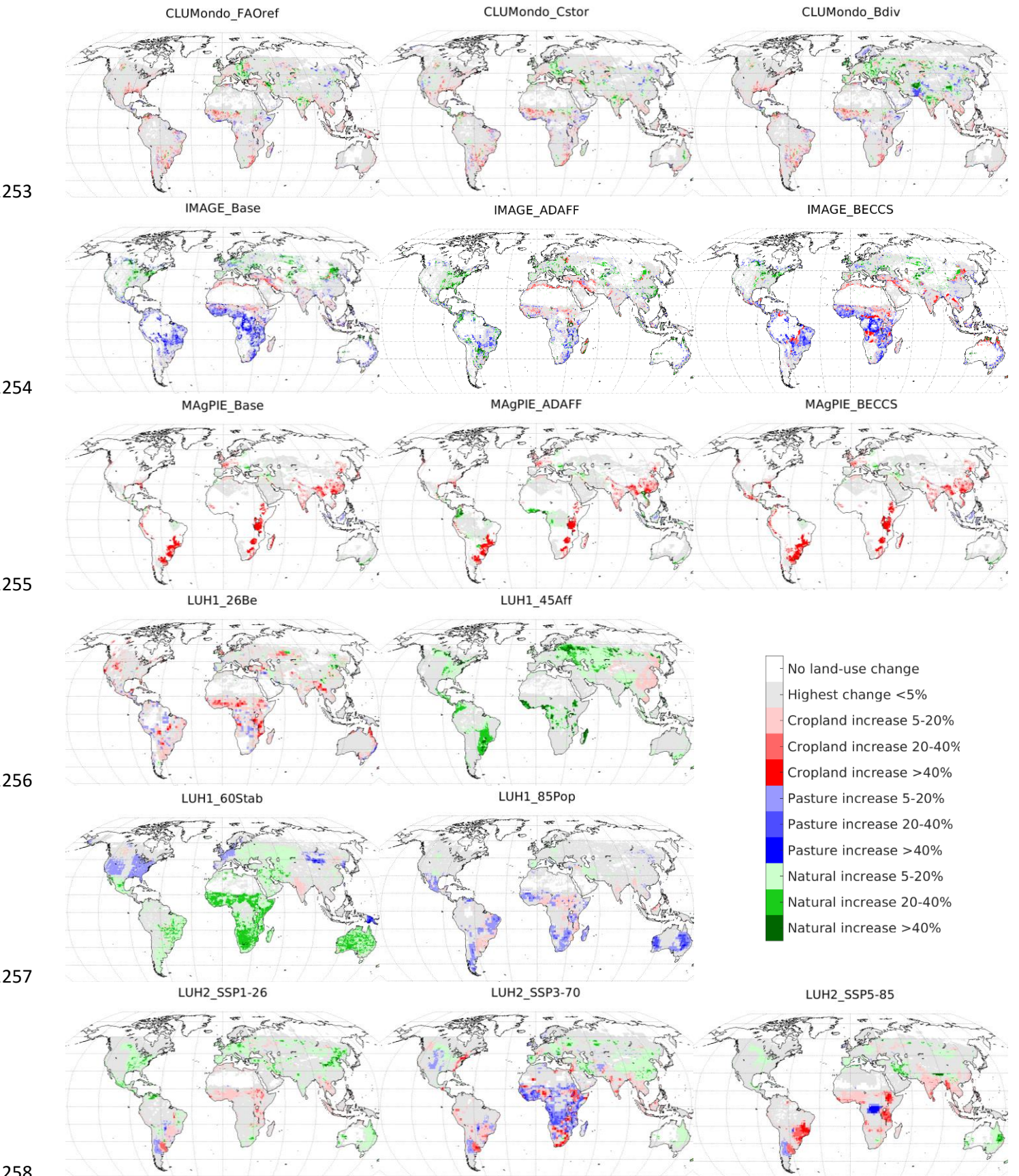
259 Fig. 2. Categories of dominant land-use change from 2000-2004 to 2036-2040 for each of 16 land-use scenarios. The 260 legend is identical for all plots.
