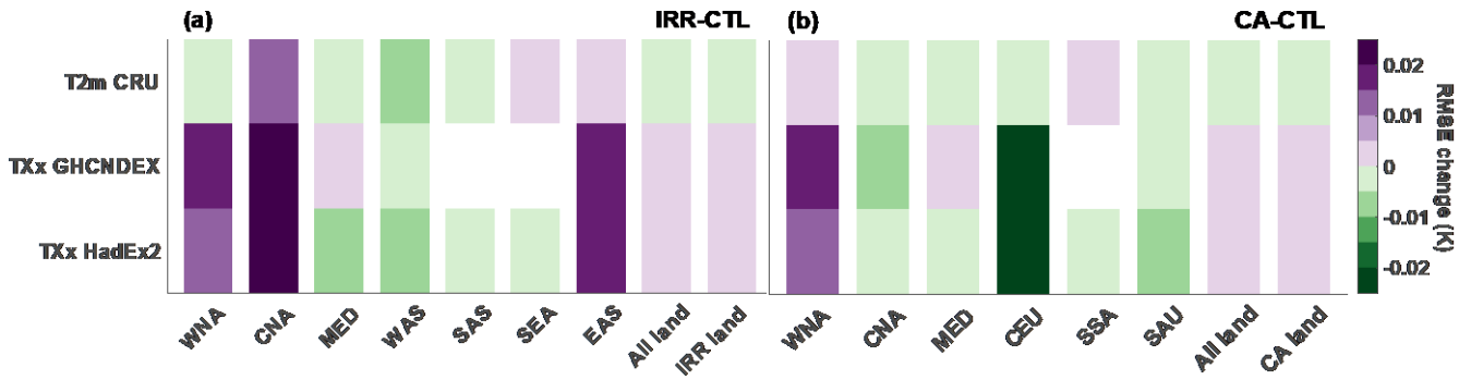
725 Figure 2. Added value of including irrigation and CA in the simulated warming trends over 1981-2010. Absolute change in spatial root-mean-square error (RMSE) for the (a) IRR and (b) CA ensemble relative to the CTL ensemble over different regions (x axis) and with respect to 3 observational products (y axis). Considered regions are the SREX regions where irrigation is extensive (as highlighted in Figure 1a) and where CA is extensive (Figure 1b), in addition to global land, global irrigated land and global CA land. Observational products are for near-surface air temperature T_{2m} (CRU), annual maximum daytime temperature TXx (GHCNDEX and HadEX2). The spatial RMSEs are computed for the ensemble mean warming trend in every pixel, and subsequently averaged over the selected region. Regions with an observational coverage below 50% are marked in white.
