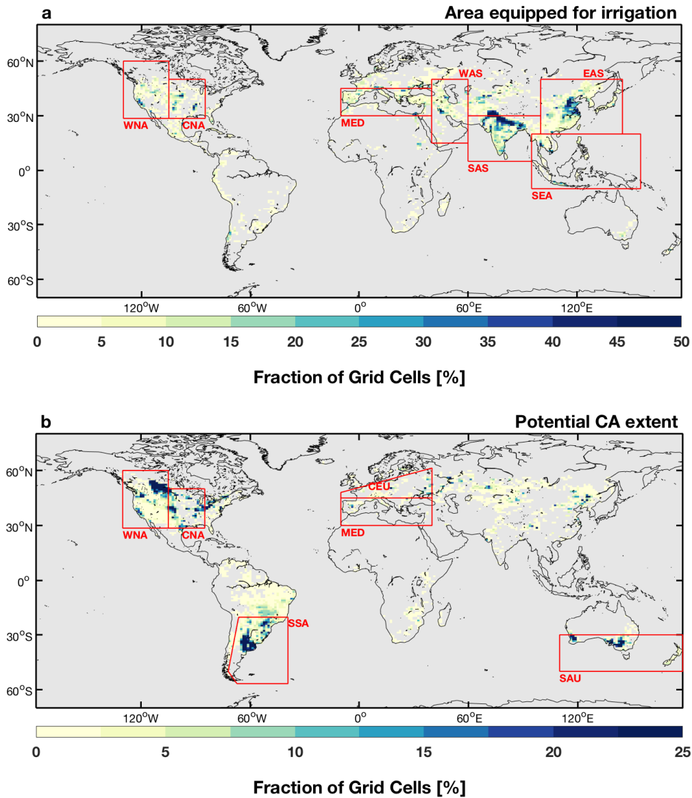
715 Figure 1. (a) Percentage of each grid cell equipped for irrigation (%) (Siebert et al. , 2005). (b) Potential estimate of CA extent mapped to the CLM crop PFT (Prestele et al. , 2018). The red boxes in (a) denote the regional domains where irrigation is extensive and were thus examined in greater detail including Western North America (WNA), Central North America (CNA), south Europe and Mediterranean (MED), West Asia (WAS), South Asia (SAS), Southeast Asia (SEA), and East Asia (EAS). The red boxes in (b) denote the regional domains where CA is extensive and were thus examined in greater detail including WNA, CNA, MED, South-eastern South America (SSA), Central Europe (CEU) and Southern Australia (SAU).
