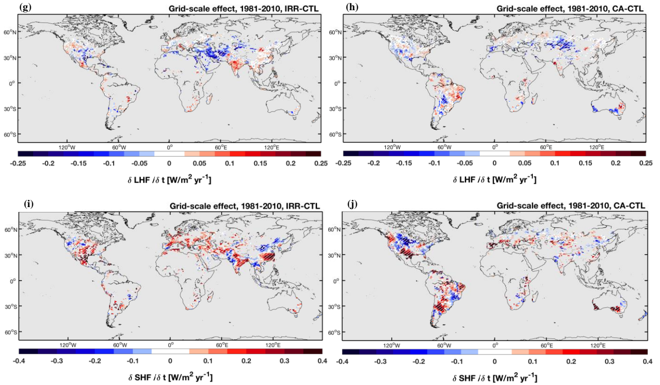
780 Figure 6. Grid-scale differences between the CTL and IRR ensemble (IRR minus CTL) (a, c, e, g and i) and between the CTL and CA ensemble (CA minus CTL) (b, d, f, h and j). For T_s (a-b), TMQ (c-d), ET (e-f), LHF (g-h) and SHF (i-j), displayed over irrigated/CA pixels for comparative purposes. Differences are based on the ensemble mean warming trends of each experiment for 1981–2010. Hatching denotes less than 10% change induced by the model on mean warming trends of lumped ensemble members.
