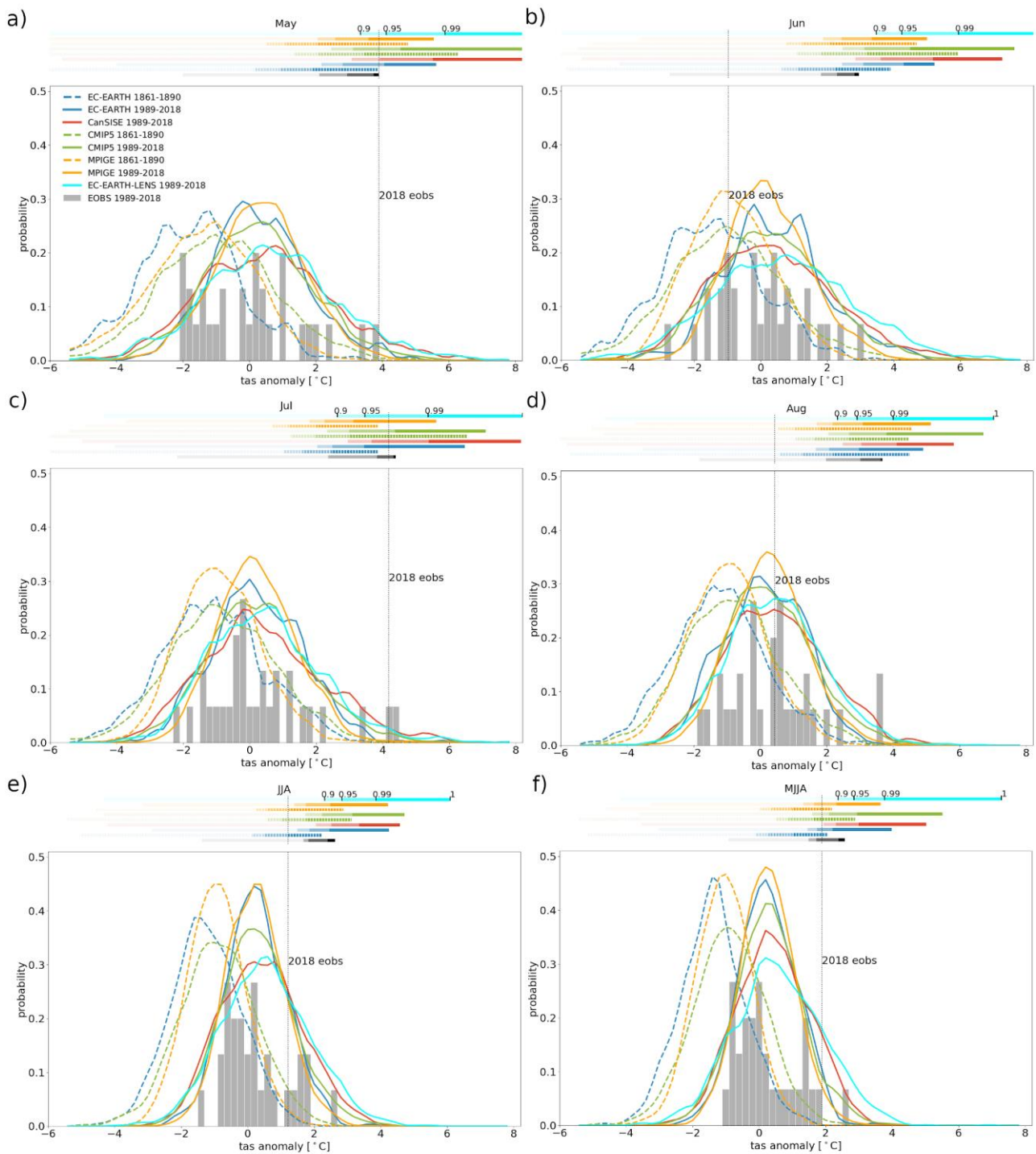
10 Figure S3. As in Figure 2 but for the Northern half of Sweden (as defined in Fig. S1 red).
