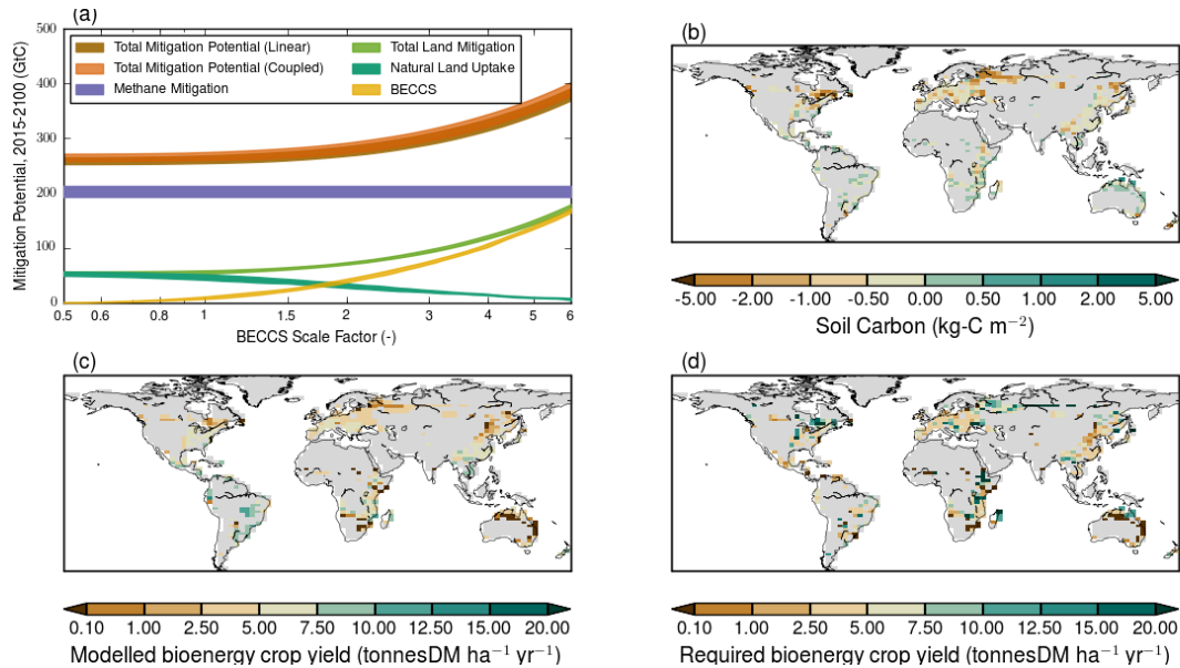
1081 Figure 10 (a) The total and component mitigation potential (GtC) for different mitigation options, involving methane and land use, as a function of the 1082 BECCS efficiency factor ( \kappa , Sect. 2.4.3) for the temperature pathway reaching 1.5°C. The spread of the functions width of the lines represent the 1083 interquartile range of the sensitivity-136-member ensembles. Maps of (b) the change of the modelled soil carbon (kg-C m -2 ) between 2015 and 2099, as the 1084 difference between the scenario with BECCS and the natural land-management scenario; (c) the modelled mean bioenergy crop yield in the JULES 1085 simulations ( \kappa = 1 ) and (d) the required bioenergy crop yield for BECCS to provide a larger carbon uptake than forest regrowth/afforestation (assuming 1086 \kappa = \kappa^* and 87% efficiency of BECCS). Grid cells which do not exceed 1% BECCS cover for any year in the simulation are masked grey.
