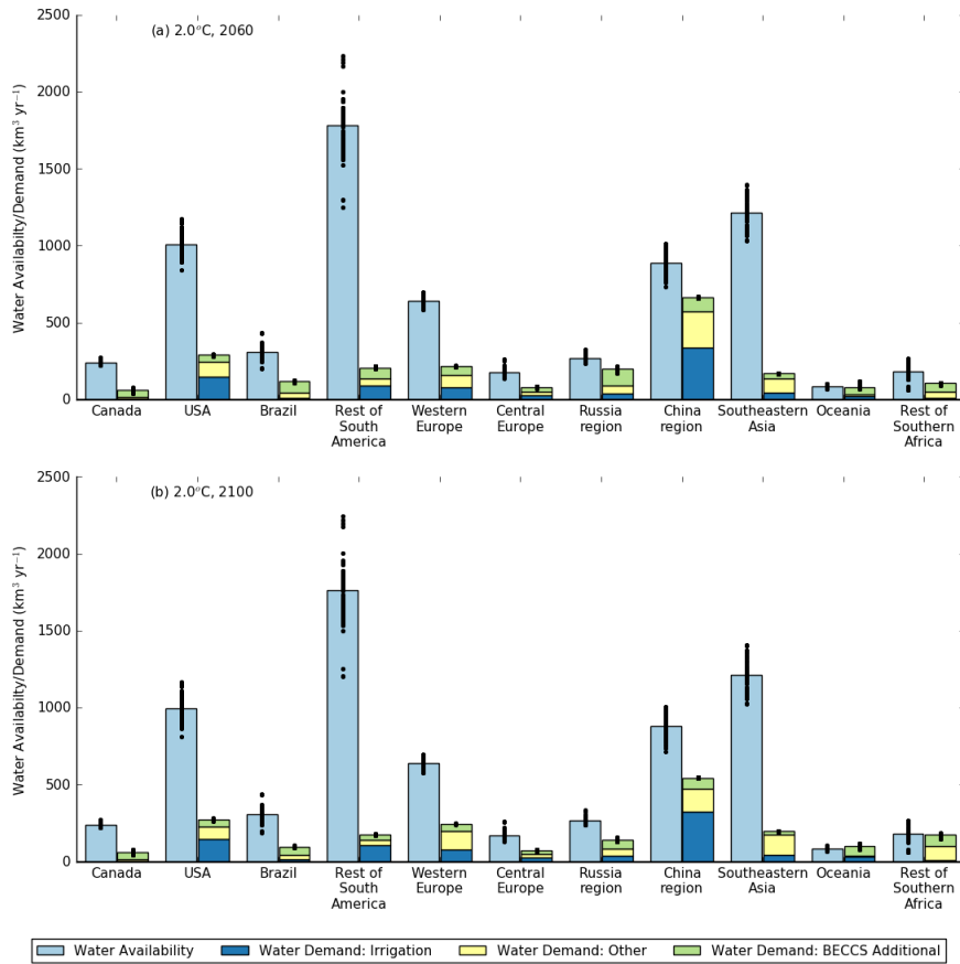
1112 Figure 14 | Water availability (light blue), SSP2-IMAGE water demand estimates for irrigation (dark blue), other uses (i.e., energy 1113 generation, industry and domestic; yellow) and the additional water demand from BECCS (green) for the years 2059-2060 and 2099- 1114 2100 for the 2.0°C warming target, with a BECCS \kappa factor of 3. The points are the individual results from the 34 GCMs emulated 1115 and 4 factorial runs 136-member ensembles, while the bars are the corresponding median values of the different GCM/factorial 1116 ensembles.
