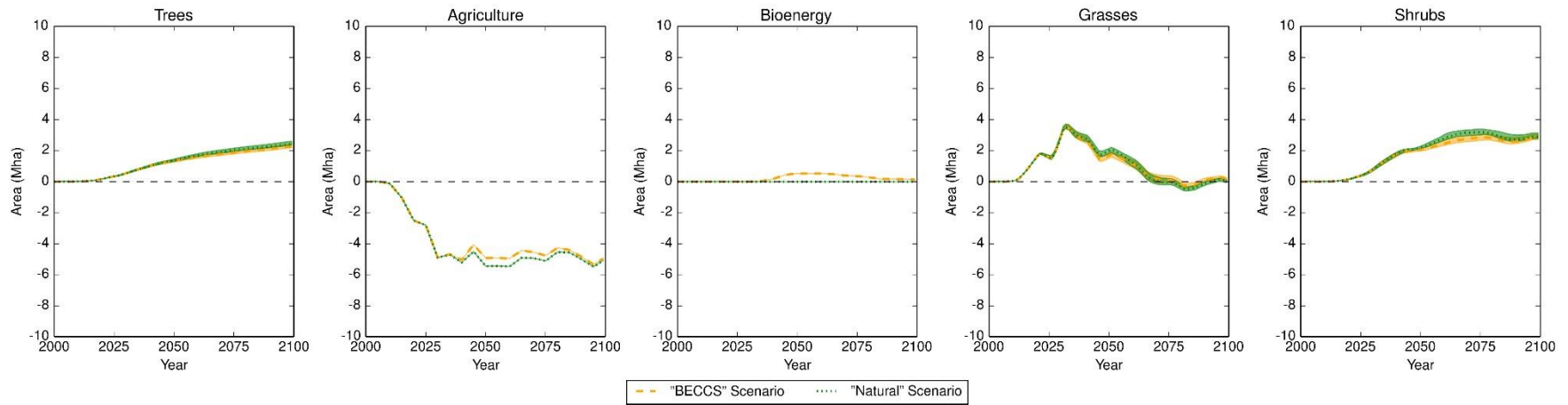
Fig. SI.2d: Central America
