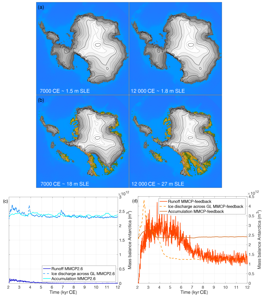
Figure 11. (a) Antarctic ice sheet configuration at 7000 CE and 12 000 CE using scenario MMCP2.6 and (b) MMCP-feedback. Only grounded ice is shown. Main mass balance components (over grounded ice) explaining the change in ice sheet geometry for scenarios MMCP2.6 (c) and MMCP-feedback (d). GL: grounding line. Note that the land–sea mask has not changed due to the change in GMSL but only due to isostatic changes. CE1
