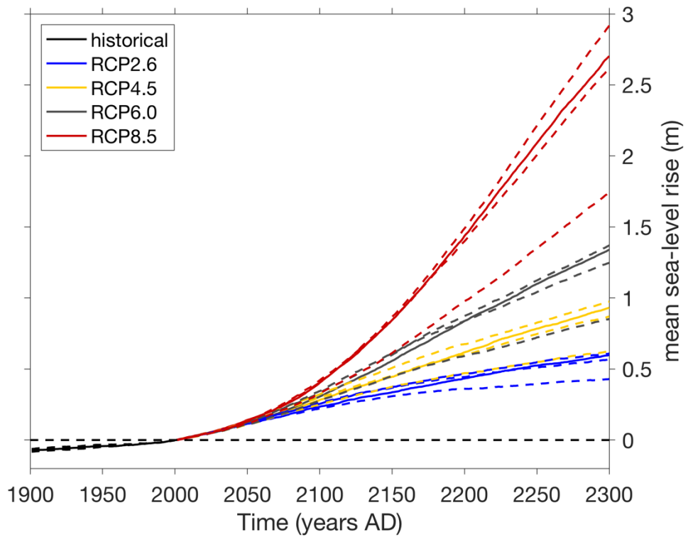
Figure S1: Global mean sea level change for the period 1900-2300 AD using 4 different parameter sets of LOVECLIM.
