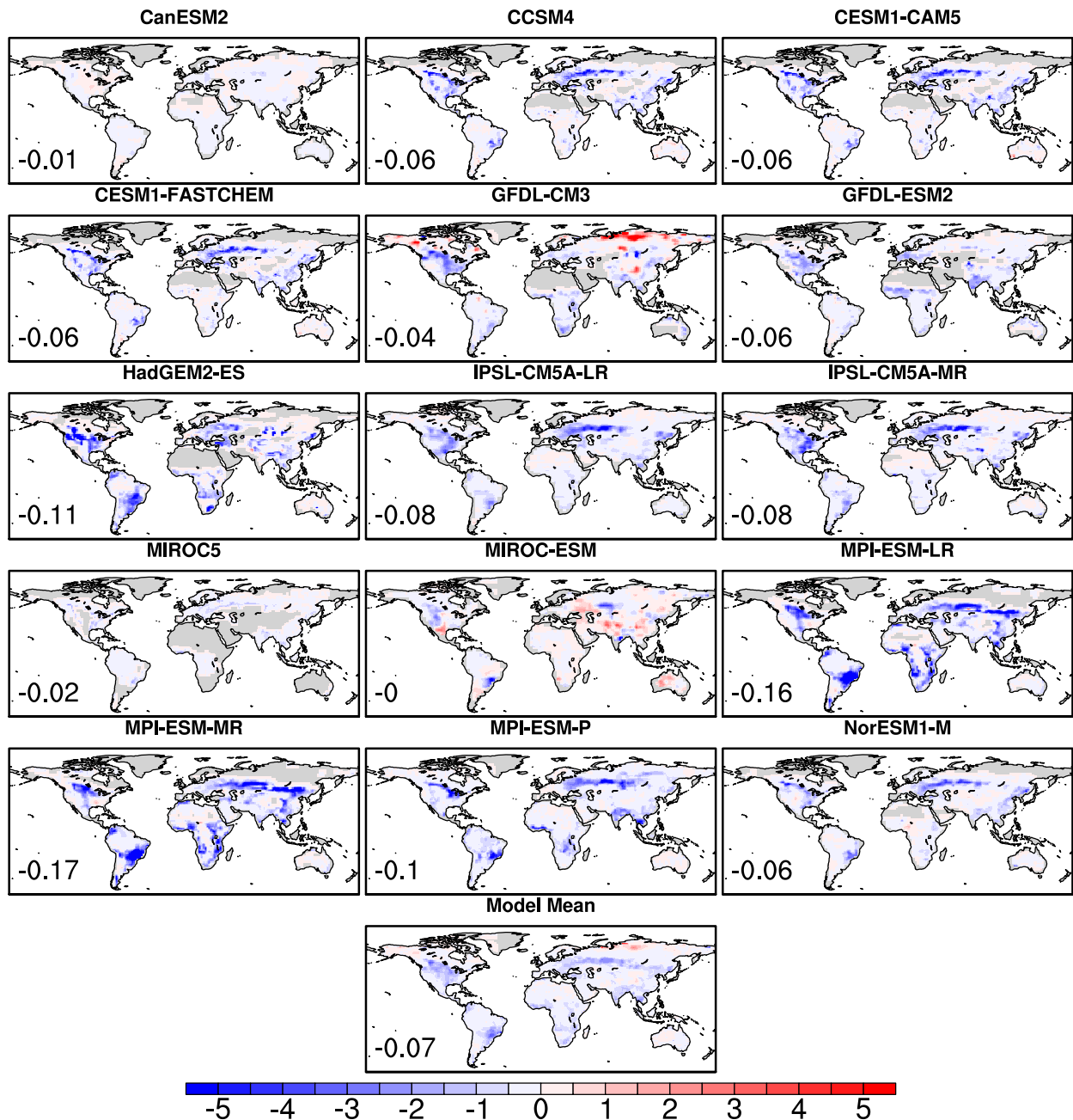
Figure 12: Radiative Forcing from historical conversions between trees and crops/grasses (from the pre-industrial to the 1981-2000 period) in the analysed CMIP5 models (in \text{W/m}^2 ), obtained by applying the reconstruction method (see the description of the methodology in Section 2.4). The numbers in the bottom-left corner of each map indicate the global mean Radiative Forcing. For the computation of the Model Mean, if several CMIP5 models contain the same Land Surface Model they were attributed a lower weight so that the sum of their weights equal 1.
