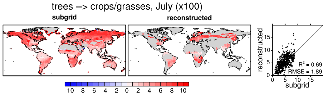
820 Figure 4: Subgrid (left) and reconstructed (right) estimates of the present-day (2002-2010) potential albedo change associated to a transition from trees to crops/grasses in the CLM4.5 simulations, for the month of July. Note that absolute differences have been multiplied by 100 to facilitate reading.
