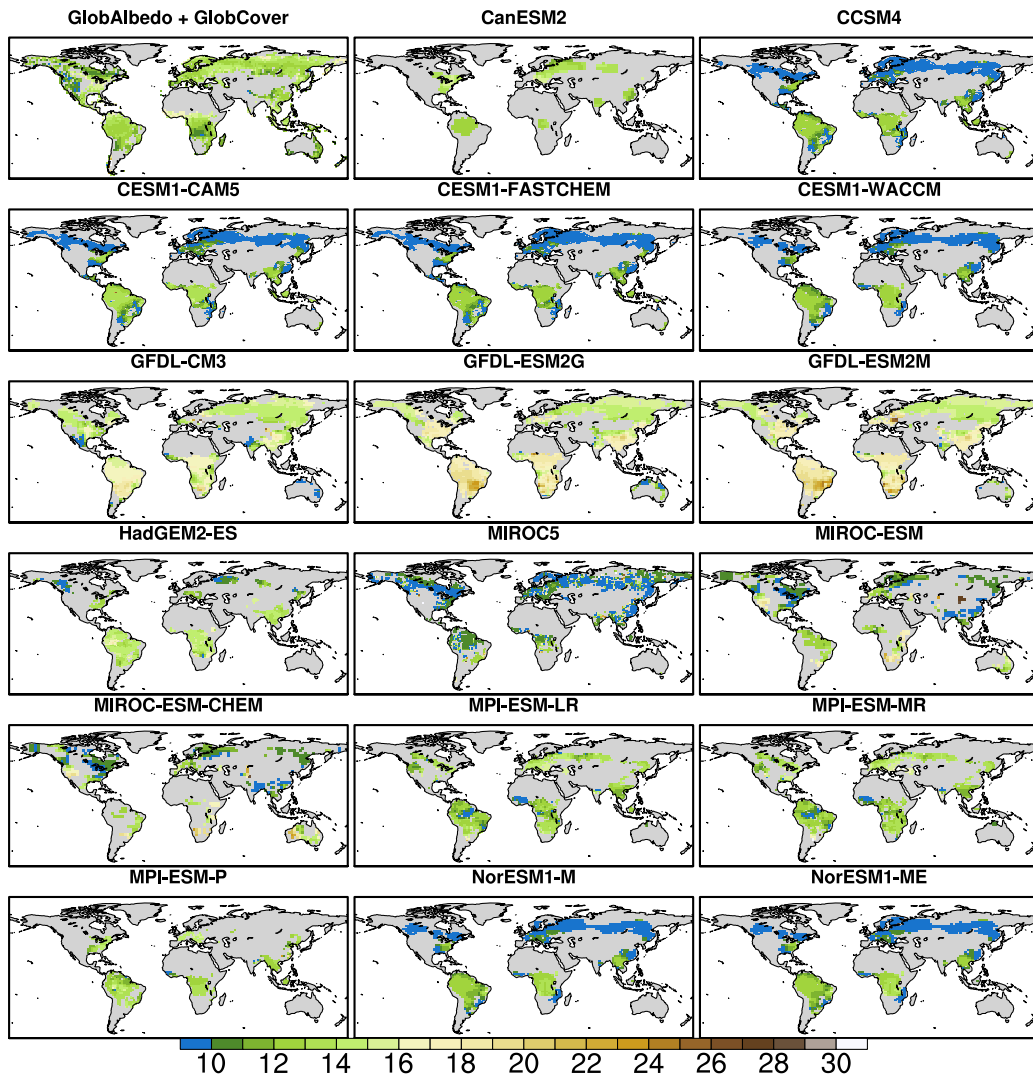
Figure 6: Present-day July albedo of trees retrieved from the combination of the observational data GlobAlbedo (over the 1998-2011 period) and GlobCover (2005-2006, top-left corner), and in the analysed CMIP5 models (the climatology over the 2000-2004 period was considered). Note that the albedo values have been multiplied by 100 to facilitate readability.
