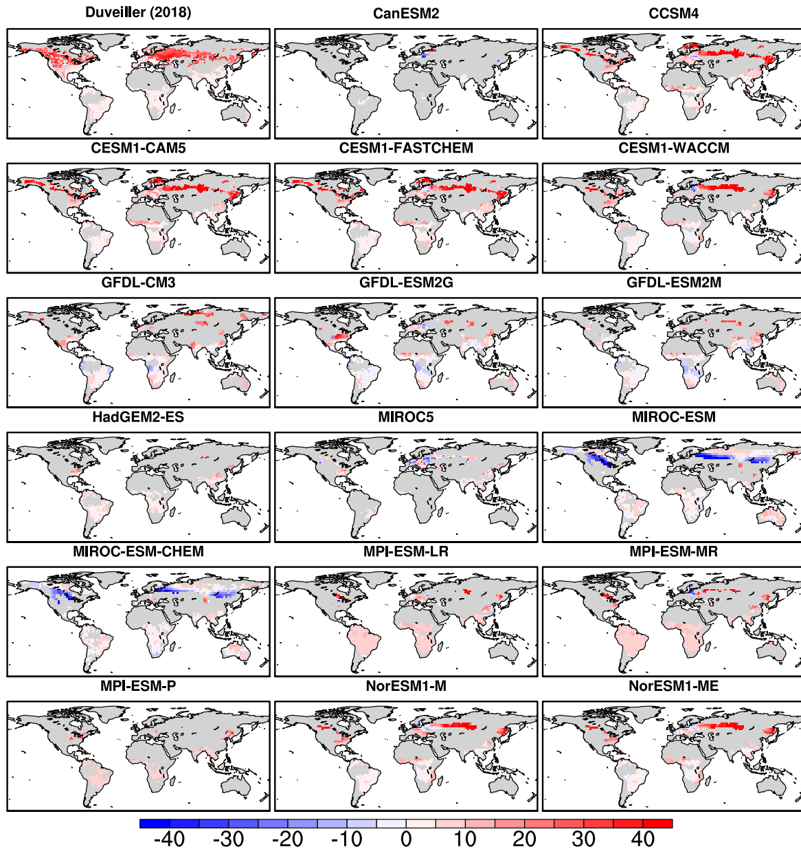
845 Figure 11: Same as Figure 10, but for January. Note that the scale is different.
