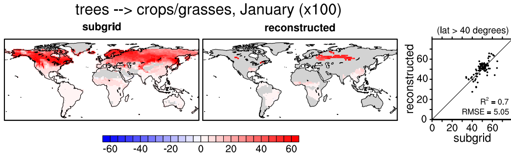
825 Figure 5: Same as Figure 4, but for the month of January. The scatter plots in this case only display the results for the grid cells north of 40° (i.e., over areas considered as snow-covered). Note that the scale is different.
