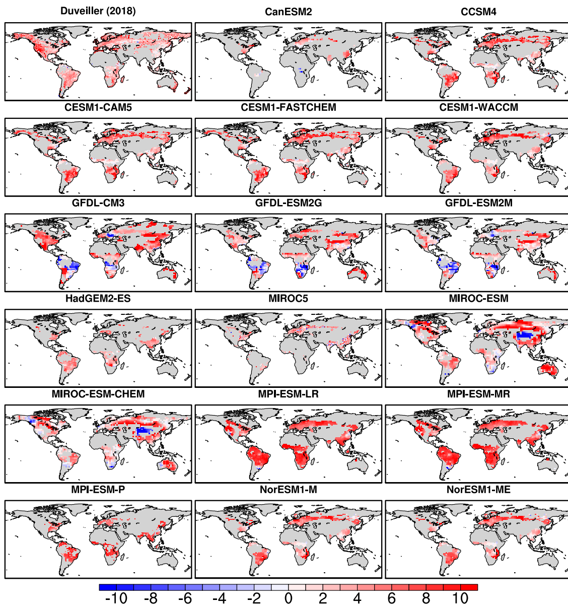
840 Figure 10: Potential present-day July albedo change associated to a transition from trees to crops/grasses according to the observational dataset of Duveiller, Hooker and Cescatti (2018a, derived from satellite data collected over the 2008-2012 period, top-left corner) and in the analysed CMIP5 models (the climatology over the 2000-2004 period was reconstructed). Note that the absolute differences have been multiplied by 100 to facilitate readability.
