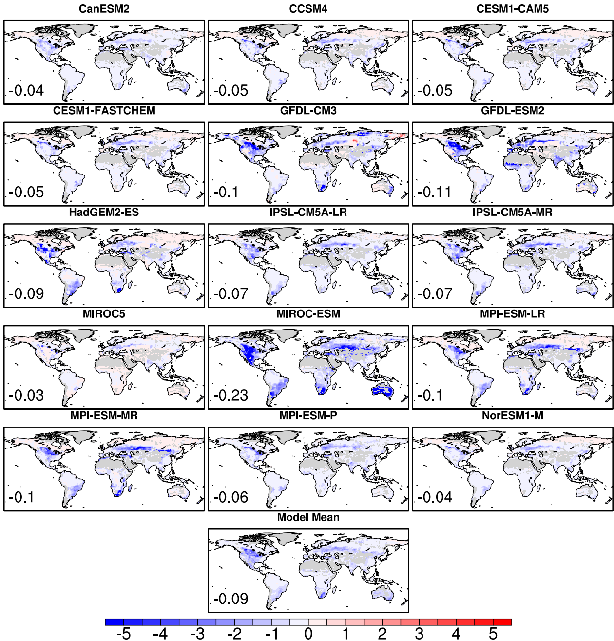
Figure 13: Same as Figure 12, but for the observation-constrained Radiative Forcing from historical conversions between trees and crops/grasses.
