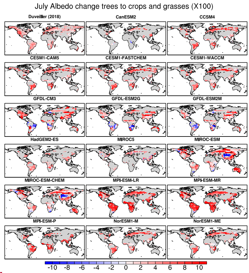
015 Figure 10: Potential present-day July albedo change associated to a transition from trees to crops/grasses according to the observational dataset of Duveiller, Hooker and Cescatti (2018a, derived from satellite data collected over the 2008-2012 period , top-left corner) and in the analysed CMIP5 models ( the climatology over the 2000-2004 period was reconstructed ). Note that the absolute differences have been multiplied by 100 to facilitate readability.
