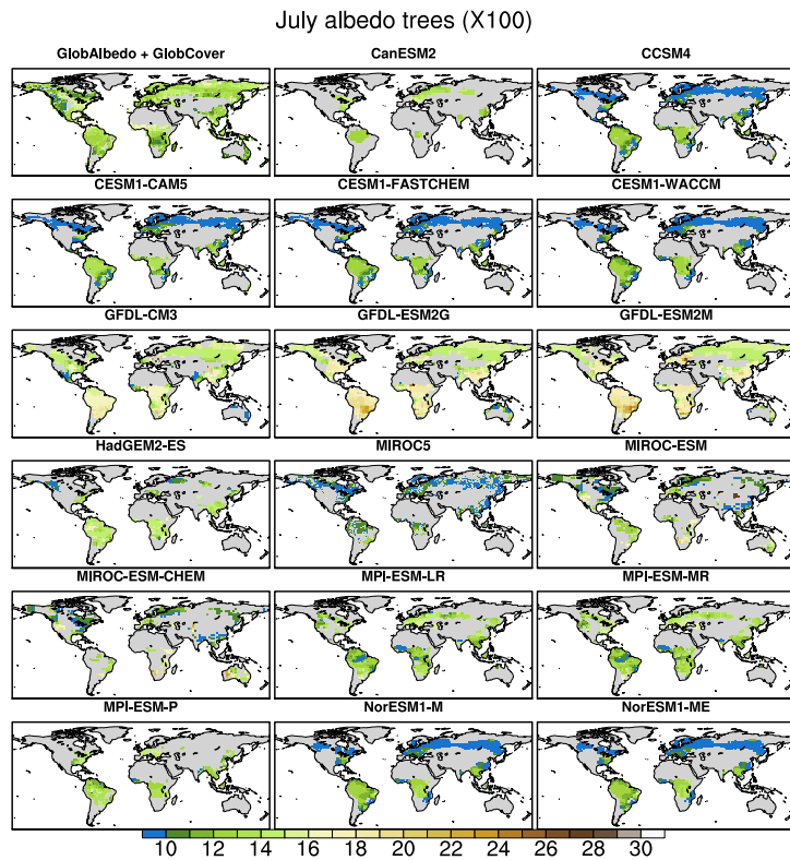
995 Figure 6: Present-day July albedo of trees retrieved from the combination of the observational data GlobAlbedo (over the 1998-2011 period) and GlobCover (2005-2006, top-left corner), and in the analysed CMIP5 models (the climatology over the 2000-2004 period was considered). Note that the albedo values have been multiplied by 100 to facilitate readability.
