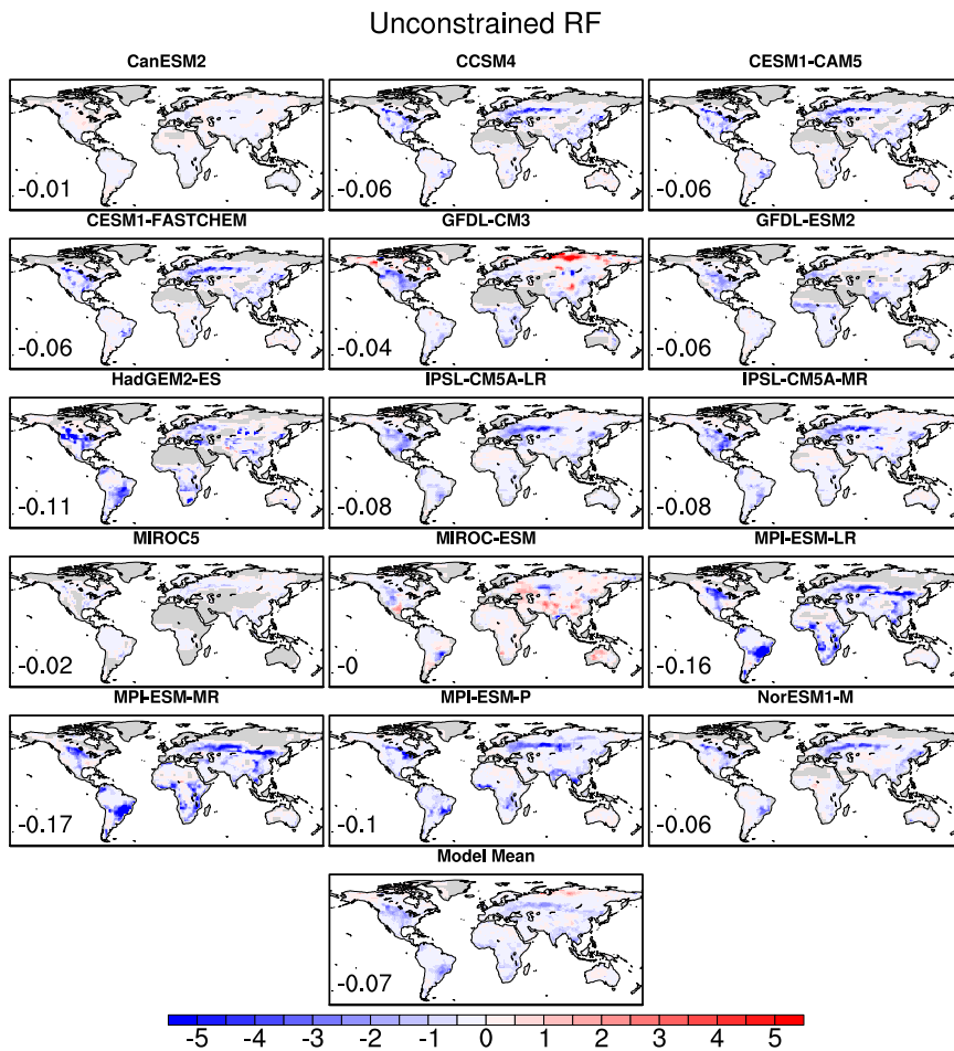
1025 Figure 12: Radiative Forcing from historical conversions between trees and crops/grasses (from the pre-industrial to the 1981-2000 period) in the analysed CMIP5 models (in W/m 2 ), obtained by applying the reconstruction method (see the description of the methodology in Section 2.4). The numbers in the bottom-left corner of each map indicate the global mean Radiative Forcing. For the computation of the Model Mean, if several CMIP5 models contain the same Land Surface Model they were attributed a lower weight so that the sum of their weights equal 1.
