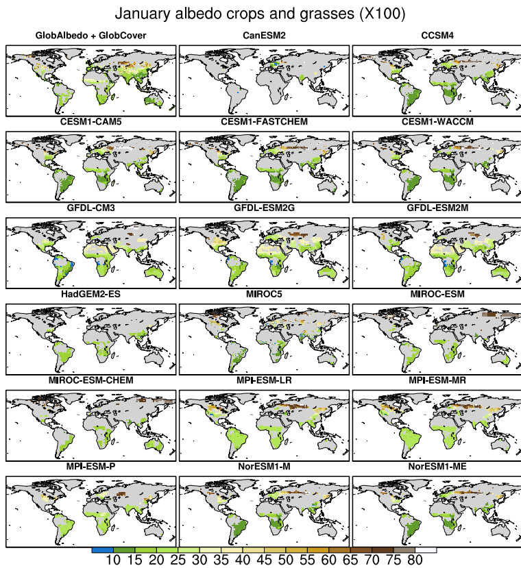
Figure 9: Same as Figure 8, but for the month of January. Note that the scale is different.
