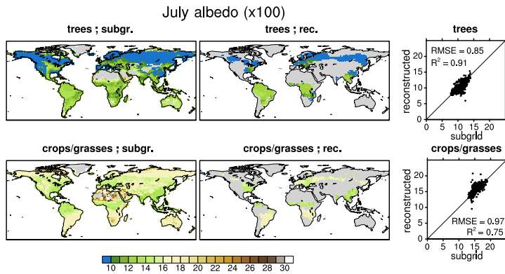
970 Figure 2: Subgrid (left) and reconstructed (middle) estimates of the present-day (2002-2010) albedo of trees (upper row) and crops/grasses (lower row) in the CLM4.5 simulations, for the month of July. The scatter plots (right) indicate the relationship between reconstructed (y-axis) and subgrid estimates (x-axis), with each dot indicating the results of a grid cell for which both methods could be applied. Note that albedo values have been multiplied by 100 to facilitate readability.
