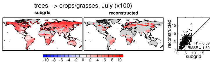
985 Figure 4: Subgrid (left) and reconstructed (right) estimates of the present-day (2002-2010) potential albedo change associated to a transition from trees to crops/grasses in the CLM4.5 simulations, for the month of July. Note that absolute differences have been multiplied by 100 to facilitate reading.
