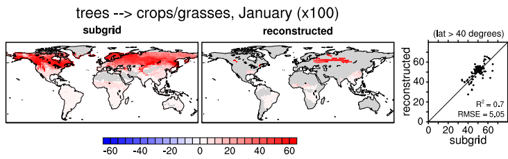
990 Figure 5: Same as Figure 4, but for the month of January. The scatter plots in this case only display the results for the grid cells north of 40° (i.e., over areas considered as snow-covered). Note that the scale is different.
