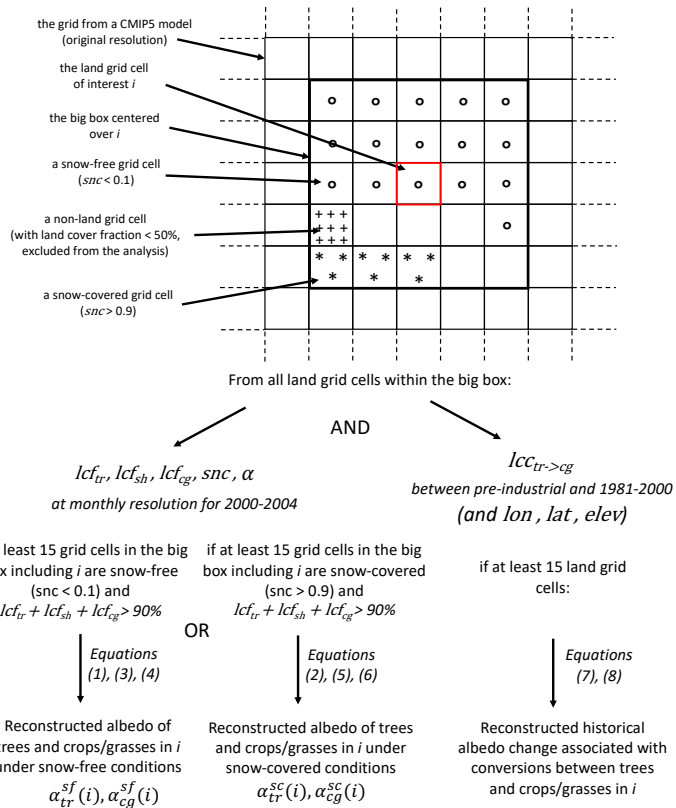
965 Figure 1: Description of the two employed reconstruction methodologies. snc stands for snow cover fraction, \alpha for albedo, lcf for land cover fraction, lcc for land cover conversion, the suffixes tr, sh and cg for trees, shrubs and crops/grasses, respectively, lon for longitude, lat for latitude, and elev for elevation.
