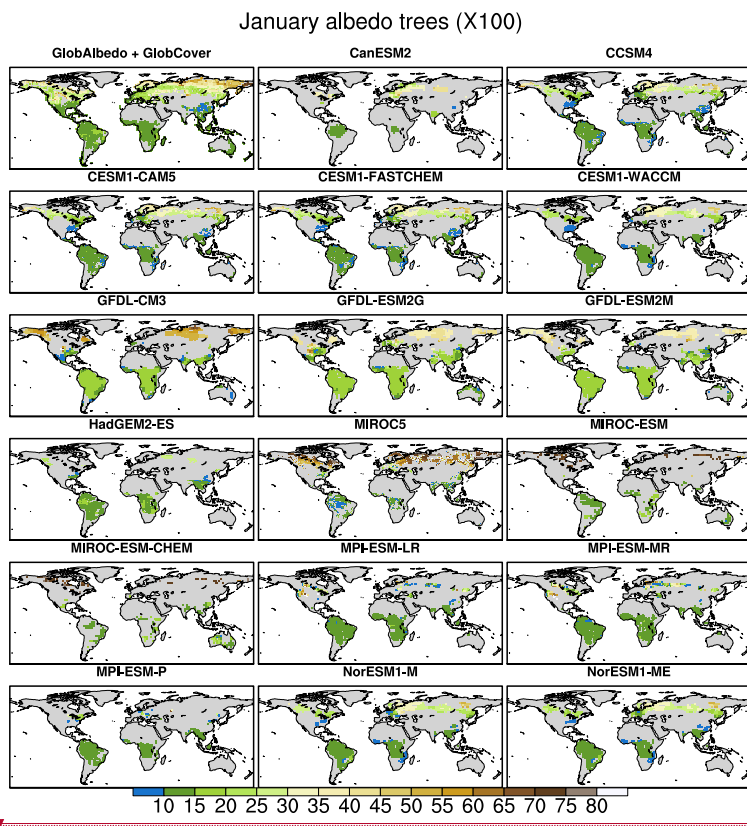
Figure 7: Same as Figure 6, but for the month of January. Note that the scale is different.
