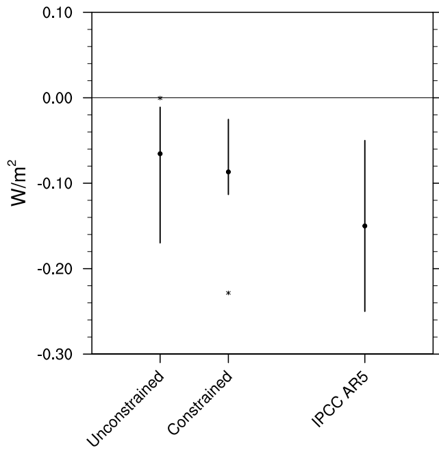
1040 Figure 14: Spread in the unconstrained (left bar) and observation-constrained (middle bar) estimates of the global Radiative Forcing 1045 from historical conversions between trees and crops/grasses (from the pre-industrial to the 1981-2000 periods), for the CMIP5 models shown in Figures 11 and 12 (in W/m^2 ), as well as the IPCC AR5 estimate of the global Radiative Forcing from historical land-use changes (mean estimate and spread as in Myhre et al. , 2013). The dots on the left and middle bars show the Model Mean results for the unconstrained and observation-constrained estimates, respectively, the asterisks mark the results for the MIROC- ES model, while the lengths of the bars indicate the spread between the remaining values (i.e., excluding MIROC-ES ).
