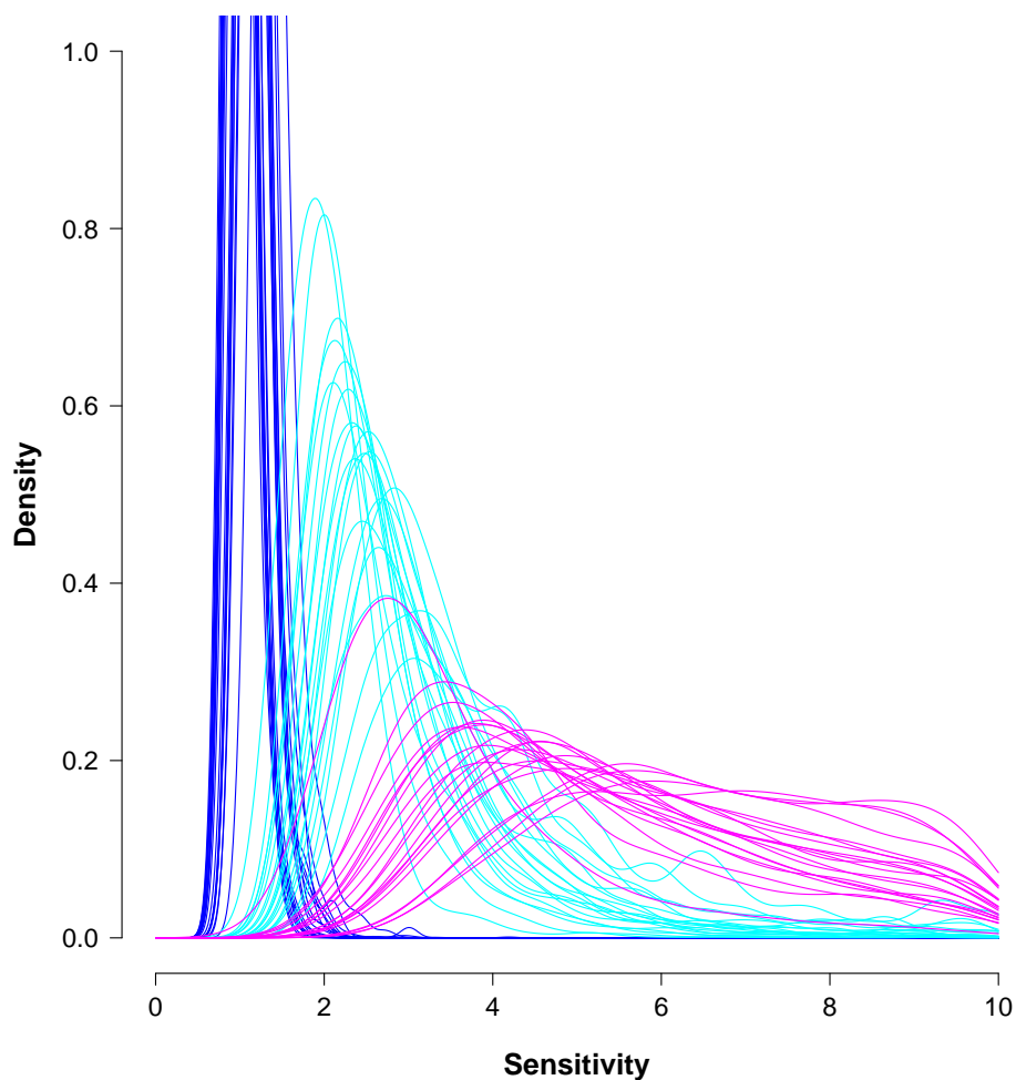
Figure 8. As Figure 7 but for multiple parametric uncertainties.
