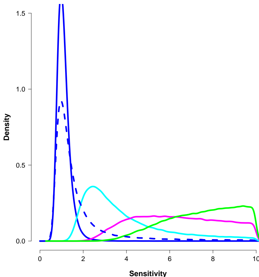
Figure 2. Posterior estimates of sensitivity based on \Psi estimated from 150y time series with unforced 2-layer model. Four solid-line pdfs in blue, cyan, magenta and green represent estimates based on \Psi^o = 0.05, 0.1, 0.15, and 0.2 respectively, where only S is uncertain with uniform prior. Dotted blue line represents posterior estimate for \Psi^o = 0.05 with additional modelling uncertainties as described in main text.
