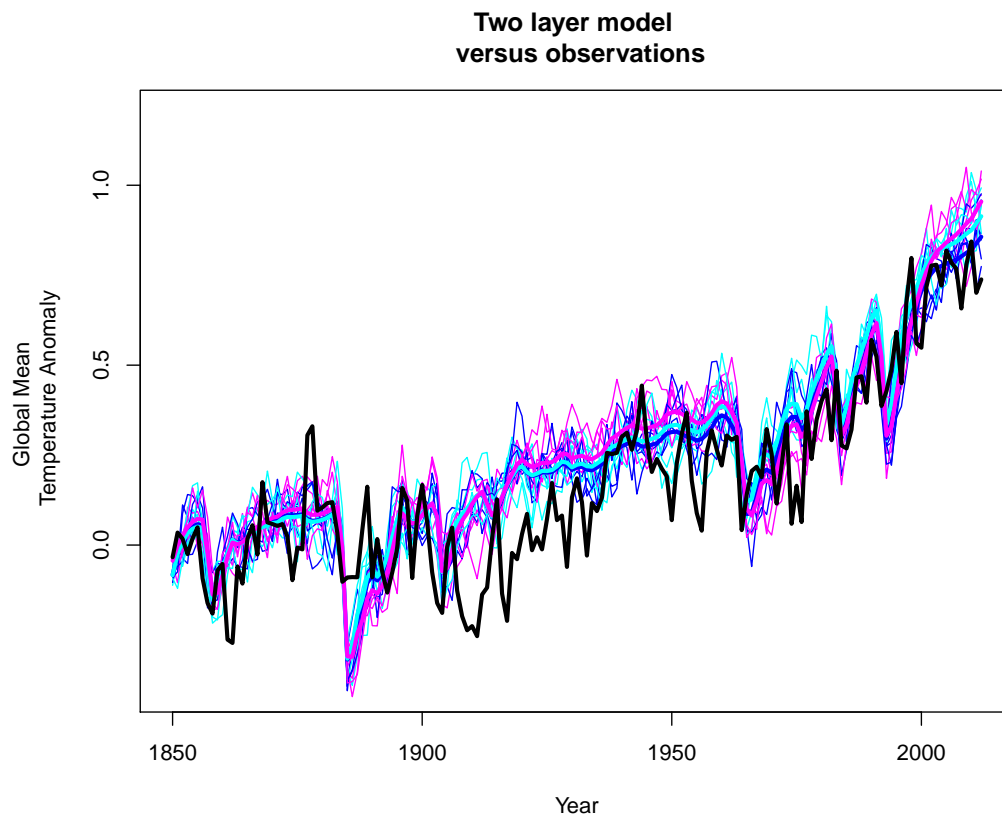
Figure 4. Simulations of instrumental period with 2-layer model. Thick lines are forced response excluding internal variability, thin lines are 5 replicates of each parameter set including internal variability. Blue lines: S = 1.78^{\circ}\text{C} , \gamma = 0.7\text{Wm}^{-2} \text{ }^{\circ}\text{C}^{-1} , \epsilon = 1.3 . Cyan lines: S = 2.5^{\circ}\text{C} , \gamma = 1.0\text{Wm}^{-2} \text{ }^{\circ}\text{C}^{-1} , \epsilon = 1.7 . Magenta lines: S = 5^{\circ}\text{C} , \gamma = 1.0\text{Wm}^{-2} \text{ }^{\circ}\text{C}^{-1} , \epsilon = 1.7 , \alpha = 1.7 . Black line is HadCRUT data.
