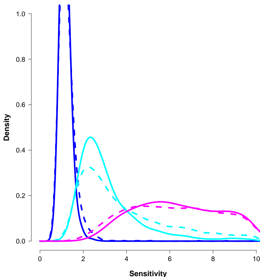
Figure 6. Posterior estimates of sensitivity based on \Psi estimated from 20th century simulations with 2-layer model. Three solid-line pdfs in blue, cyan and magenta represent estimates based on \Psi^o = 0.1, 0.18, and 0.25 respectively, where only S is uncertain with uniform prior. Dashed lines represent equivalent posteriors with additional modelling uncertainties as described in main text.
