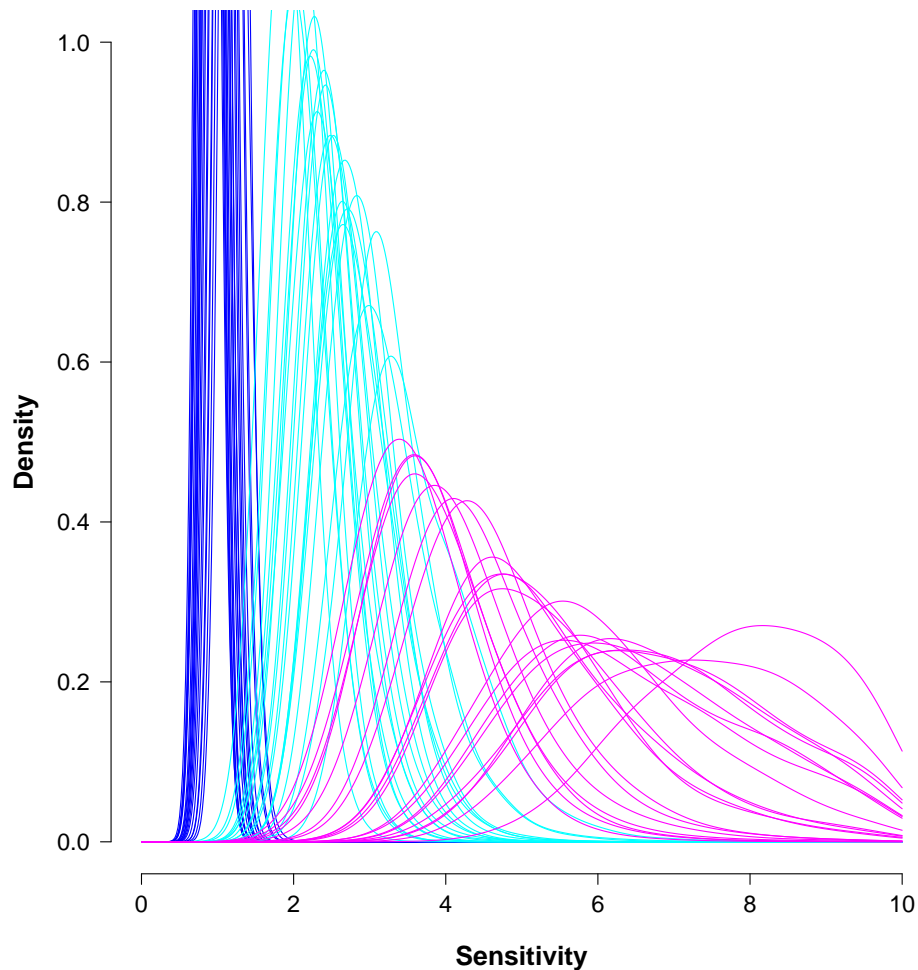
Figure 7. Posterior estimates for the climate sensitivity using Bayesian estimation using the full 1880–2012 observational time series of annual mean surface temperature anomalies after detrending. 20 replicates are performed for each true sensitivity of 1, 2.5, 5°C as indicated by colours blue, cyan and magenta respectively. Only S is considered uncertain.
