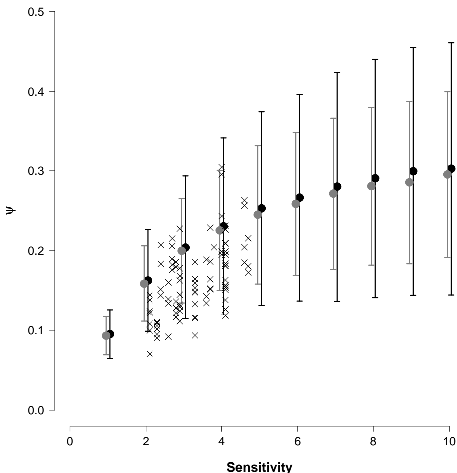
Figure 5. \Psi estimated from 20th century simulations from 2-layer model. Grey results are based on simulations where only S is considered uncertain. Black results additionally account for uncertainty in \gamma , \epsilon , \sigma and \alpha . Large dots show means of 1000 simulations, with error bars indicating \pm 2\text{sd} ranges for each ensemble. Crosses indicate results generated by CMIP5 models.
