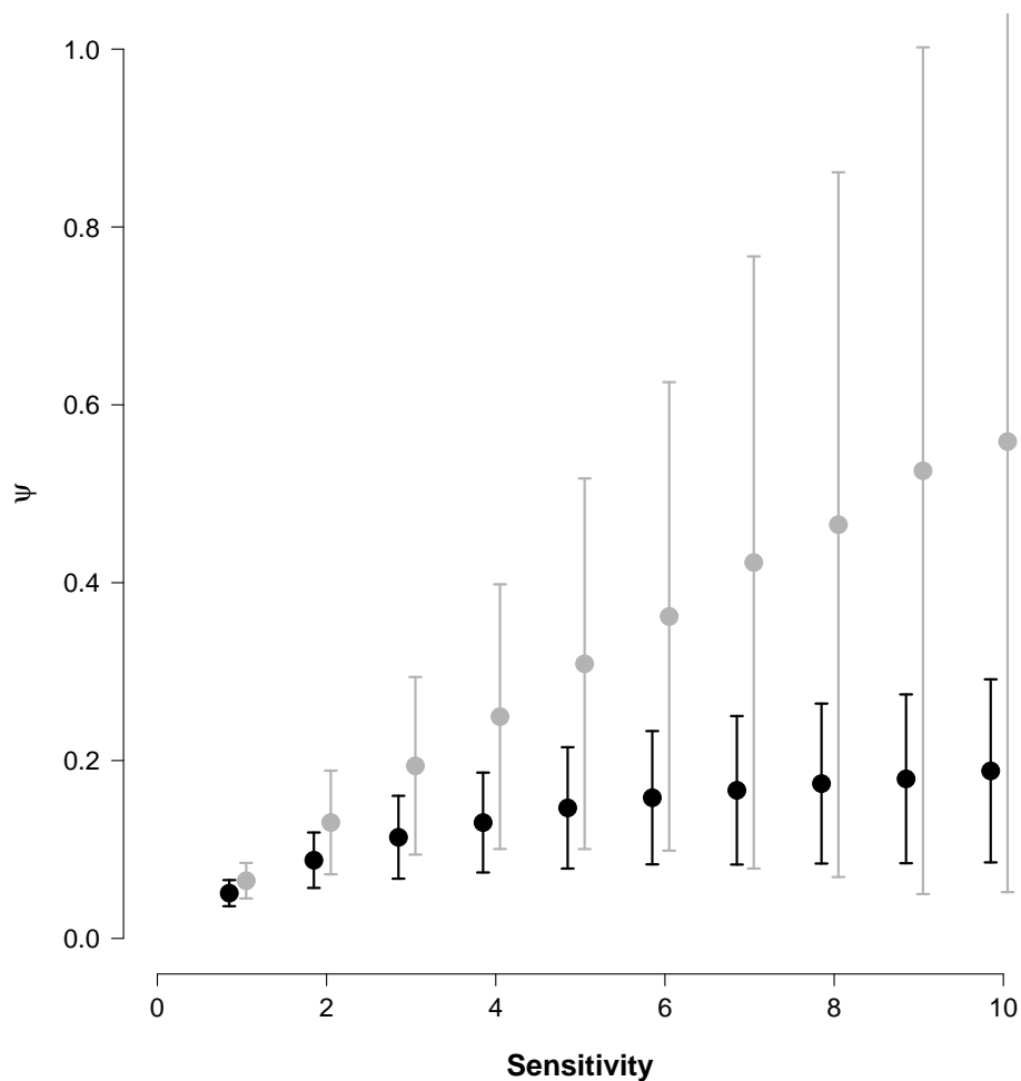
Figure 1. \Psi estimated from 150y time series for 1- and 2-layer model. Grey results are for single-layer model and black results for two-layer model. Large dots show means of 1000 simulations, with error bars indicating \pm 2\text{sd} ranges for each ensemble. Results are calculated at each integer value of sensitivity and offset slightly for visibility.
