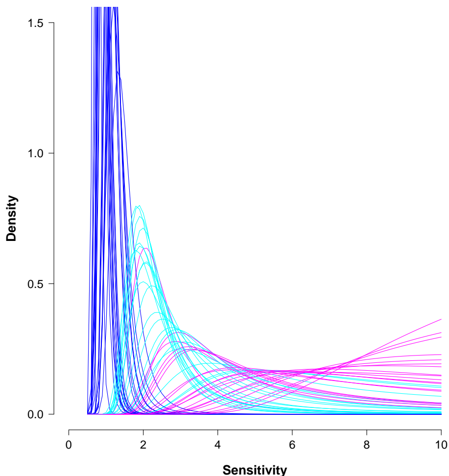
Figure 3. Posterior estimates for the climate sensitivity using Bayesian estimation using the full 150 year time series of annual mean surface temperatures. 20 replicates are performed for each true sensitivity of 1, 2.5, 5°C as indicated by the colour blue, cyan and magenta respectively.
