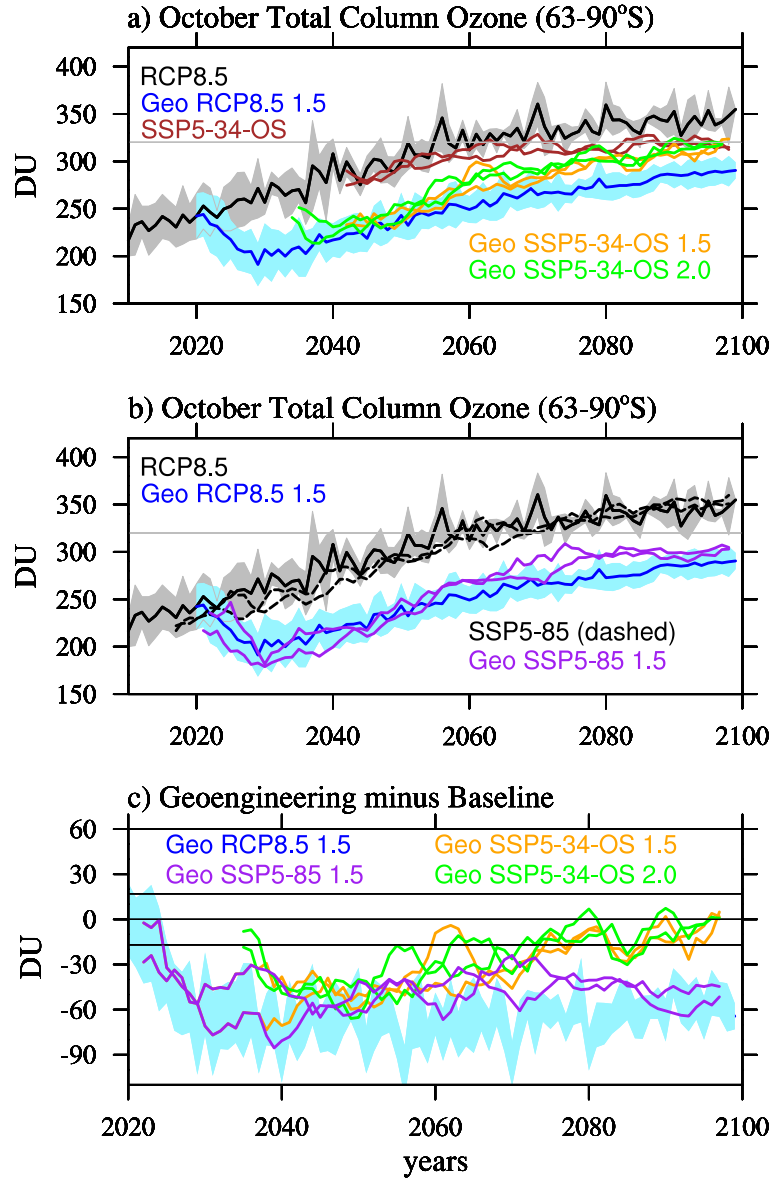
Figure 11. October averaged total column ozone between 63-90°S for different model experiments and ensemble members (different colors) (panel a and b). Grey and light blue areas show the standard deviation of the GLENS ensemble and the light grey line indicates 1980 values. Panel c: differences between geoengineering and corresponding baseline experiments, the two black lines around zero indicate the standard deviation from the GLENS baseline simulations. A running mean over 5 years has been applied to the results.
