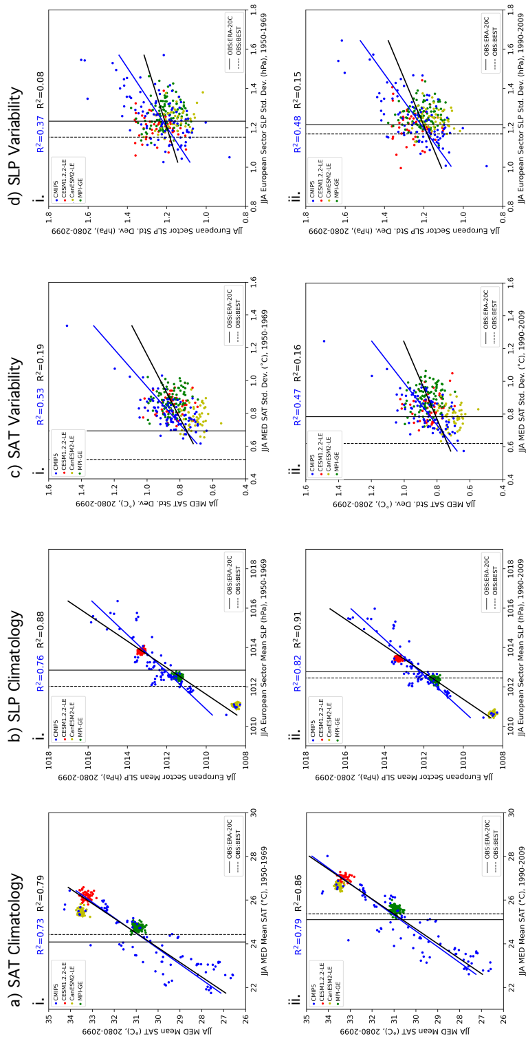
Figure C2. As in Figure C1, but for JJA and the MED region in columns a and c.
