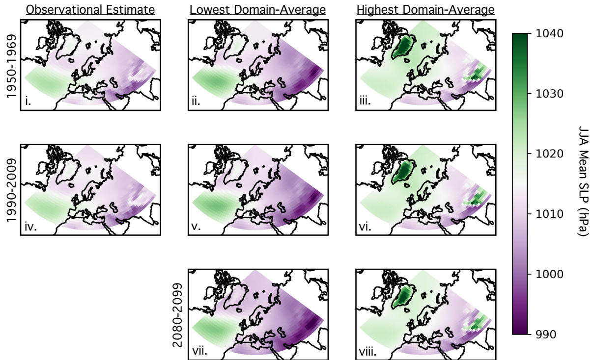
Figure C4. As in Figure C3, but for JJA SLP climatology.
