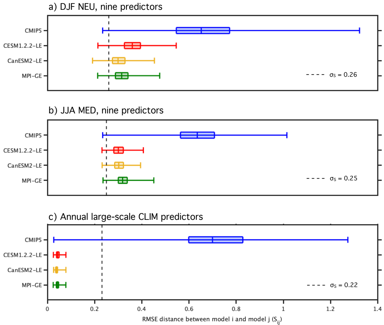
Figure B2. Distributions of RMSE distance ( S_{ij} ) within the SMILEs, the CESM1.2.2-LE (red), the CanESM2-LE (yellow), the MPI-GE (green) and the CMIP5 ensemble (blue). The box element spans the 25th to 75th percentile of the distribution; median S_{ij} is indicated by the horizontal line within the box. The whisker element spans the full range of the S_{ij} distribution. The value of \sigma_S used for the weighting is indicated by the dashed line. DJF NEU distances based on the nine predictors are shown in panel a, JJA MED distances based on the nine predictors are shown in panel b, and distances based on annual global land SAT and Northern Hemisphere SLP climatology are shown in panel c.
