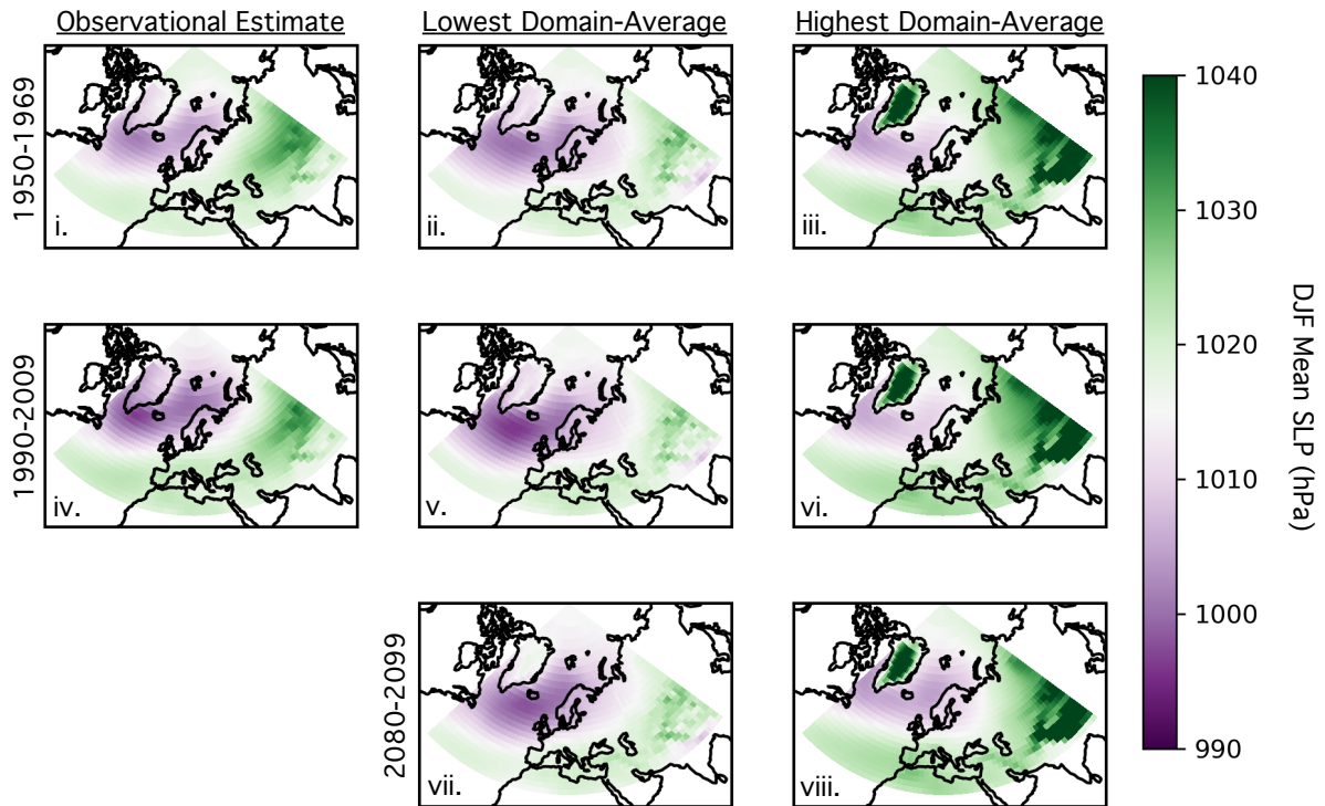
Figure C3. The spatial pattern of DJF SLP climatology for: 1950-1969 (i-iii), 1990-2009 (iv-vi), and 2080-2099 (vii-viii). The ERA-20C observational estimate of SLP climatology is shown in the left column (i,iv). The ensemble member with the lowest domain-average SLP climatology for the 1990-2009 historical period is shown in the center column (ii,v,vii). The ensemble member with the highest domain-average SLP climatology for the 1990-2009 period is shown in the right column (iii,vi,viii).
