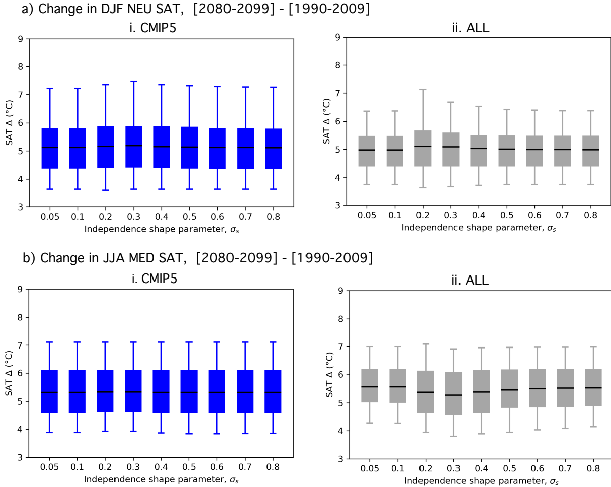
Figure B3. \sigma_S sensitivity of the nine predictor RMSE weighting in Figure 3. \sigma_S used for each weighting is indicated below each box element. Box-and-whiskers showing the SAT change distribution under the RMSE independence scaling weighting assumption ( \Delta , [2080-2099]-[1990-2009]) for the CMIP5 ensemble (i; blue) and ALL ensemble (ii; gray). The box element spans the 25th to 75th percentile of the distribution; mean SAT change is indicated by the horizontal line within the box. The whisker element spans the 5th to 95th percentile. DJF NEU SAT change is shown in a and JJA MED SAT change is shown b.
