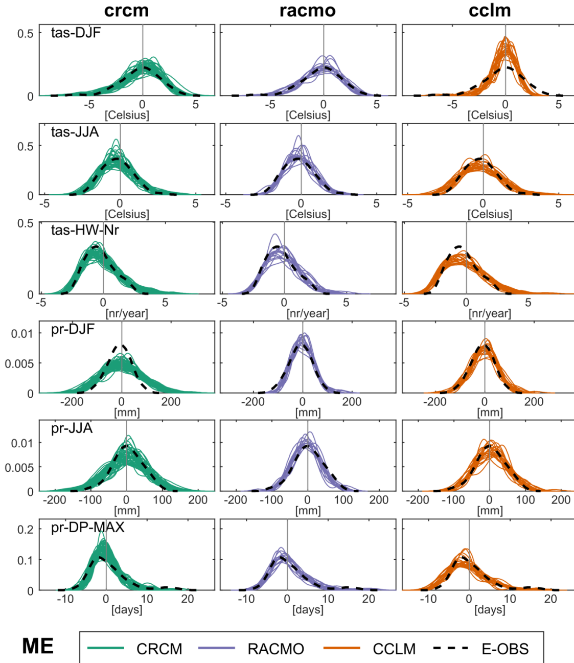
Figure 5: Probability density functions of the annual anomalies during the period 1957-2015 in E-OBS and each ensemble member for all 6 indicators in Mid-Europe (ME)
