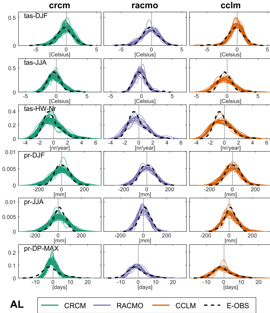
500 Figure 6: Probability density functions of the annual anomalies for all 6 indicators in the Alps (AL). For details see Figure 5
