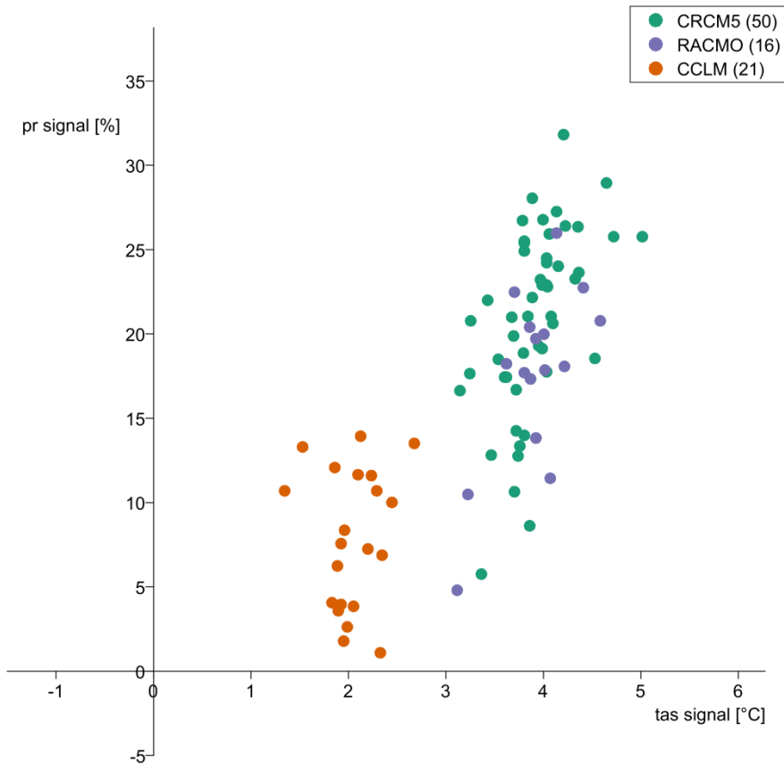
485 Figure 3: Change in winter temperature and precipitation for every member of the three ensembles in Mid-Europe (2070-2099 against 1980-2009). Changes are relative to each members' value in 1980-2009 for precipitation, while temperature changes are absolute
