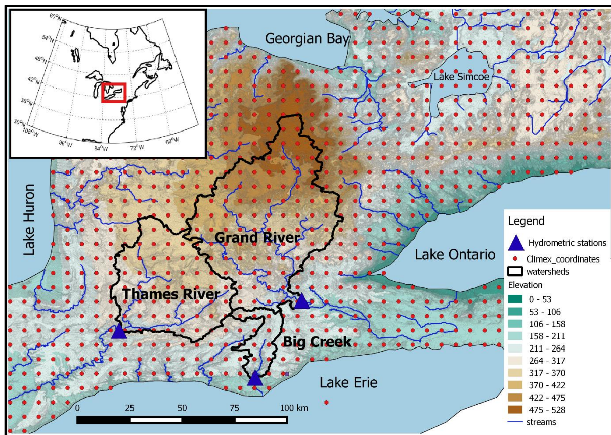
668 669 Figure 1: Location of the three watersheds and the ClimEx grid points used in this study and situation in the north- 670 eastern North American domain (Inset). Elevation source: High Resolution Digital Elevation Model (HRDEM, Natural 671 Resources Canada).
