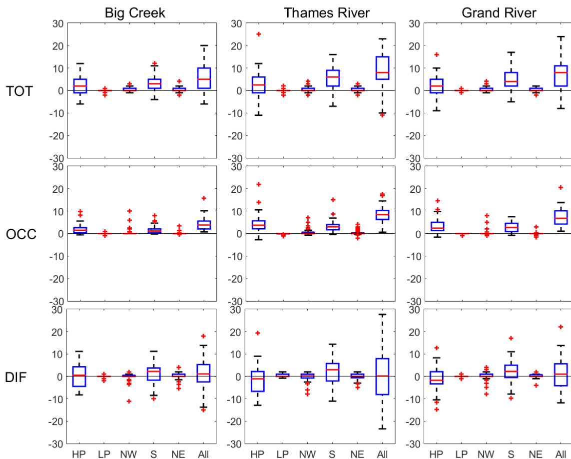
Figure 9: upper panels: Distribution of change in number of high flows between 1961-1990 and 2026-2055 simulated from the 50 members of the ensemble (TOT). Mid panels: Distribution of theoretical change in number of high flows using the factor of change in number of heavy rain and warm events between 1961-1990 and 2026-2055 (OCC). Lower panels: TOT minus OCC (DIF). Boxes extend from the 25th to the 75th percentile, with a horizontal red bar showing the median value. The whiskers are lines extending from each end of the box to the 1.5 interquartile range. Plus signs correspond to outliers.
