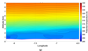
(g) Figure 7 a. Vertical cross sections of potential temperature at 31.1° N on 0700 UTC March 2, 2004 (6 km resolution WRF product). Red circle indicates region of sinking of air column (blocking of air). b. Vertical cross sections of u-wind speed at 31.1° N on 0700 UTC March 2, 2004 (6 km resolution WRF product). Red circle indicates region of blocking of air. c. Vertical cross sections of potential temperature at 31.1° N on 1100 UTC March 2, 2004 (6 km resolution WRF product). Red arrow indicates generation of Kelvin waves (cold air surge). d. Vertical cross sections of u-wind speed component at 31.1° N on 1100 UTC March 2, 2004 (6 km resolution WRF product). Red arrow indicates generation of Kelvin waves. e. Vertical cross sections of potential temperature at 31.1° N on 1500 UTC March 2, 2004 (6 km resolution WRF product). Red arrow indicates Kelvin wave (cold air surge) over time. f. Vertical cross sections of u-wind speed at 31.1° N on 1500 UTC March 2, 2004 (6 km resolution WRF product). Red arrow indicates Kelvin wave over time. g. Vertical cross sections of potential temperature at 28.85° N on 1500 UTC March 2, 2004 (6 km resolution WRF product).
