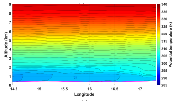
Figure 11 a. Vertical cross sections of potential temperature at 21.57° N on 0700 UTC December 8, 2011 (2 km resolution WRF product). Red circle indicates possible stability of the atmosphere. b. Vertical cross sections of u-wind speed at 21.57° N on 0700 UTC December 8, 2011 (2 km resolution WRF product). Red circle indicates blocking of the air. c. Vertical cross sections of potential temperature at 21.57° N on 1100 UTC December 8, 2011 (2 km resolution WRF product). Red arrow indicates Kelvin wave (cold air surge). d. Vertical cross sections of u-wind speed at 21.57° N on 1100 UTC December 8, 2011 (2 km resolution WRF product). Red arrow indicates Kelvin wave. e. Vertical cross sections of potential temperature at 18.89° N on 1500 UTC December 8, 2011 (2 km resolution WRF product).
