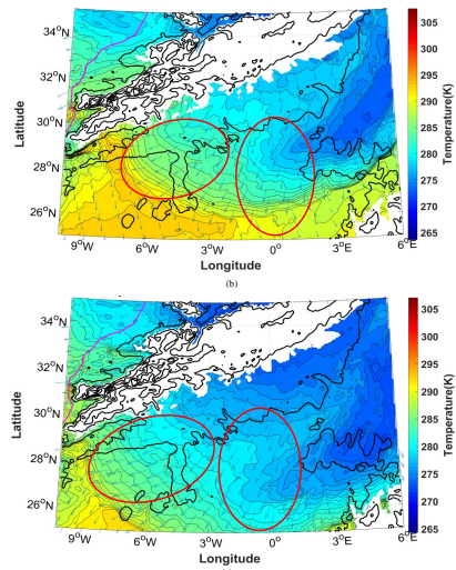
Figure 6 a. Temperature and wind speed/direction at 925 hPa on 1800 UTC March 2, 2004 (54 km resolution MERRA product) (Pukharel, 2016). Blue arrow lines indicate the wind flow. b. Temperature and wind speed/direction at 925 hPa on 1800 UTC March 2, 2004 (6 km resolution WRF product). Blue arrow lines indicate wind flow. The red circled areas represent the turning of the one wind component to the right in response to the Coriolis force and another component was turning to the left away from the mountains farther north and east as it goes south-southwestwards. c. Temperature and wind speed/direction at 925 hPa on 2200 UTC March 2, 2004 (6 km resolution WRF product). Blue arrow lines indicate wind flow. The red circled areas represent the turning of the one wind component to the right in response to the Coriolis force and another component was turning to the left away from the mountains farther north and east as it goes south-southwestwards.
