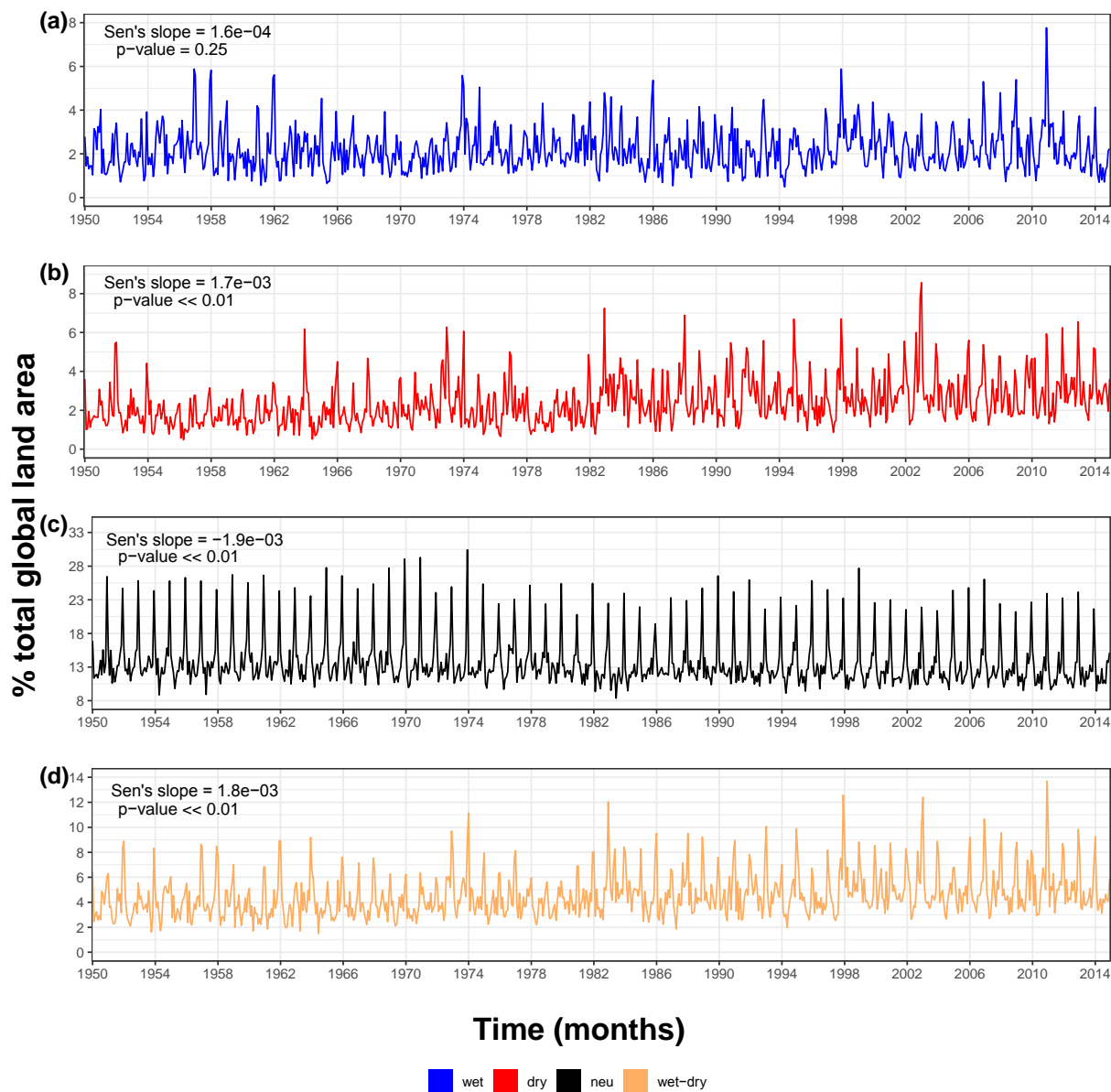
Figure 1. Percentage (%) of total land area with (a) wet (blue) and (b) dry (red) extremes along (c) neutral (black) and (d) extreme wet + extreme dry (orange) events over the 1950-2014 period. Wet extremes are sc\_PDSI\_pm \geq 3 and dry extremes sc\_PDSI\_pm \leq -3 monthly observations. Sen's slopes and the significance of the Mann Kendall test ( p -values) are shown in each panel.
