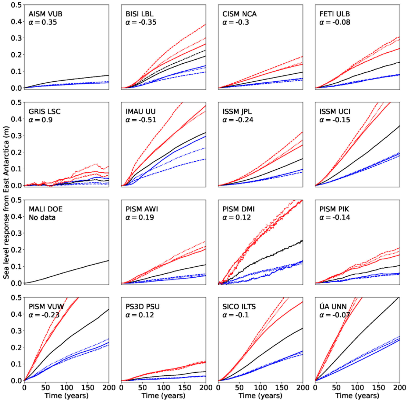
Figure 4a: Linearity check for East Antarctica Response of ice sheet models to additional basal melting of 8 m/yr (solid black line) underneath all ice shelves in East Antarctica compared to 4 m/yr (solid blue line) and 16 m/yr (solid red line). In order to check the linearity of the response to the warming amplitude the dashed red line gives the times series of the response to 8 m/yr of basal melt multiplied by 2 and the dashed blue line the same but divided by 2. The dotted lines give the scaled response with the scaling exponent \alpha (see equations (5) and (6)). A positive scaling exponent means that the ice sheet model responds super-linearly to basal ice shelf melting in this region. A negative \alpha indicates a sub-linear response in this region. AISM--VUB did not provide a 16 m/yr simulation. The black dashed line for BISI-LBL represents the simulation with 500m horizontal resolution that is used for the projections. The linearity is tested with a set of simulations at 1km horizontal resolution.
