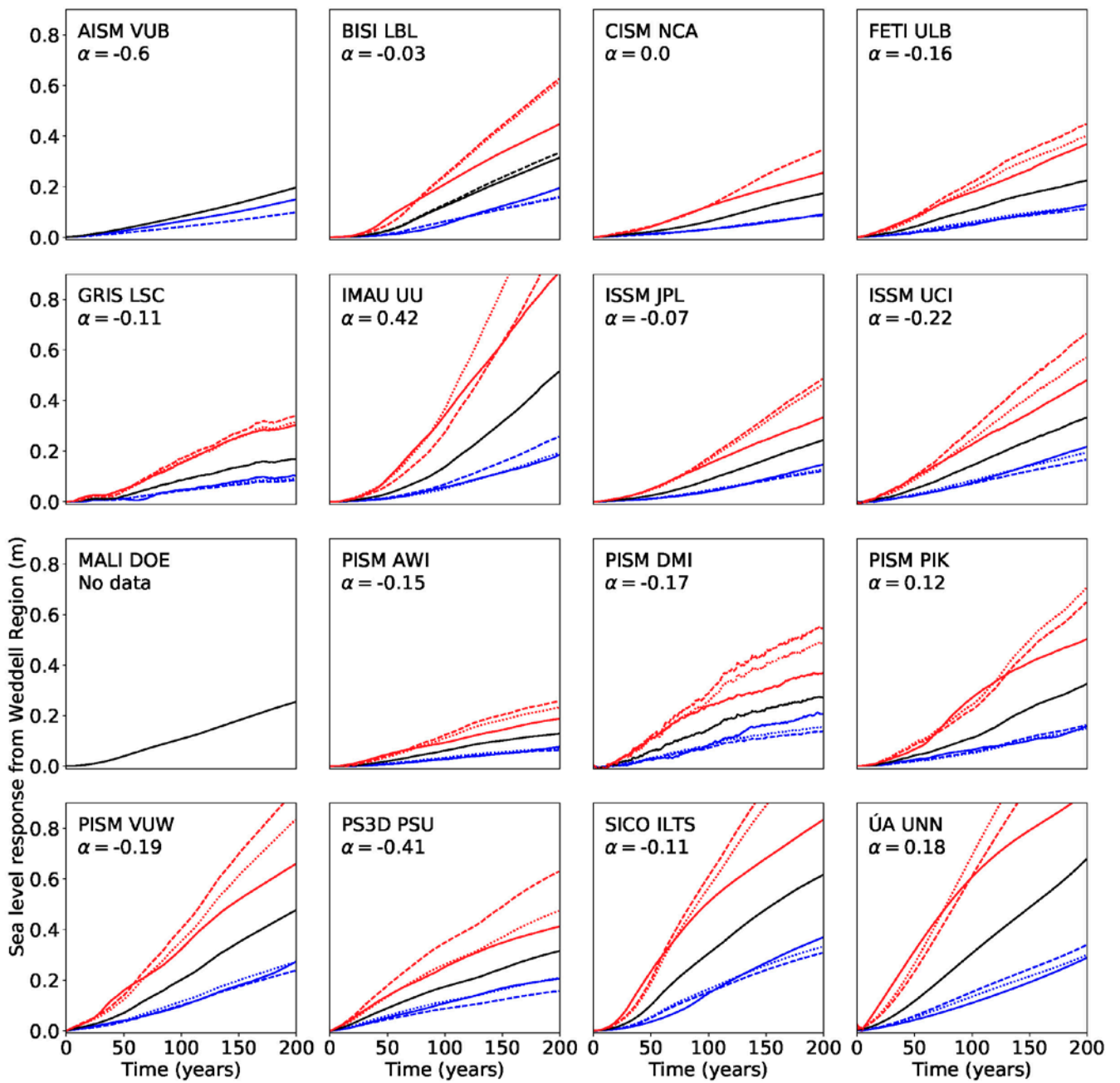
Figure 4d: Linearity check for the Weddell region as in Figure 4a.
