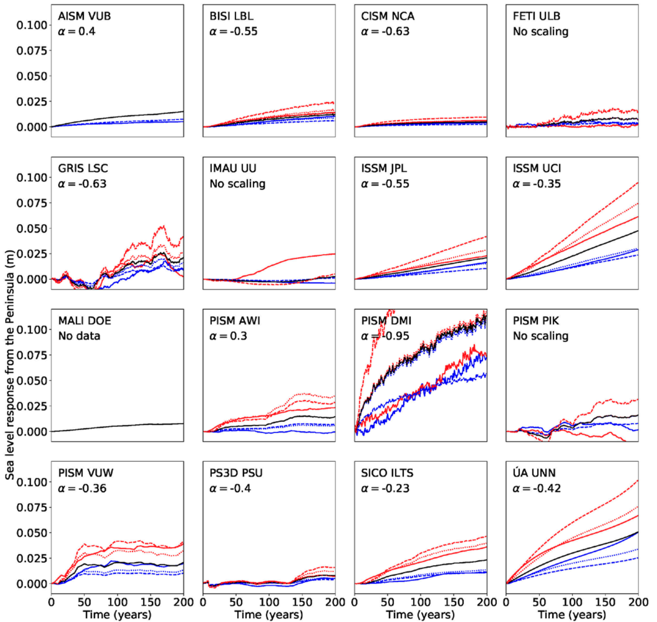
Figure 4e: Linearity check for the Antarctic Peninsula as in Figure 4a.
