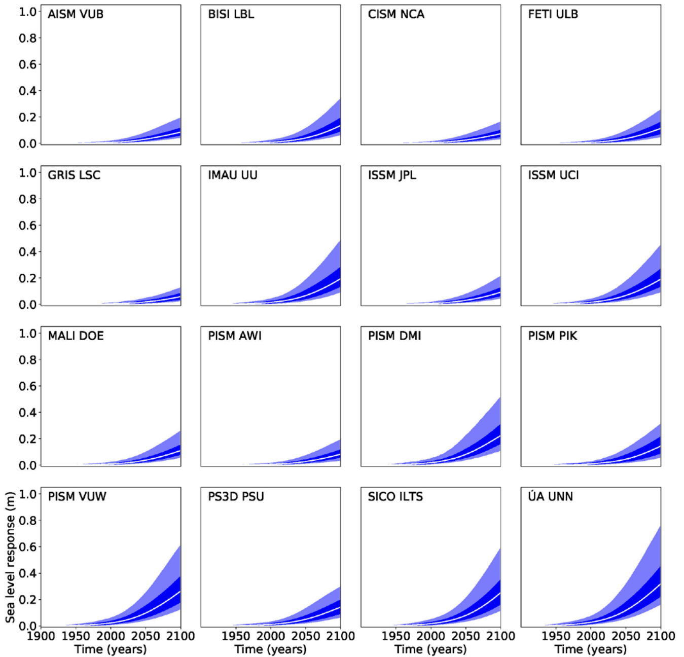
Figure 8: Projection of Antarctica’s sea level contribution under the RCP-2.6 carbon concentration scenario following the procedure depicted in Figure 1 and detailed in Section 2. The white line represents the median value, the dark shading the likely range (66-percentile around the median) and the light shading the very likely range (90-percentile around median). Compare Tables 7-10 for the values and their comparison to the other scenarios.
