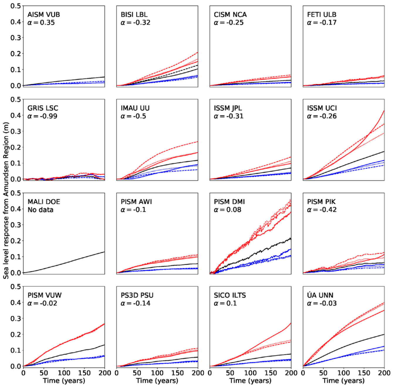
Figure 4c: Linearity check for the Amundsen region as in Figure 4a.
