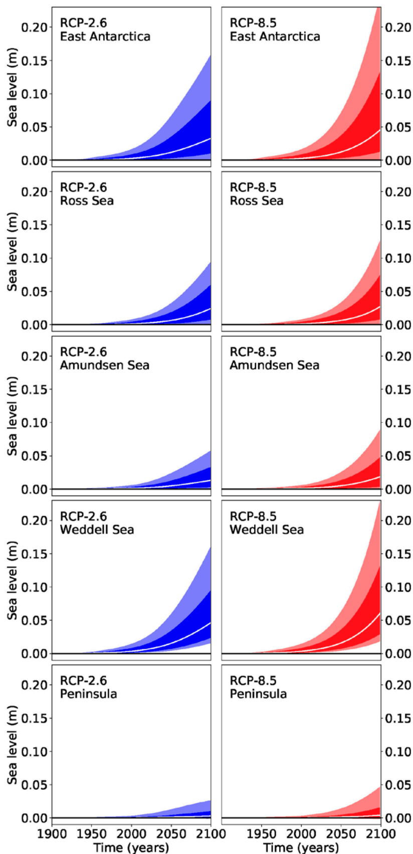
Figure 11: Projections from all models of the future sea level contribution of the different Antarctic sectors following the procedure depicted in Figure 1 and detailed in Section 2. The white line represents the median value, the dark shading the likely range (66-percentile around the median) and the light shading the very likely range (90-percentile around median).
