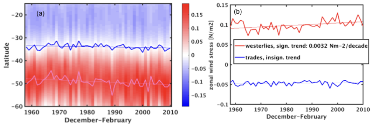
Figure 2. Temporal evolution of zonal mean ( 40^{\circ} W- 100^{\circ} E) zonal wind stress [ \text{N}/\text{m}^2 ] (shaded color) and the meridional position of maximum of westerlies (light pink curve) and of wind stress curl (blue curve). The linear trends in their positions are also displayed. There is a significant trend of -0.52^{\circ}/\text{decade} in the position of the westerlies and an insignificant trend for the trades (a) and the temporal evolution of the intensity of wind stress of westerlies (mean between 60^{\circ} S and of the latitude where wind stress turns eastward) and trades (mean between latitude where wind stress turns eastward and 15^{\circ} S) and their corresponding linear trends (b), both in December–February derived exemplary from the COREv2 data set in the period 1958–2009.
