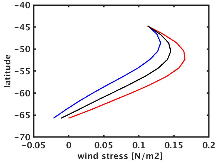
Figure 4. Impact of the meridional surface temperature gradient between 30^{\circ} S - 80^{\circ} S on the Southern Hemisphere wind stress intensity and position. Black curve shows the climatological mean of the zonal wind stress at the latitudinal range 45^{\circ} S - 65^{\circ} S in December–February (seasonal mean over the period 01/1948-08/2012) with NCEP1. The blue and red curves show the mean wind stress profile in years with a steeper temperature gradient (more than one standard deviation) (red line) or in years with a flatter temperature gradient (more than one standard deviation) (blue line). The meridional temperature gradient was estimated as the slope of a linear fit of the zonal mean temperature against latitude.
