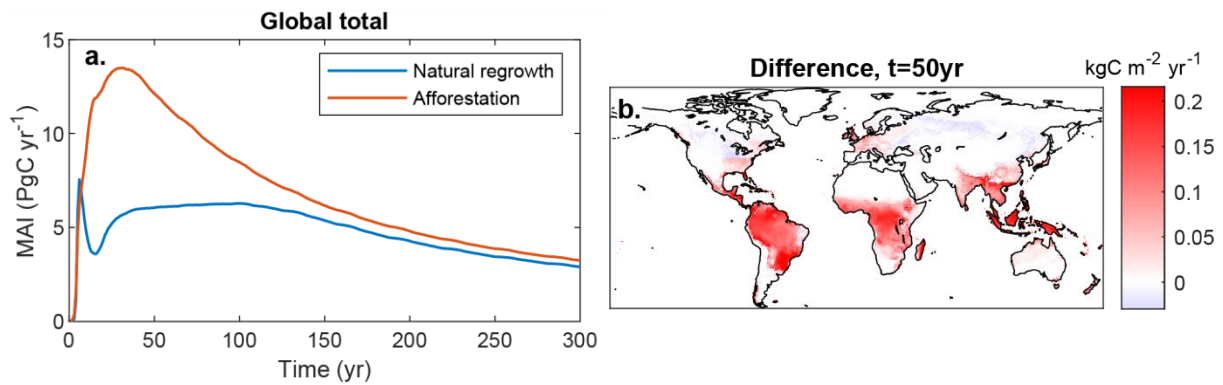
Figure 8. Mean ecosystem sequestration rate (Mean annual increment, MAI), determined as total C storage divided by time since start for LPJmL simulations with only forest plantations or only natural vegetation. (a) global total versus time; (b) difference between (afforestation minus natural regrowth) after 50 years.
