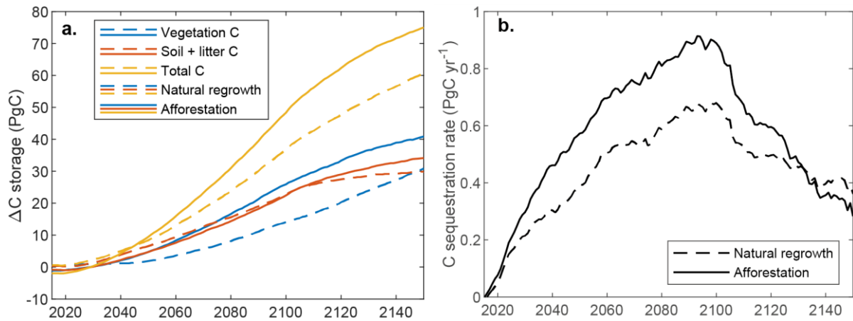
Figure 9 Results of the simulations for gradual afforestation and natural regrowth. Both graphs show differences relative to the baseline simulation with constant land-use. (a) global C storage; (b) global C sequestration rate, smoothed using a 10-year moving average window.
