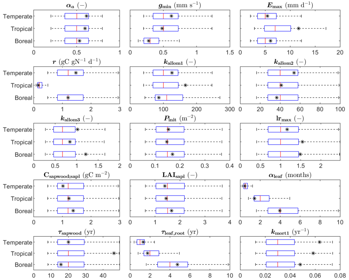
Figure 3. Prior distributions and estimated final values of the FPFT parameters estimated in the calibration. The boxplots indicate the 5% and 95% percentiles (whiskers) the median (red line) and 25% and 75% percentiles (box) or the priors. The final parameter estimate is indicated by the asterisk (*). See Table 1 Table 4 for explanation of the parameters.
