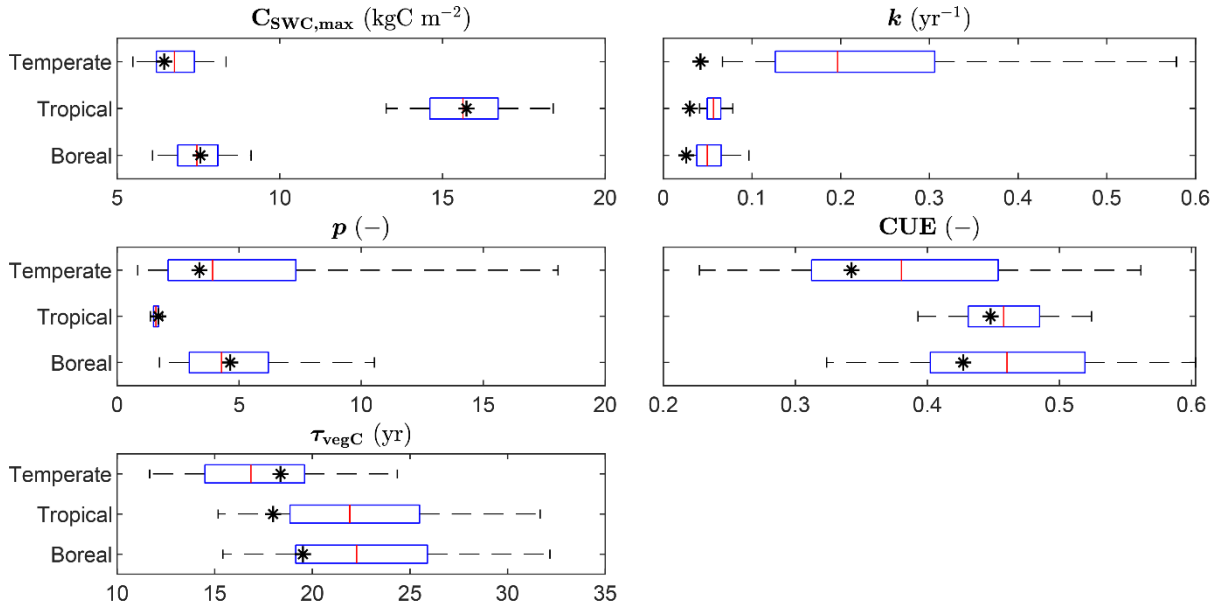
Figure 4. Ranges of the observations used in the calibration and LPJmL estimates after calibration. The boxplots indicate the 5% and 95% percentiles (whiskers) the median (red line) and 25% and 75% percentiles (box) of the likelihood function. The final fitted value is indicated by the asterisk (*). C_{SWC,max} : maximum stemwood C, k : growth rate; p : shape factor, CUE: carbon use efficiency (NPP to GPP ratio); \tau_{vegC} : vegetation C turnover time (vegetation C to NPP ratio).
