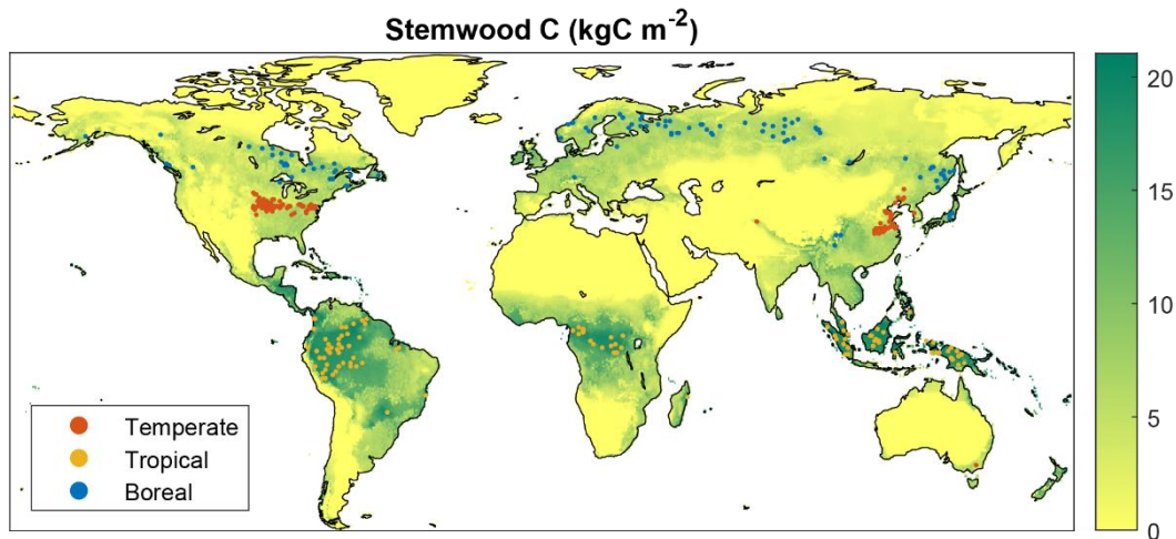
Figure 1. Location of the grid cells included in calibration simulations (100 per FPFT). The map shows simulated stemwood C (kgC m -2 ) for a simulation with potential natural vegetation.
