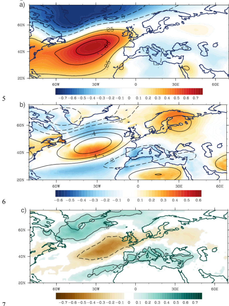
1 Figure 4. Correlation between principal component time series of the SNAO SLP in JA and a) sea level pressure 2 b) temperature at 2m (shaded) and geopotential height at 850hPa (contours), c) precipitation. All derived from 3 the CTRL run. Contours in a) and c) are shown for 0.25 and 0.5 correlations. Correlations are shown only when 4 significant at 1% level.
