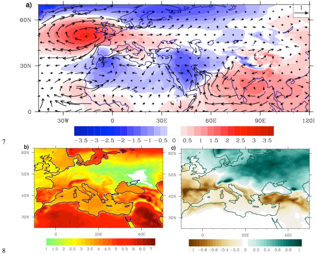
1 2 Figure 7. Projected future changes for the summer (JJA) a) sea level pressure (hPa, shaded) and u,v wind 3 components at 850hPa (m/s, vector), b) surface temperature (°C), c) total precipitation rate [mm/day], 4 over the period 2061-2099 compared with the baseline period 1961-1999. Changes are derived at the original horizontal 5 resolution. 6
