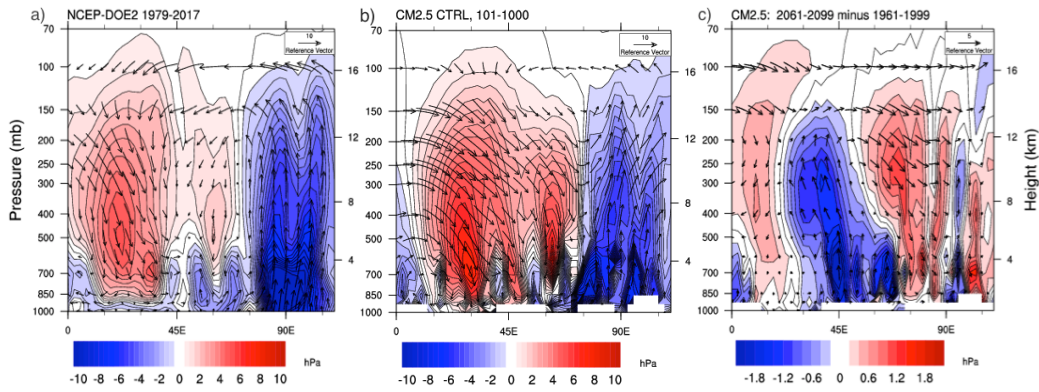
1 Figure 2. Height (pressure)-longitude cross-section of vertical velocity (Pa/s, shaded contours, downward motion 2 denoted with positive values) and vector of zonal wind (m/s) and vertical velocity (converted to m/s and scaled 3 with a factor of 1000) in July. Figure shows time-mean values in July a) derived for the period 1979-2017 in 4 NCEP-DOE2, b) derived from 101-1000 years of CTRL run in CM2.5; and c) projected future changes in the 5 period 2061-2099 in PROJ ensemble mean, compared with the baseline period 1961-1999 in the HIST ensemble 6 mean. All fields are shown on the 2.5°x2.5° horizontal grid and at the original vertical levels, common for CM2.5 7 and NCEP-DOE2.
