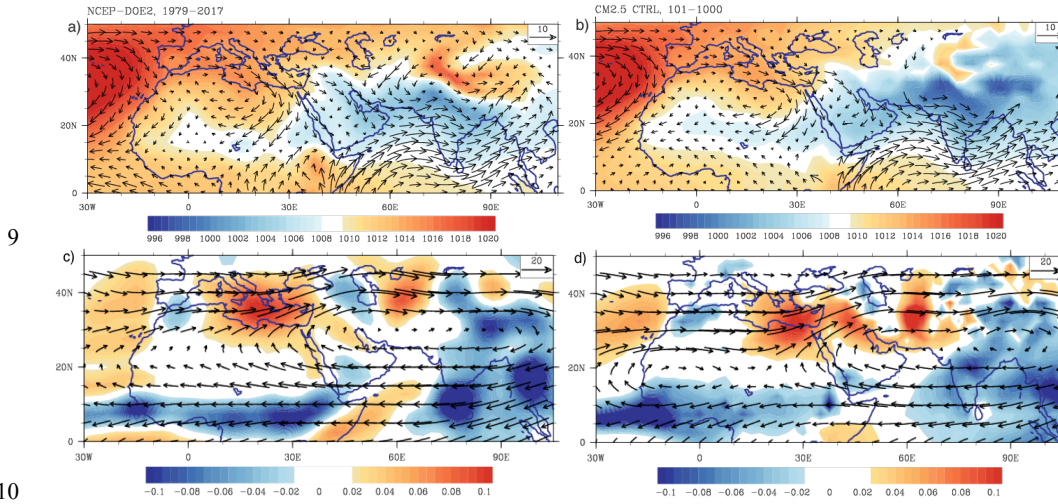
2 3 Figure 1. Seasonal (JJA) time-mean sea level pressure (hPa) and wind vector at 850hPa (m/s) in a) NCEP-DOE2, 4 b) CM2.5. Seasonal (July) time-mean vertical velocities at 500hPa (Pa/s, downward motion denoted with positive 5 values) and wind vectors at 200hPa (Pa/s, downward motion denoted with positive values), estimated for c) 6 NCEP-DOE2, and d) CM2.5 CTRL. Observational data is used for 1979-2017, control simulations data is used 7 for years 101-1000. All data sets are interpolated to the 2.5° horizontal grid. 8
