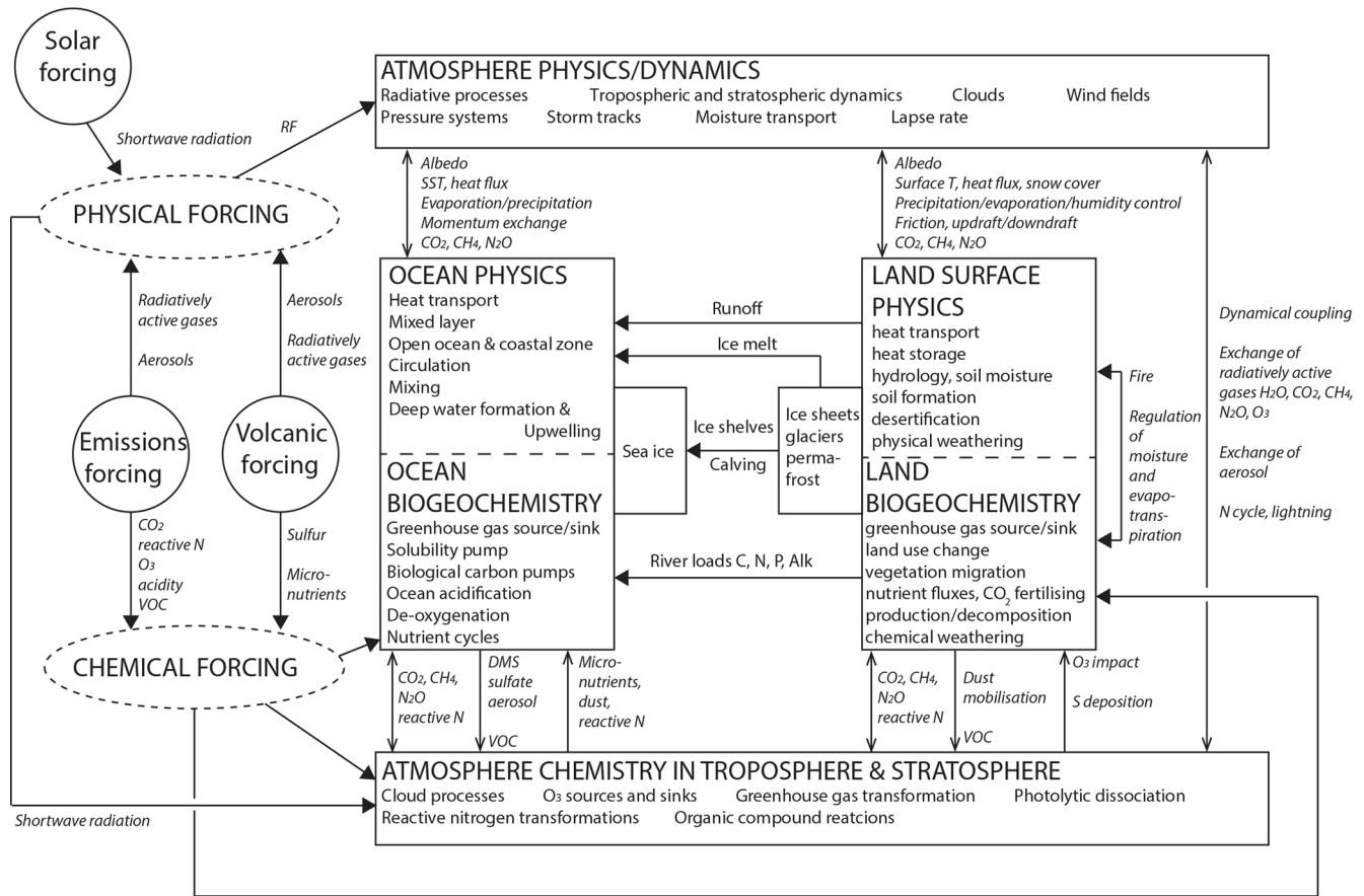
Figure 1. The Earth system as an extension of the physical climate system (inspired by Bretherton, 1985 TS3 ).
