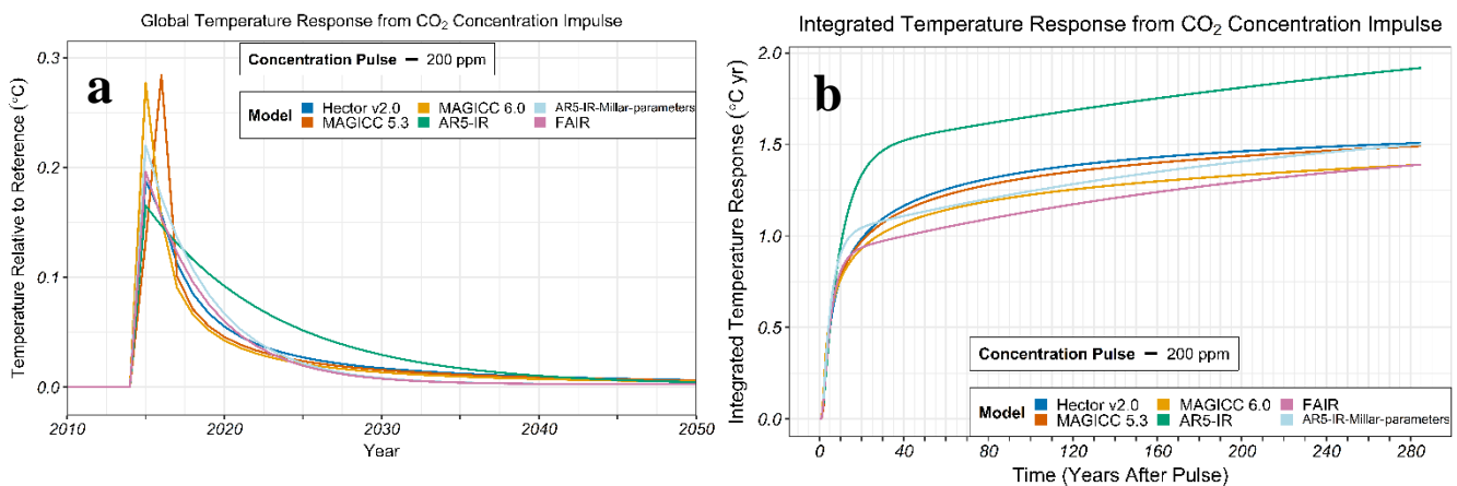
155 Figure R1 Global mean temperature response (a) and integrated global mean temperature response (b) from a CO 2 concentration perturbation in SCMs (MAGICC 6.0 – yellow, MAGICC 5.3 BC-OC – red, Hector v2.0 – blue, AR5-IR – green, FAIR – pink, AR5-IR-Millar-parameters –light blue). The time-integrated response, analogous to the Absolute Global Temperature Potential, is reported as 0-285 years after the perturbation.
