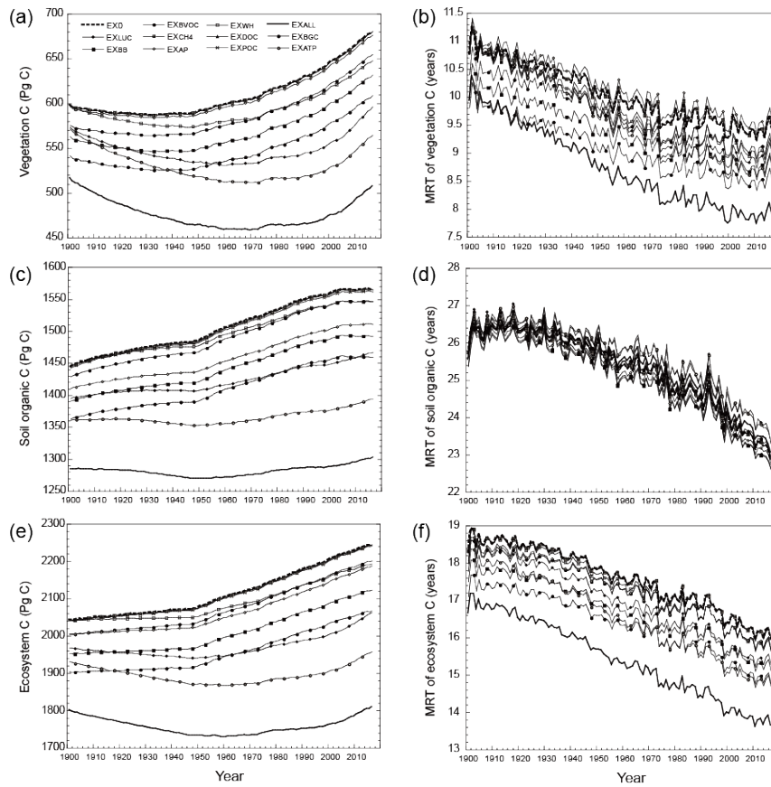
Figure 4. Time series of simulated carbon stocks and their mean residence time (MRT) in different experiments. (a) 5 Vegetation biomass and (b) its MRT, (c) soil organic carbon and (d) its MRT, and (e) total ecosystem carbon stock and (f) its MRT.
