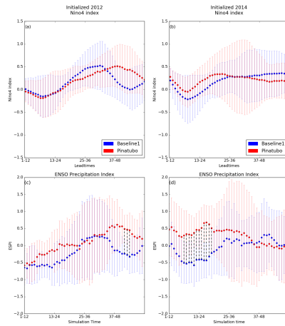
Figure 10: Top row shows the Niño4 index and bottom row shows the ENSO Precipitation Index (ESPI) for the first four prediction years calculated as a 12 month running mean to reduce variance. Left (right) column shows the 2012 (2014) initialized experiments. Error bars show the standard deviation of the ensemble and vertical black lines indicate a significant difference.
