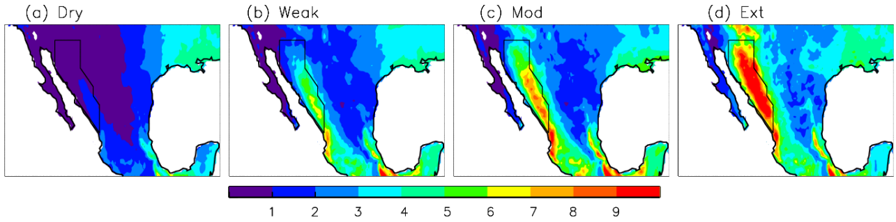
Figure 3. Mean daily rainfall (mm/day) (1981-2014) for the (a) dry days, (b) weak precipitation days, (c) moderate precipitation days, and (d) extreme precipitation days over the WNAM. Black boundary delineates the study region.
