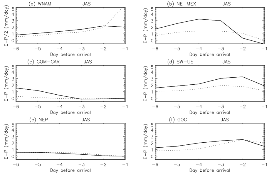
Figure 8. JAS time series of (E - P)_n (n=1 to 6) integrated over (a) WNAM, (b) NE-MEX, (c) GOM-CAR, (d) SW-US, (e) NEP and (f) GOC. Solid line: wet days. Dotted line: dry days. Note that the panel a is scaled by 0.5.
