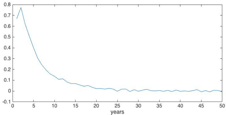
Fig. 2. Green's function for the global average surface air temperature.
