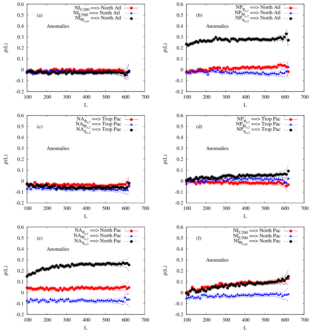
Figure B1. CCM as a function of the size L of the samples, as obtained from the anomaly of the monthly time series displayed in Fig. 1 for the reanalyses ERA-20C and ORA-20C. Each line with symbols corresponds to the influence of one variable on a specific coupled ocean-atmosphere basin. The specific variables are denoted in the caption corresponding to each line in each Panel.
