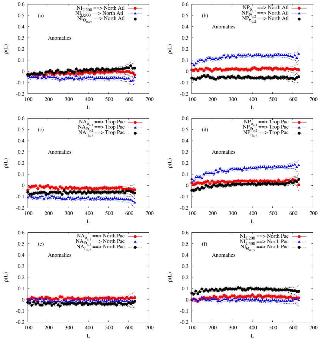
Figure B2. CCM as a function of the size L of the samples, as obtained from the anomaly of the monthly time series displayed in Fig. 2 for the reanalyses ERA-20C and ORAS4. Each line with symbols corresponds to the influence of one variable on a specific coupled ocean-atmosphere basin. The specific variables are denoted in the caption corresponding to each line in each Panel.
