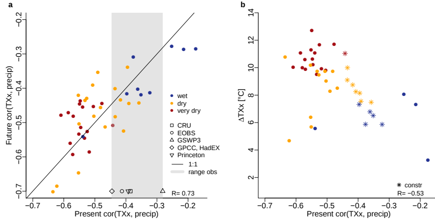
Figure 5. a) Future versus present-day cor(TXx, precip) for wet (blue), dry (orange), very dry very dry models (red) and for observations. The 1-to-1 line is shown in black. The gray background depicts the minimum and maximum from the distribution of cor(TXx, precip) of the observational datasets. b) Projected increase increase in TXx versus present-day cor(TXx, precip). The stars indicate the models within the constrained ensemble, the colors refer to the three model subgroups as in a).
