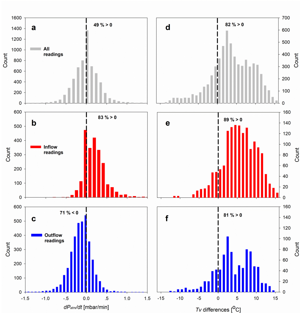
5 Figure. 6. Histograms of changes of atmospheric barometric pressure ( dP_{atm}/dt ) and T_v difference between the shaft and the atmosphere. The gray color (a, d) represents data from all 42 days of measurement. Red (b, e) and blue colors (c, f) represent data from the inflow and outflow events, respectively. Positive values of dP_{atm}/dt can drive inflow events from the atmosphere into the underground cavity, whereas negative values can drive outflow events. T_v differences (X-axis) are between 12 m-deep inside the shaft and the atmosphere.
