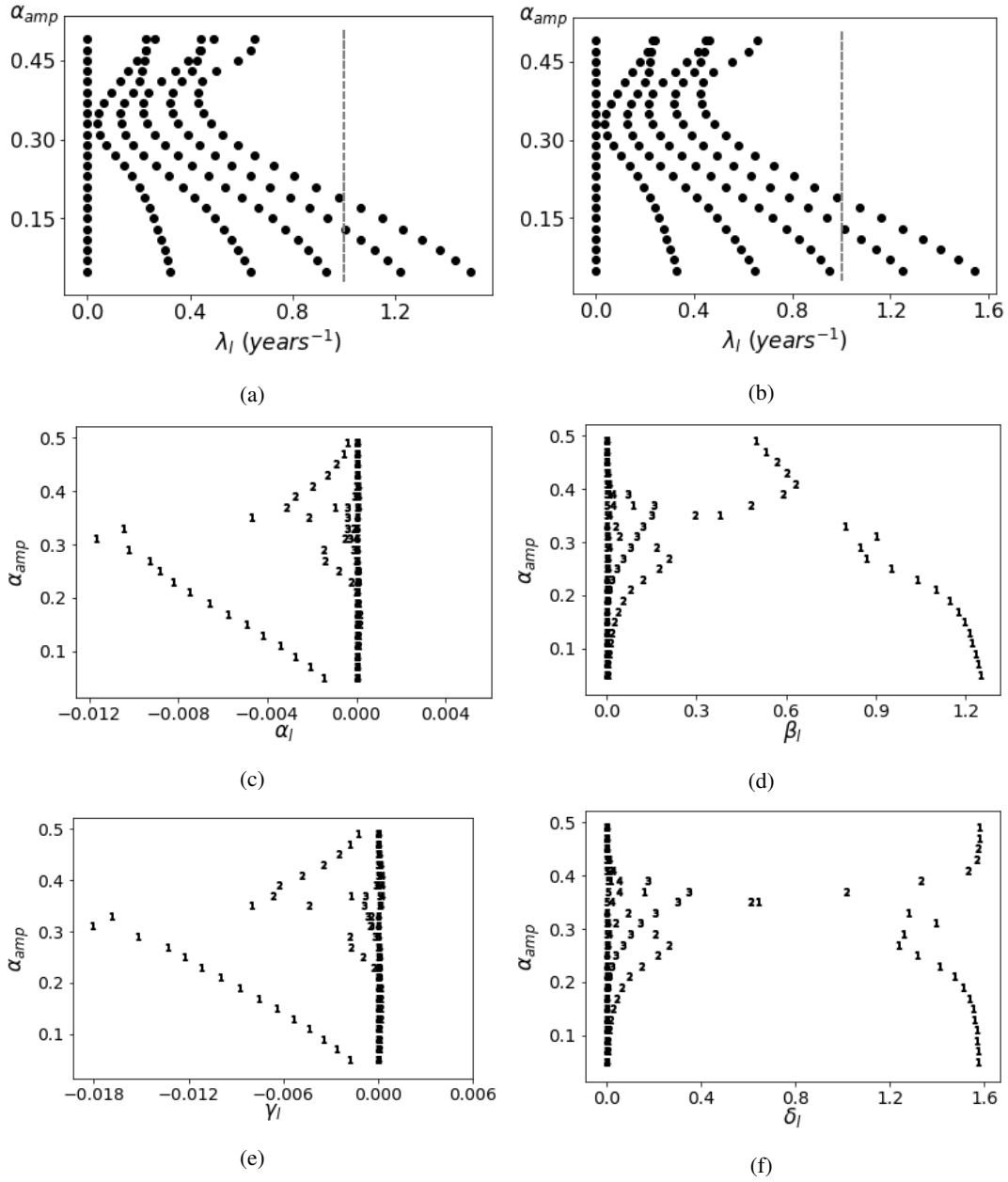
Figure 6. (a) Eigenvalues of the EBM depending on the amplitude of the albedo function for the simple EBM. The zero eigenvalues correspond to the invariant measure. (b) The extended EBM. (c) Albedo projection terms for solar forcing ( \alpha_l ) as defined in Equation 4.8 where the markers denote l (d) Same for temperature \beta_l (e,f) projections terms for GHG forcing \gamma_l and \delta_l respectively.
