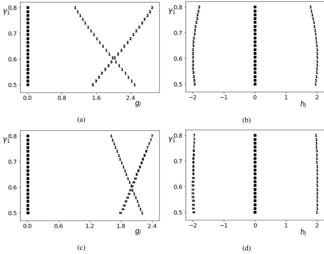
Figure 4. (a,b) Projections g_l (of predictor variable) and h_l (of predictand variable) for a weakly coupled two-dimensional OU system with \delta = 0.2 , (c,d) same for \delta = 0.5 .
