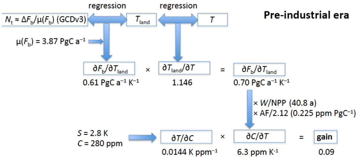
Figure 1: Schematic of the analysis of global fire-temperature relationships for the (a) satellite and (b) pre-industrial eras. F_b , biomass burning flux; T_{land} , global mean land temperature; T , global mean temperature. W , global land carbon storage; NPP, global net primary production; W/NPP = residence time of land carbon. AF, airborne fraction; 2.12 = conversion factor from ppm to \text{Pg C} . S , climate sensitivity; C , atmospheric \text{CO}_2 mole fraction. N_t , normalized anomalies of charcoal data; \Delta F_b , biomass burning flux anomalies; \mu(F_b) , mean biomass burning flux. See text for sources of temperature data.
