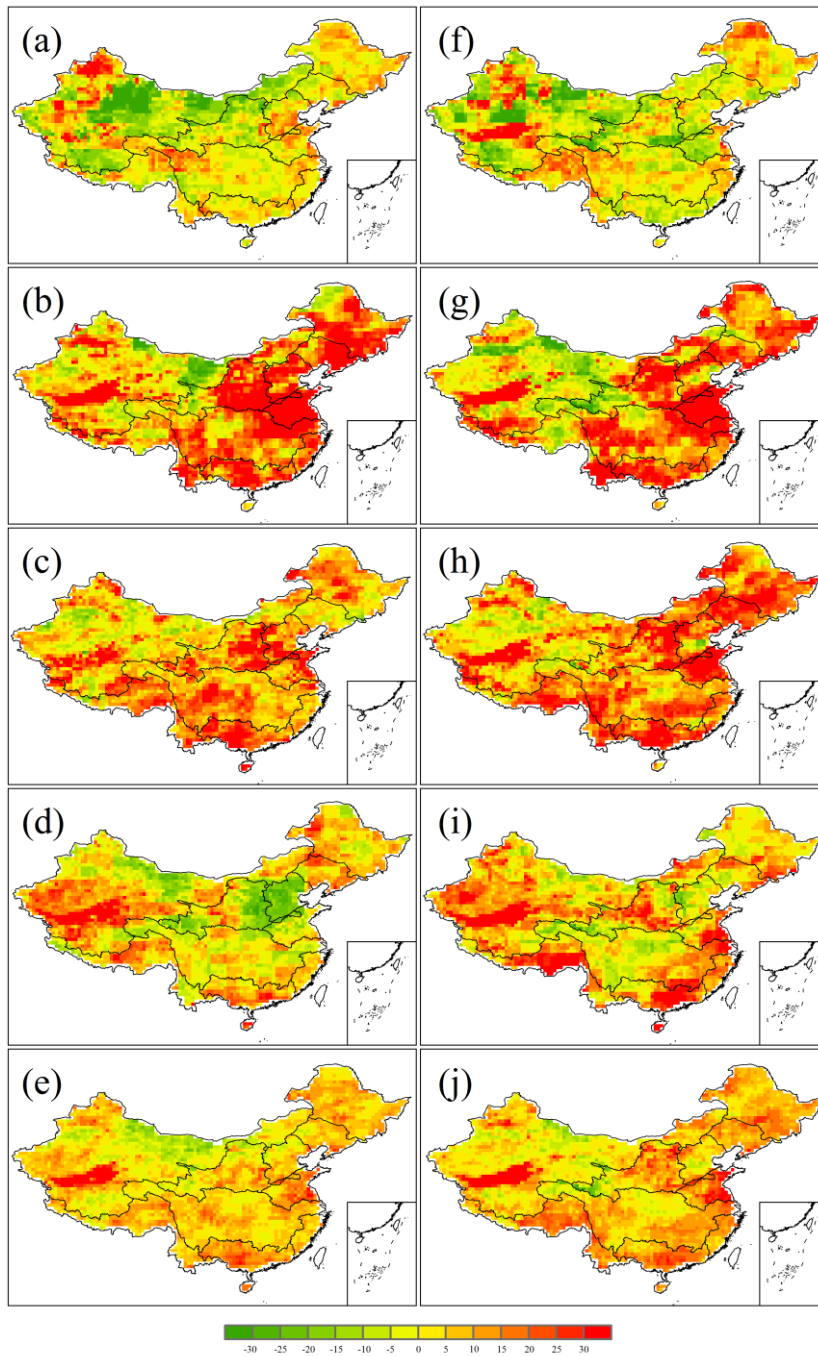
Figure 5: Median values of the changes in SD of runoff (%) in China under the 1.5°C (a, b, c, d, e) and 2.0°C (f, g, h, i, j) warming scenarios by the ECHAM6-3-LR (a, f), MIROC5 (b, g), NorESM1-HAPPI (c, h), CAM4-2degree (d, i), all the four GCMs (e, j), relative to 2006-2015.
