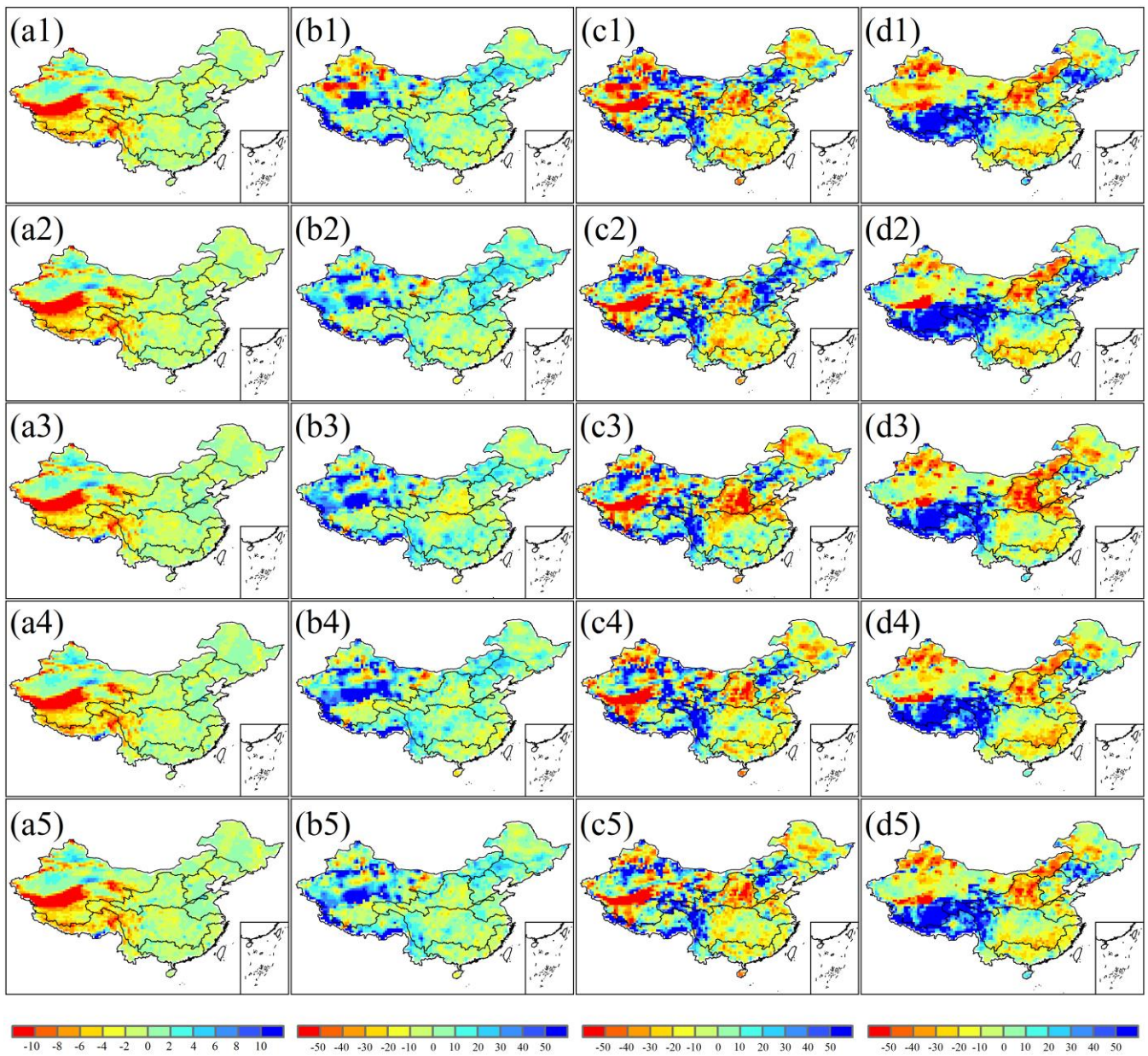
Figure 12: Differences between the HAPPI data and the observed data including annual mean temperature ( ^{\circ}\text{C} ) (a1-a5), annual precipitation (%) (b1-b5), as well as the differences between the projected annual runoff (%) (c1-c5) and annual TEWR (%) (d1-d5) by the HAPPI data and by the observed data, for 2006-2015, based on the ECHAM6-3-LR (a1, b1, c1, d1), MIROC5 (a2, b2, c2, d2), NorESM1-HAPPI (a3, b3, c3, d3), CAM4-2degree (a4, b4, c4, d4), and all the four GCMs (a5, b5, c5, d5), respectively.
