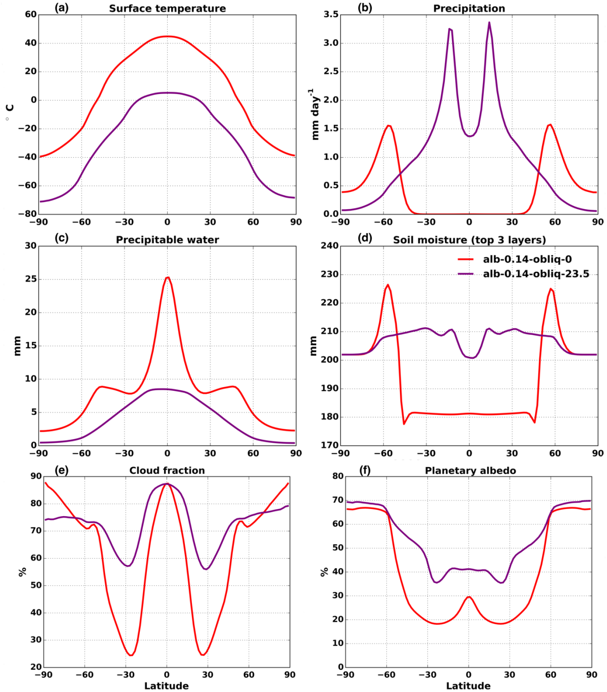
Figure 9: Annual mean meridional profiles as in Fig. 2. The red lines represent the HD state as in Fig. 2 (Z14 simulation in Table 1 with an obliquity of 0°). The purple lines correspond to the simulation with same initial conditions as in the HD state in Fig. 2 but with an obliquity of 23.5° (S14 simulation in Table 1).
