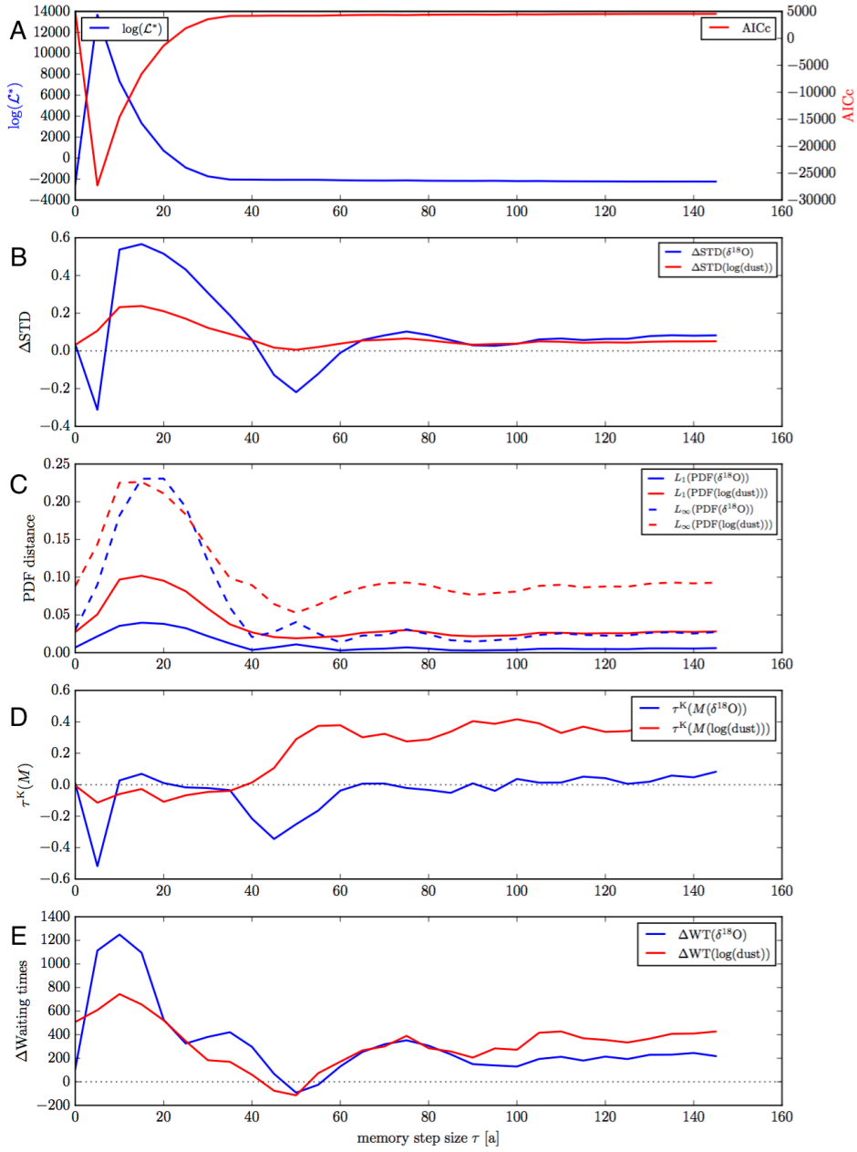
Figure 5. Summary statistics for different memory step sizes \tau . (A) Log-likelihood and AICc values for different memory step sizes \tau . The AICc is computed as AICc = 2pn/(n - p - 1) - 2\log \mathcal{L}^* . (B) Difference between observed and simulated standard deviations. (C) L^2 - and L^\infty -distances between observed and simulated PDFs. (D) Kendall's \tau -statistic between the third-order moments M(\theta) , computed for observed and simulated time series, respectively. (A-E) Difference between observations and simulations in terms of average waiting times between subsequent transitions from stadials to interstadials. In (B)–(E), statistics for simulated time series are obtained as averages over 1000 simulations using the full model.
