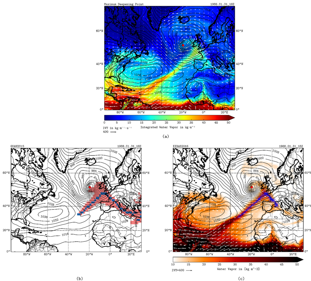
Figure 2. Example of a well-defined Atmospheric River associated to an explosive cyclone development land-falling the British Isles on 31 January 1988, 18 UTC. Mean Sea Level Pressure field (hPa) is indicated as black isolines in all panels. (a) total integrated column of water vapor (IWV, colours, kg·m -2 ) and integrated vapour transport (IVT, arrows, kg·m -1 ·s -1 ). (b) Shape region (red) and central axis of the Atmospheric river (blue) for the GUAN2015 algorithm. (c) as a) but showing only IWV values above 10 kg·m -2 and the blue crosses highlights the central axis of the Atmospheric River detected by the EIRAS2016 algorithm. In addition the location of the MDP is highlight with a red dot.
