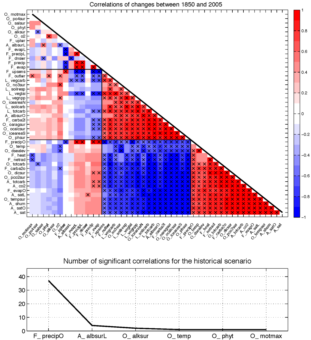
Figure 3. top: Correlation matrix for the historical scenario. The correlations are calculated between changes in the 46 model output variables for temporal differences between 1850-1860 and 1995-2005 from the results of the perturbed parameter simulations (as in Figure 1). Correlations significant on a 5% significance level are marked with 'x'. The order of the variables was determined based on their correlation strength to surface air temperature (A_sat) in the historical scenario. Prefixes A, O, L and F, stand for atmosphere, ocean, land and fluxes, respectively, for detail description of the model output variables see Table A1.
